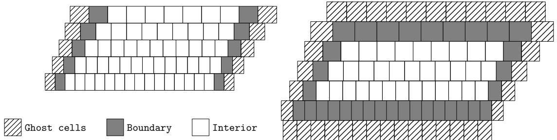
Figure 3.4: Ghost, boundary and interior cells for zonal (left) and meridional (right) advection for a rectangular subdomain.
