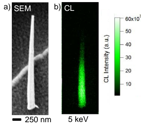
Figure 4.28 – a) SEM image of a ZnTe NW with a ZnMgTe shell deposited on a Si substrate. b) Low temperature cathodo-luminescence monochromatic image of the same NW taken at the maximum of the CL spectrum (at 2348.2 meV). The image was recorded at 5K and using an electron beam excitation of 5 KeV and a spot size aperture of 3.
