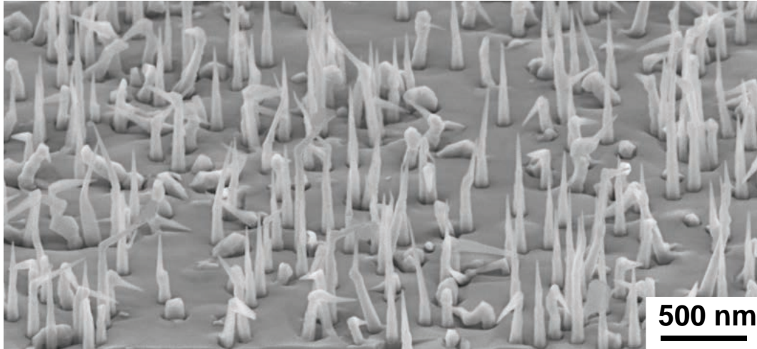
Figure 4.3 – SEM image of sample B : cone-shaped ZnTe NWs with a CdTe insertion. The growth conditions are written in the text.
