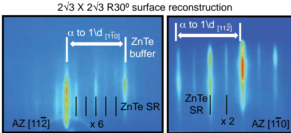
Figure 2.8 – RHEED diffraction pattern of the 2\sqrt{3} \times 2\sqrt{3} R30^\circ SR on the ZnTe(111)B surface along the [11-2] and [1-10] azimuths. The 2D diffraction of the ZnTe layer is indicated in white and the streaks corresponding to the SR in black.
