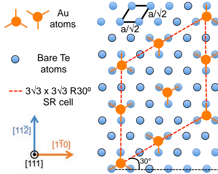
Figure 2.21 – A possible motif for the Au-induced 3\sqrt{3} \times 3\sqrt{3} R30° surface reconstruction cell is shown over the ZnTe(111)B surface. In black we indicate the ZnTe unit cell, in red the SR cell, in blue de Te atoms and finally, in orange the Au atoms.
