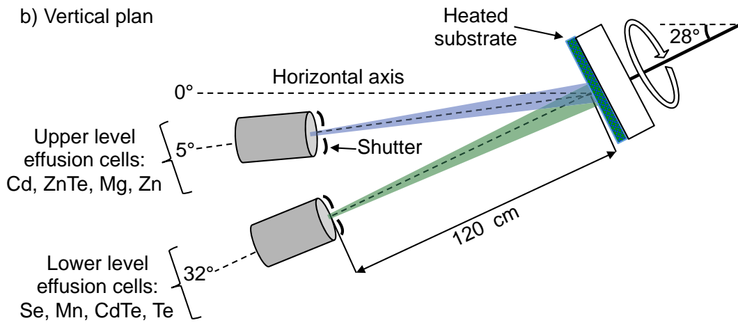
Figure 1.8 – Scheme of the II-VI MBE chamber used for in this work. The angles of the effusion cells with respect to the sample normal are indicated.
