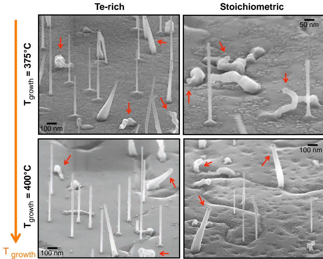
Figure 3.23 – SEM images of samples grown at T_{growth} = 375^{\circ}\text{C} and T_{growth} = 400^{\circ}\text{C} under both stoichiometric and Te rich conditions. Notice that the scale of the image of the sample grown at T_{growth} = 375^{\circ}\text{C} and stoichiometric conditions is twice bigger than the others.
