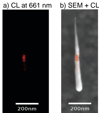
Figure 4.30 – a) Low temperature CL monochromatic image of an isolated ZnTe NW with a CdTe QD (sample B) deposited on a Si substrate. The image was taken at 1872 meV (661nm) corresponding to a CdTe emission. The image was recorded at 5K and using an electron beam excitation of 30 KeV. b) SEM image of the same NW with the CL image superposed.
