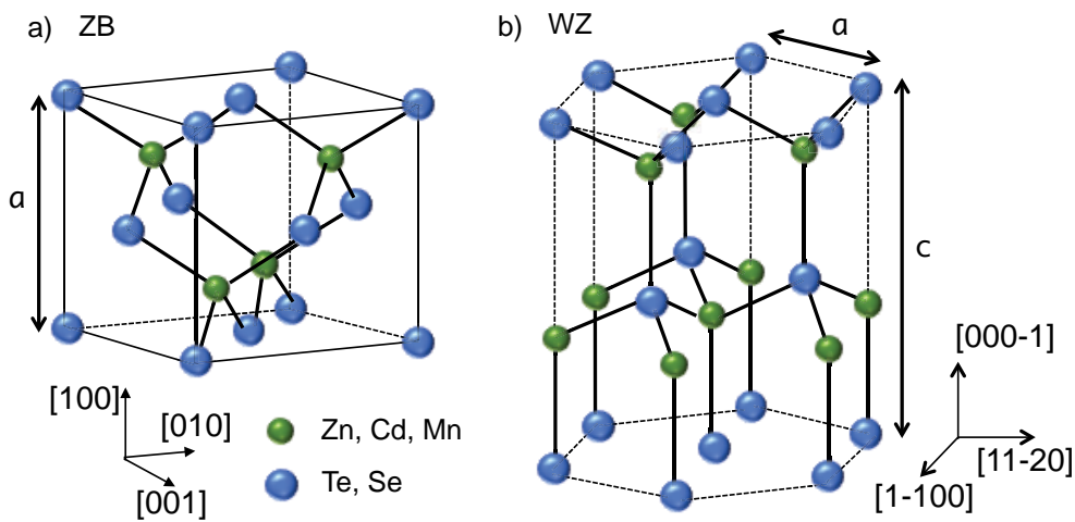
Figure 1.1 – Zinc-blende (ZB) and Wurtzite (WZ) crystal structure of II-VI semiconductors.
