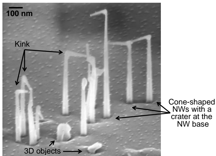
Figure 3.7 – SEM image of ZnTe NWs with a CdTe insertions grown under Te-rich flux conditions. Only cone-shaped NWs are observed on the sample (no cylinder-shaped NWs). We also observed objects crumbling on the surface, they are indicated as “3D objects”.
