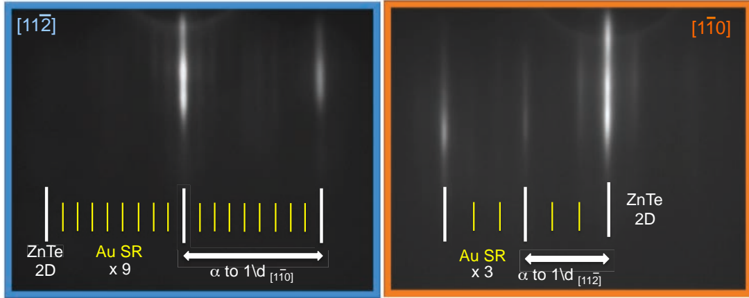
Figure 2.19 – 3\sqrt{3} \times 3\sqrt{3} R30° surface reconstruction (SR) observed by RHEED along [11\bar{2}] and [1\bar{1}0] azimuths. This SR is induced by Au over the ZnTe(111)B surface at temperatures above 300°C.
