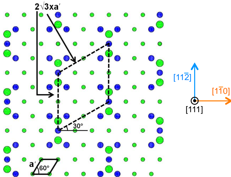
Figure 2.9 – The 2\sqrt{3} \times 2\sqrt{3} R30^\circ surface reconstruction (SR) is illustrated (based on the motif of the CdTe SR [33, 34]). The SR cell is indicated with the dash line in black and the ZnTe unit cell with a black continuous line ( a' = \frac{a}{\sqrt{2}} and a is the lattice parameter of ZnTe). Zn atoms are represented in blue and Te atoms in green. The big circles are the first Te layer and the small circles are the second Te layer.
