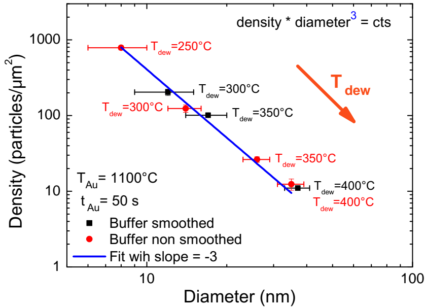
Figure 2.16 – Au-particles surface density (in logarithmic scale) as a function of the Au-particles average diameter for samples with different dewetting temperatures: T_{dew} = [250^{\circ}\text{C}–400^{\circ}\text{C}] . For all samples: t_{dew} = 5 min, T_{Au} = 1100^{\circ}\text{C} and t_{Au} = 50 s. In black: samples where the ZnTe buffer layer was smoothed at 420°C prior to the Au deposition at RT. In red: samples where the ZnTe buffer layer was not smoothed. The blue line is a fit of the data with a constant slope of -3. The data are obtained from SEM images of the surface.
