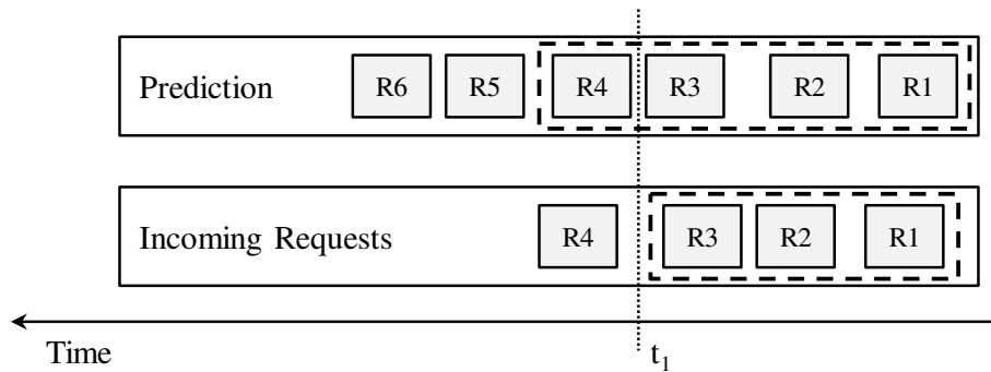
Figure 4.2: Scheduling with predicted future requests.
