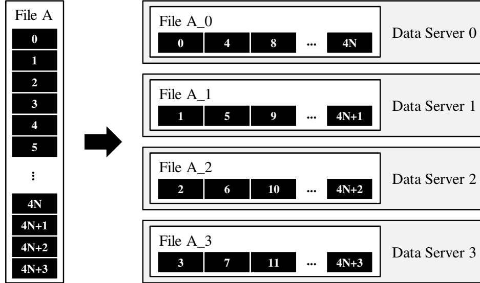
Figure 4.9: Striping of a file among four data servers.
