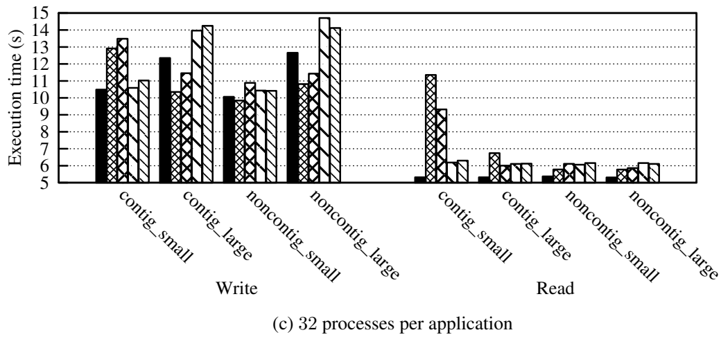
Figure A.1: Results obtained for the single application scenarios with the shared file approach in the Pastel cluster.
