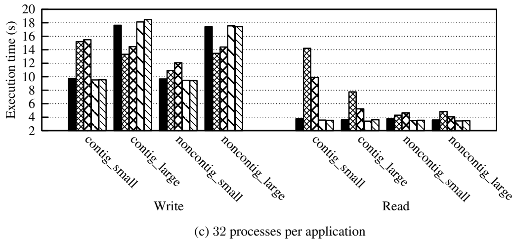
Figure A.9: Results obtained for the single application scenarios with the shared file approach in the Suno cluster.
