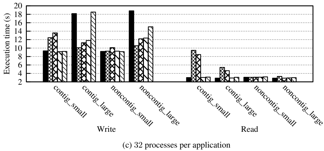
Figure A.5: Results obtained for the single application scenarios with the shared file approach in the Graphene cluster.
