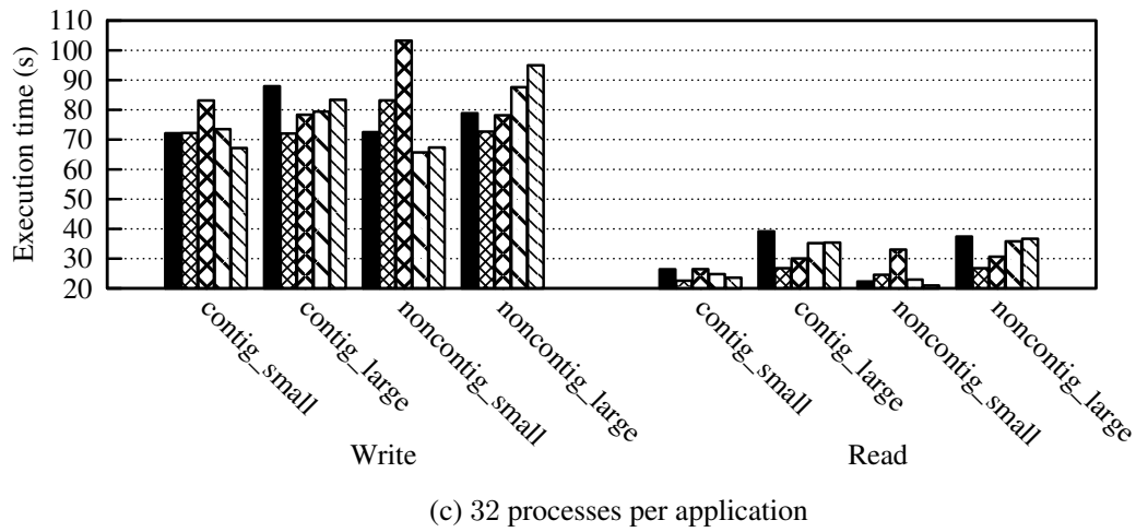
Figure A.15: Results obtained for the multi-application scenarios with the shared file approach in the Edel cluster.
