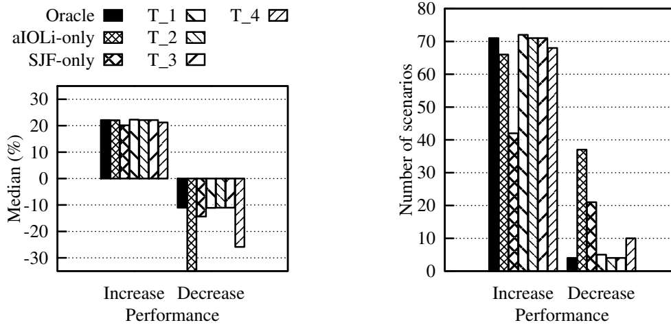
(a) Median performance differences (b) Situations with performance differences Figure 6.1: Performance results for the tested scheduling algorithm selection trees.
