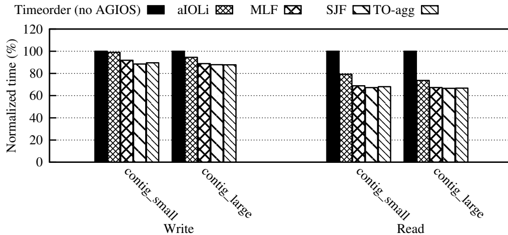
Figure 3.9: Results with four applications and the file per process approach in Suno with 32 processes.
