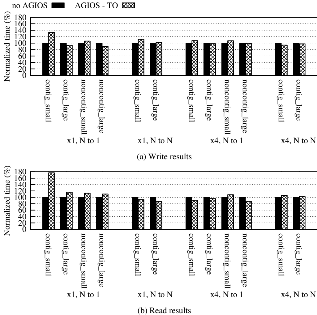
Figure 3.5: Results with TO over not using AGIOS in the Pastel cluster - tests with 16 processes.
