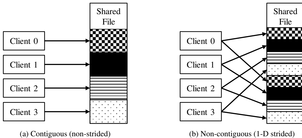
Figure 3.4: Spatial locality aspect with a shared file.
