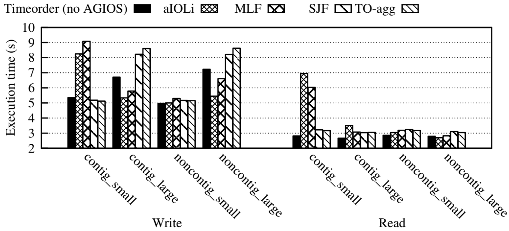
(a) 8 processes per application
