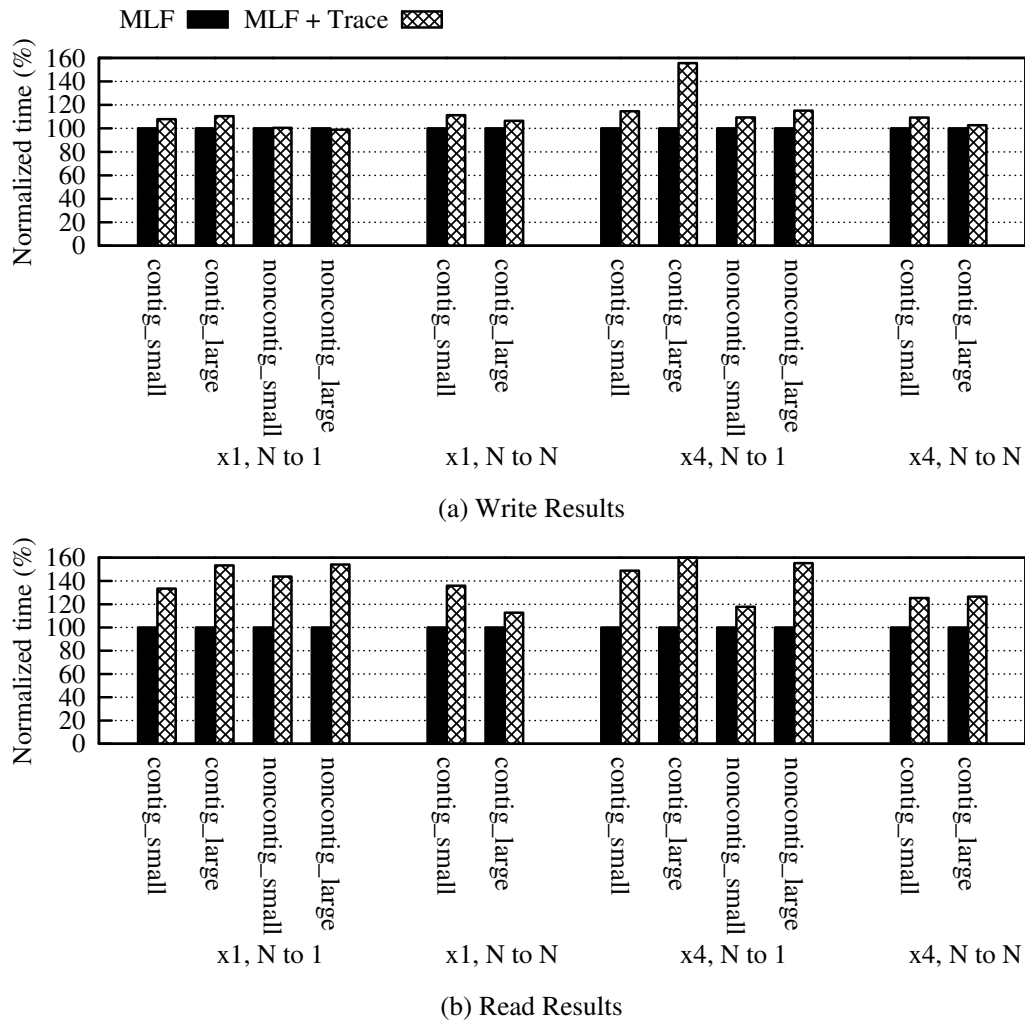
Figure 4.5: Overhead caused by trace generation on AGIOS (MLF scheduling algorithm) with 8 clients in the Pastel cluster.
