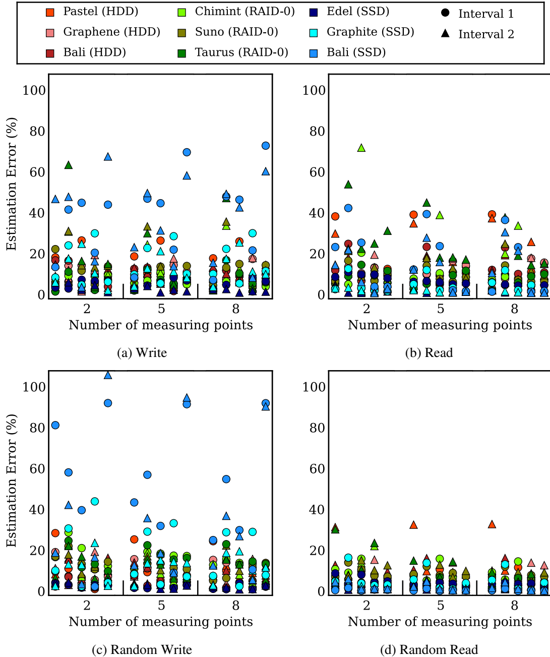
Figure 5.2: Absolute error induced by using linear regressions to estimate the access time curves.
