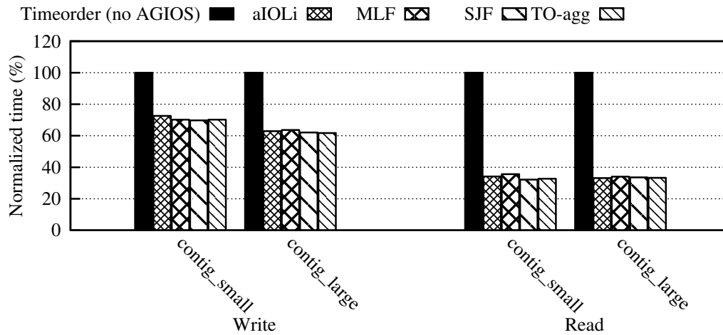
Figure 3.8: Results with a single application and the file per process approach in Pastel with 32 processes
