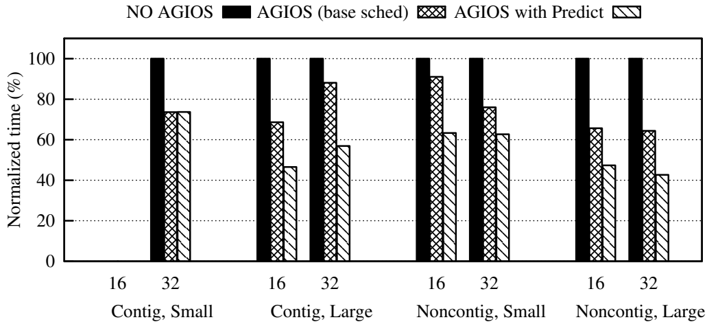
(a) Write Results
