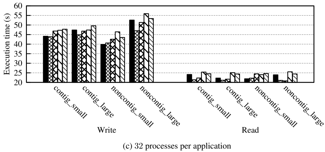
Figure A.3: Results obtained for the multi-application scenarios with the shared file approach in the Pastel cluster.
