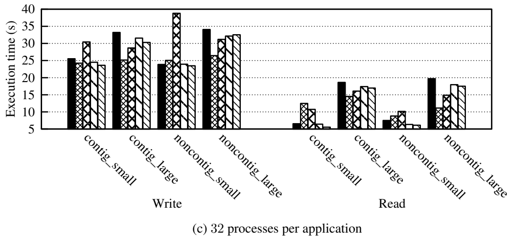
Figure A.13: Results obtained for the single application scenarios with the shared file approach in the Edel cluster.
