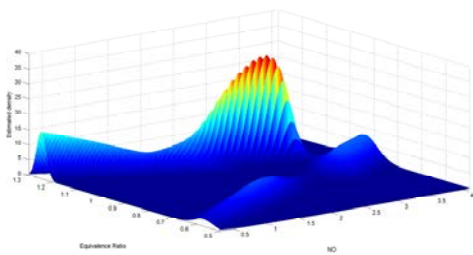
(c) 3D view of the resulting conditional density showing the 4 regression components.
