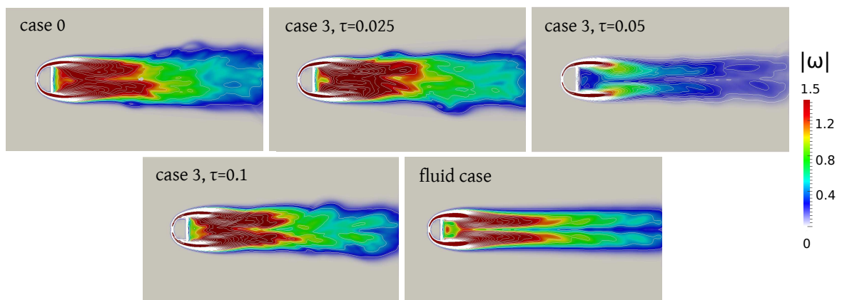
Figure 4.41: Effects of various layer thicknesses \tau for case 3 on mean vorticity magnitude for flow past a hemisphere at Re = 300 , with \lambda = 10 within the permeable region.
