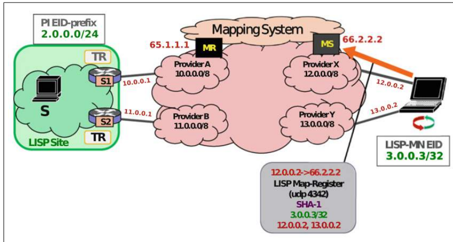
Figure 2.13: LISP Mobile Node registering procedure of an EID-to-RLOC binding
