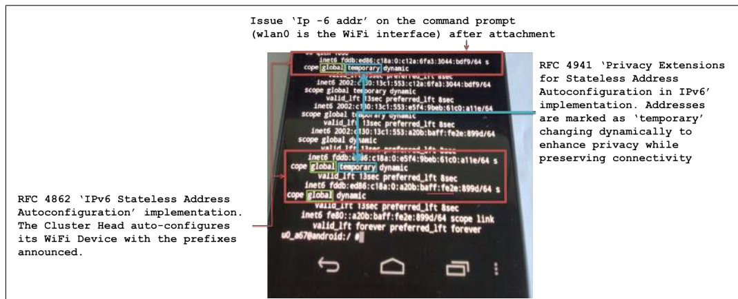
Figure 3.11: Android phone as connected to the MR.
