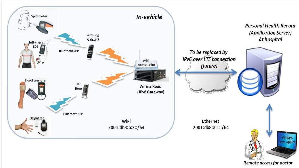
Figure 3.9: eHealth and Vehicular testbeds integration.
