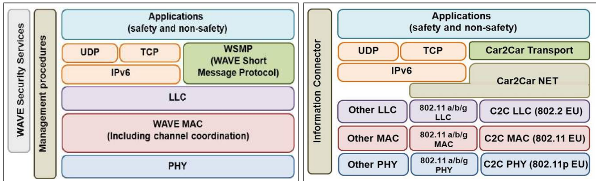
Figure 2.25: IPv6 networking support through different SDO protocol stacks
