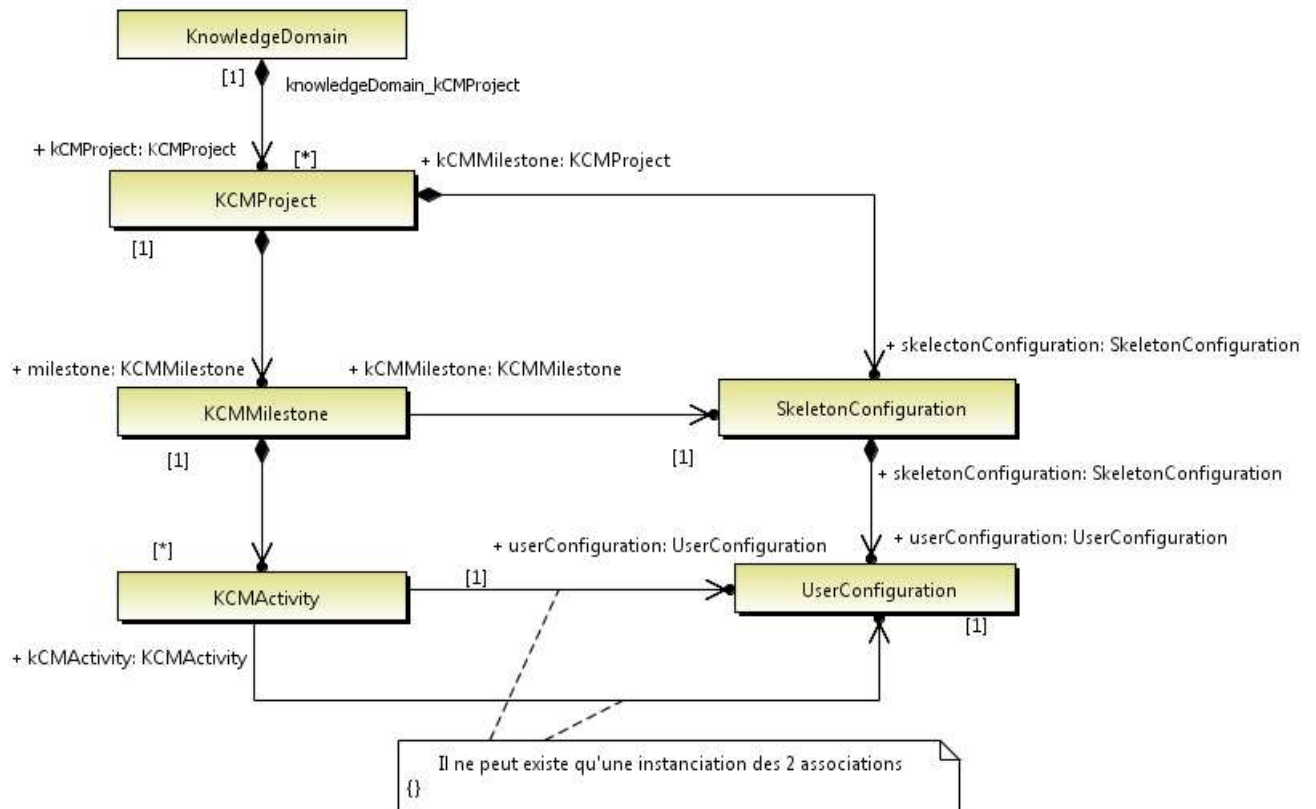
Figure 78 : package KCMProject
