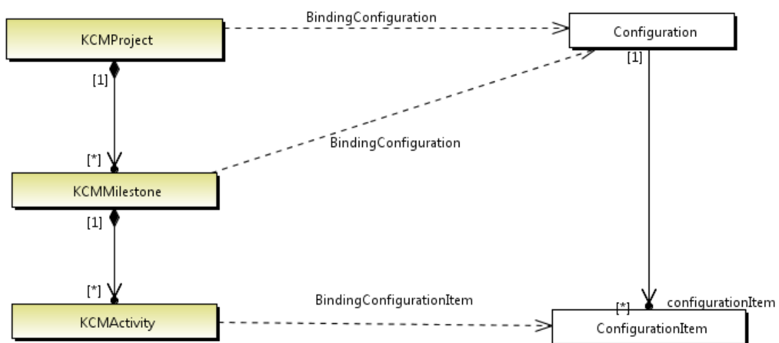
Figure 92 : diagramme ProjectBinding
