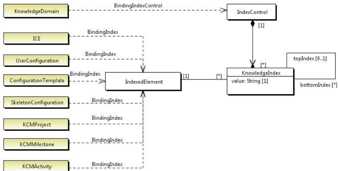
Figure 93 : diagramme KnowledgeIndexBinding
