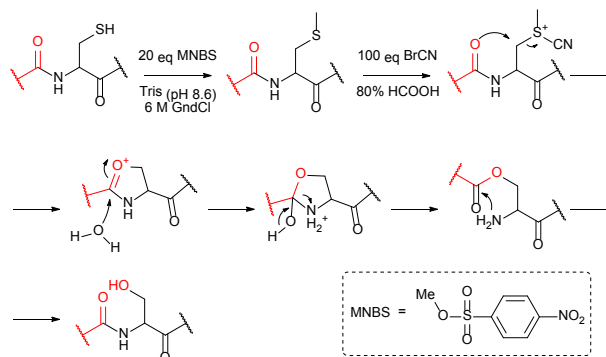
Fig. 71. Conversion of a Cys into a Ser residue by transforming the former into a corresponding methyl cysteine and following thereof by CNBr. 640 Methionine must be protected by transforming into corresponding sulfoxide form, because this is inactive for the CNBr reaction. 641
