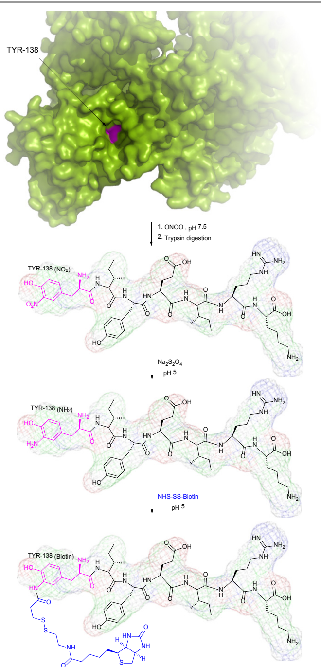
Fig. 49. Two-step biotinylation of HSA (pdb: 1A06) described by Nikov et al. 478 a ) Preferential nitration of TYR-138 (shown in magenta) and TYR-411 residues of HSA with peroxynitrite was achieved using protocol described by Jiao and colleagues. 475 b ) Aminotyrosine of the peptide 138 YIYEIARK 144 , obtained after the step of reduction with sodium dithionite and following digestion of nitrated HSA with trypsin, were selectively modified with a cleavable biotin-containing reactant at pH 5.0.
