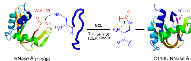
Fig. 85. Selenocysteine native chemical ligation applied for the preparation of C110U mutant of RNase A (wild-type - pdb: 7RSA). 719
