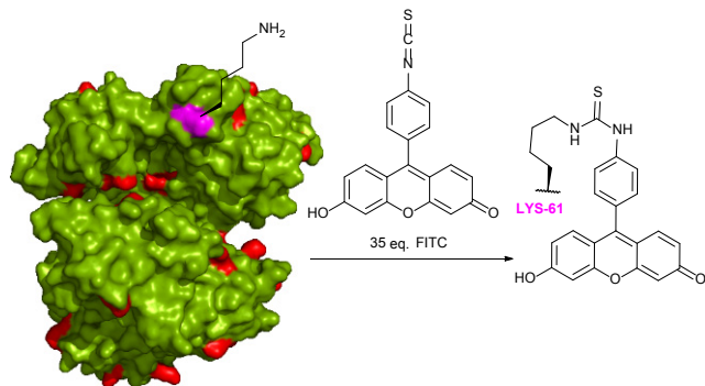
Fig. 4. Selective fluorescent labelling of LYS-61 residue (shown in magenta) of rabbit skeletal muscle G-actin (pdb: 2VYP reported by Buttick. 42 Such a high level of selectivity towards LYS-61 residue over other 33 lysine residues present in proteins (shown in red) remains unclear, but is hypothesised to be due to anomalously low pK_a value thereof.
