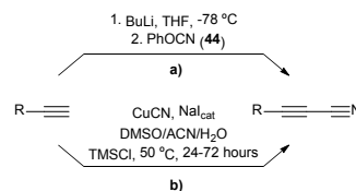
Scheme 21. Two main approaches used for arylalkynes cyanation: a ) with phenylcyanate ( 44 ); b ) by means of oxidative cyanation in the presence of CuCN.
