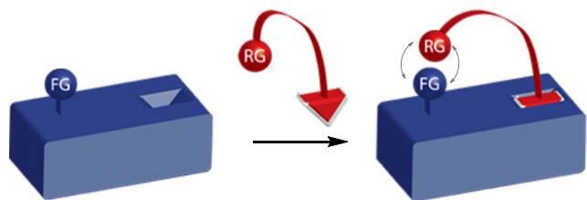
Fig. 88. Schematic representation of the proximity-driven approach for selective modification of macromolecules. Combining of promiscuous reactivity of the reactive group (RG, shown in red) with specific molecular recognition results in specific modification of the functional group of interest (FG, shown in blue).
