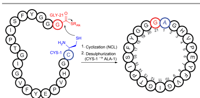
Fig. 78. Synthesis of 21-residue cyclic antibiotic peptide Microcin J25 via NCL-desulfurisation strategy resulting in alanyl-linked polypeptide chain developed by Yan and Dawson. 695 Reaction conditions: cyclisation – Tris-HCl, 6 M GndCl; desulfurisation – NaOAc, pH 4.5, 6 M GndCl, H 2 (Pd/Al 2 O 3 ).
