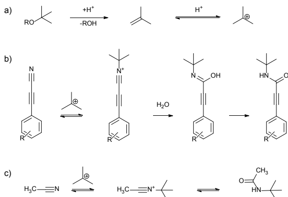
Scheme 19. Ritter reaction observed during tert -butyl deprotection. (a) Generation of the carbocation upon deprotection. (b) Ritter reaction on APN resulting in obtaining the corresponding tert -butyl amide. (c) Scavenging of the generated carbocation by acetonitrile.
