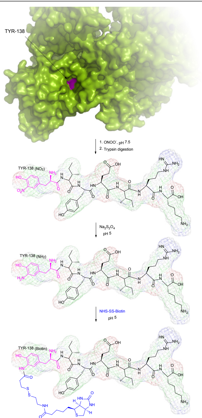
Fig. 49. Two-step biotinylation of HSA (pdb: 1AO6) described by Nikov et al. 478 a ) Preferential nitration of TYR-138 (shown in magenta) and TYR-411 residues of HSA with peroxyntirite was achieved using protocol described by Jiao and colleagues. 475 b ) Aminotyrosine of the peptide 138 YIYEIARK 144 , obtained after the step of reduction with sodium dithionite and following digestion of nitrated HSA with trypsin, were selectively modified with a cleavable biotin-containing reactant at pH 5.0.
