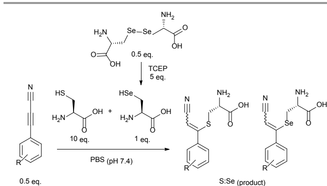
Scheme 43. Scheme of the comparative study for S vs Se selectivity.
