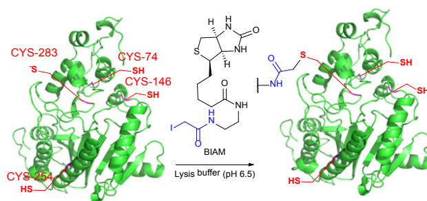
Fig. 18. Biotinylation of low- pK_a cysteine residue of rabbit muscle creatine kinase (CK, pdb: 2CRK) by BIAM. 248 The charge interaction between the negatively charged thiolate and the positively charged amino acid residues nearby results in significantly lower pK_a value of the CYS-283 residue (6.5). Consequently, selective alkylation thereof becomes possible in the presence of three other cysteine residues with higher pK_a values (8.0-9.0).
