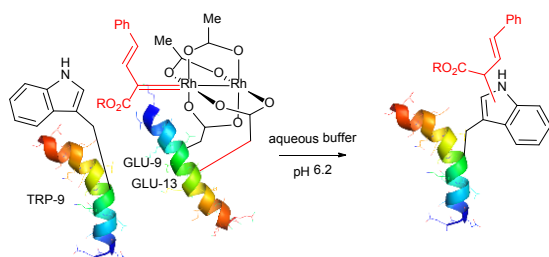
Fig. 41. Selective covalent labelling of TRP-9 residue of the peptide QEI-SALEK W SALEQEISALEK with its complementary dirhodium metallopeptide KISALQKQKESALEQKISALKQ described by Popp and Ball. 441 Rhodium cluster, chelated with two glutamate residues, is brought to a proximity of the reactive Trp residue by peptides coils self-assembling, resulting in selective peptide modification on TRP-9. Peptide structures were simulated using RaptorX web server. 435
