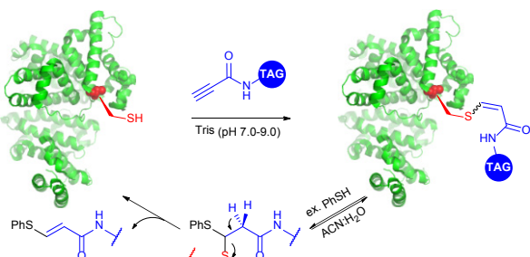
Fig. 37. Cleavable labelling of BSA (pdb: 3V03) with arylalkynone reagents elaborated by Che and associates. 409
