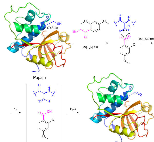
Fig. 19. Photolysis of CYS-25 residue located in papain's active site after its labelling with 2-bromo-2',4'-dimethoxyacetophenone results in the formation of the unstable thioaldehyde, which readily hydrolyses to give the corresponding aldehyde. 253,254
