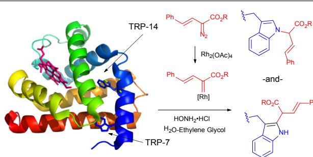
Fig. 39. Modification of horse heart myoglobin (pdb: 1YMB) with rhodium carbenoids described by Francis et al. 438 A 100 \mu M solution of myoglobin was exposed to stabilised vinyl diazo precursor (10 mM) and \text{Rh}_2(\text{OAc})_4 (100 \mu M) for 7 h. N - and C -derivatisation of indole rings of both Trp residues - TRP-14 and TRP-7 - were identified by the mass reconstruction. An excess of hydroxylamine hydrochloride (75 mM) is crucial for the efficiency of the conjugation, although its mode of action was not elucidated.
