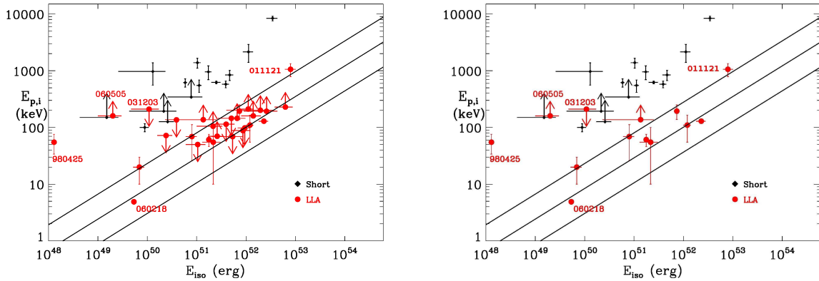
Figure 8. Location in the E_{p,i} - E_{iso} plane of LLA GRBs sample. Left, comparison of both short and long GRBs. Right, compared to short events, with firm measurements and non-compatible lower limits on E_{p,i} only.
