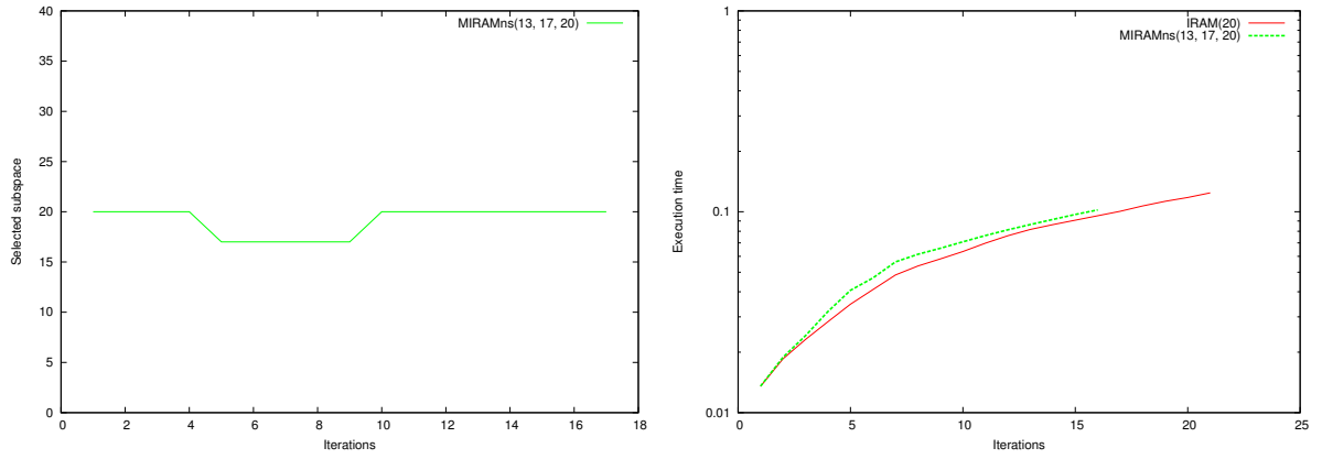
FIGURE 4.23: Execution time of MIRAMns(13,17,20) versus IRAM(20) for AM_1000 matrix, \text{tol}=10^{-8}
