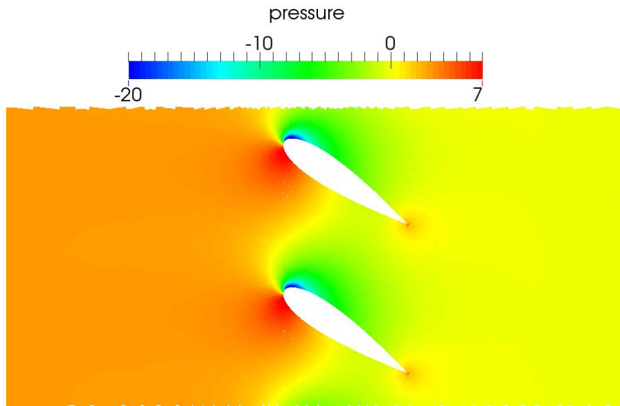
Figure 5.18: Pressure field of the rotating NACA after t = 11.8s plotted on the SPH particles and the FV mesh. A rotation speed of \omega = 0.03 rad/s is imposed. This instance corresponds to an angle of attack of 33.4^\circ .
