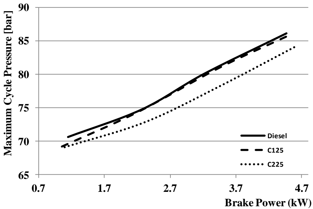
Figure 4-7, Pressure Cycle .
