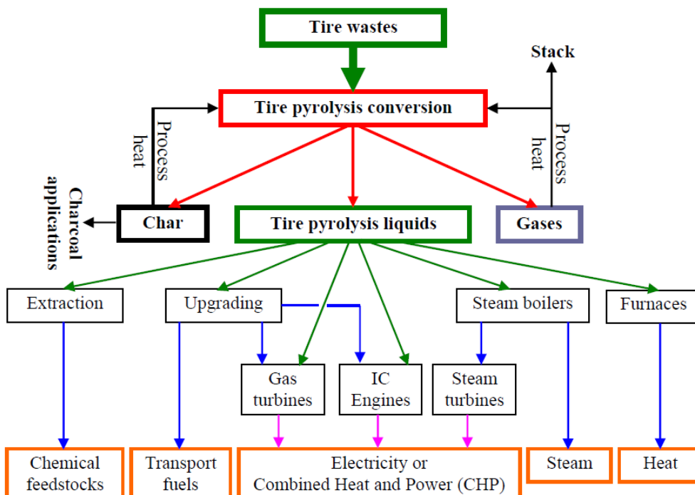
Figure 1-2:- Tire pyrolysis conversion and applications of products.
