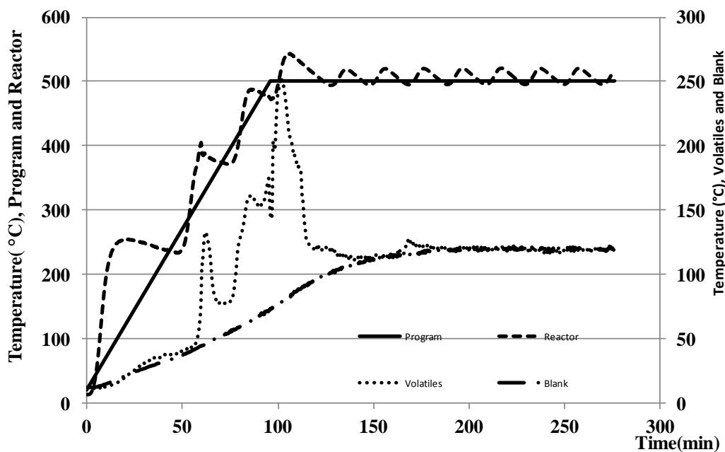
Fig 3-4, Temperatures' behavior of E2, Program, Reactor, Volatiles, and Blank
