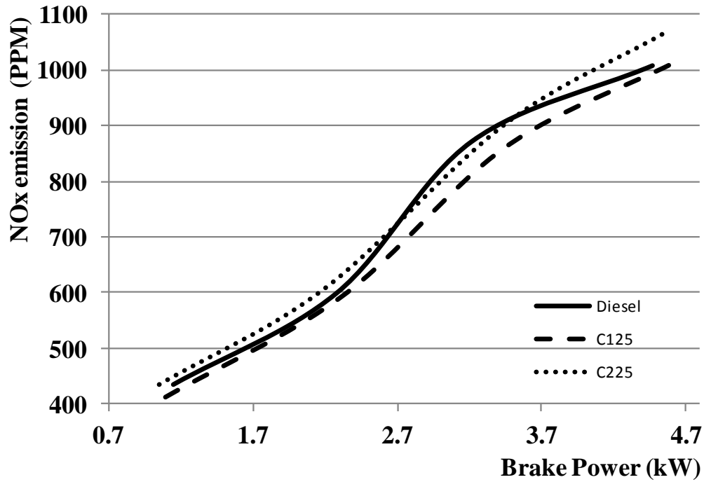
Figure 4-6, NOx emission of C125, C225 and Diesel.
