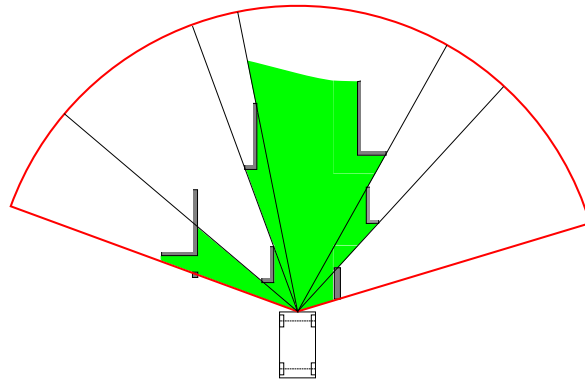
(a) Data interpretation of a lidar point cloud.
