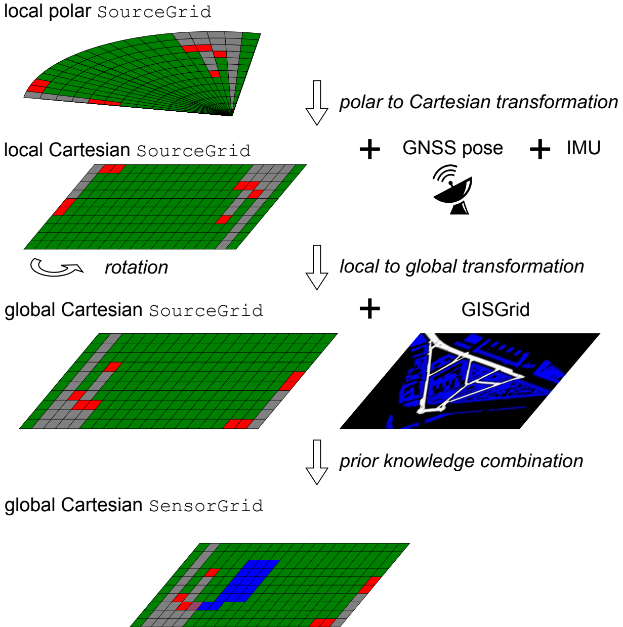
Figure 5.3 – Transformation from SourceGrid (SoG) to SensorGrid (SG).
