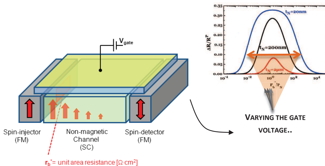
Figure 1.9 Principle of gate modulation of the r_b^*/r_N ratio. A prototypical top-gated lateral spinvalve is represented. The gate is potentially able to tune both the semiconductor resistivity and the interface resistance, and the possible change in the r_b^*/r_N ratio results in a displacement along the orange arrow in the MR plot.
