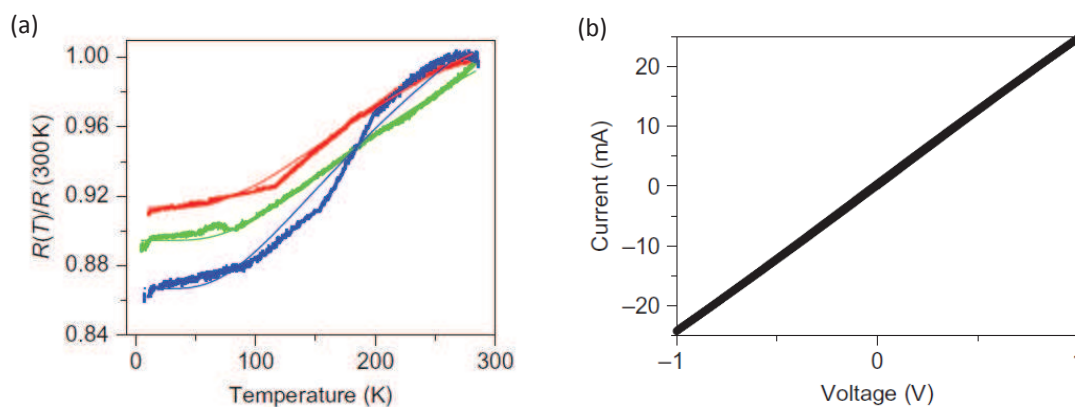
Figure 2.18 a) Normalized R(T) measurements of three independently prepared STANWs devices, between room temperature and 1.5 K (in vacuum, using an AC bridge technique). Initial resistances for each sample at 300 K: 22 (red), 45 (green), 360 (blue). Each set of data is fitted (thin lines) using a quasi-one-dimensional model of the resistance. b) I-V curve indicating current values of several tens of milliamperes at high bias ( \pm 1 V).
