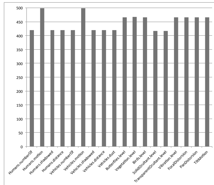
Figure 11.3: # configurations optimizing one quality attribute.
