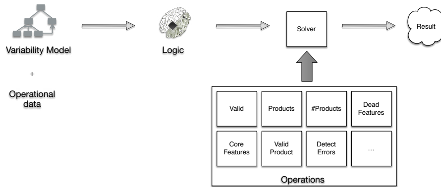
Figure 2.6: Automated analysis of feature models process .
