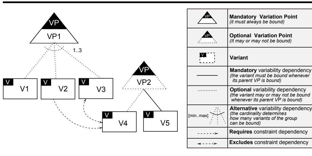
Figure 2.3: OVM notation.
