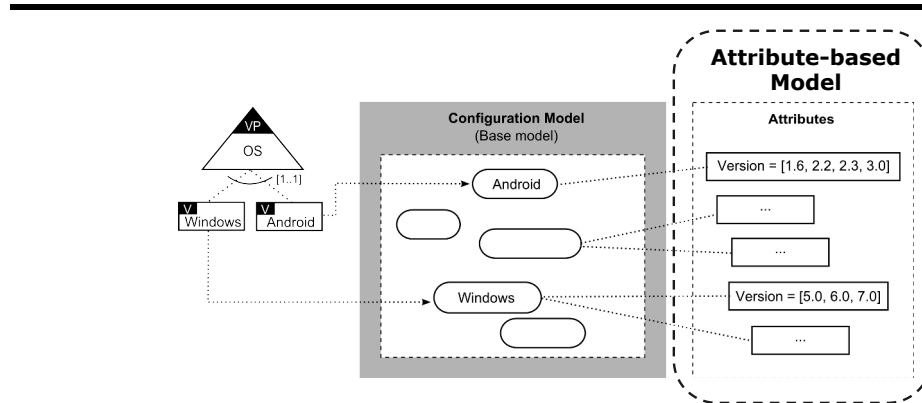
Figure 2.4: OVM with attributes.
