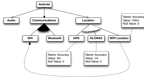
Figure 2.2: Attributed feature model example.
