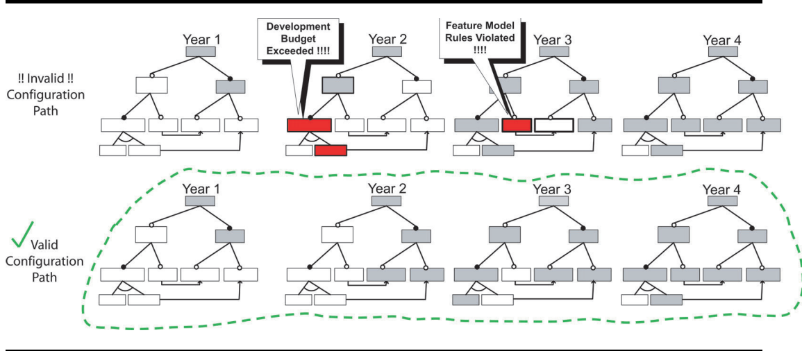
Figure 8.1: Potential configuration paths.
