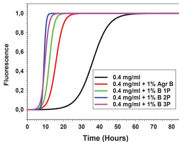
Figure 1.8: Repeated seeding leads to a decrease of T_{lag} and an increase of the apparent rate of polymerization ( 1/\tau ). Kinetics of amyloid polymerization of the rPrP at 0.4 mg/ml in buffer B at room temperature was obtained in a 96-well plate. The experimental results were normalized in order to clearly evidence that the T_{lag} and speed polymerization. The first kinetic (black line) was obtained without seeding. All the other curves were obtained after seeding at 0.004 mg/ml using the previous amyloid as presented on the figure.
