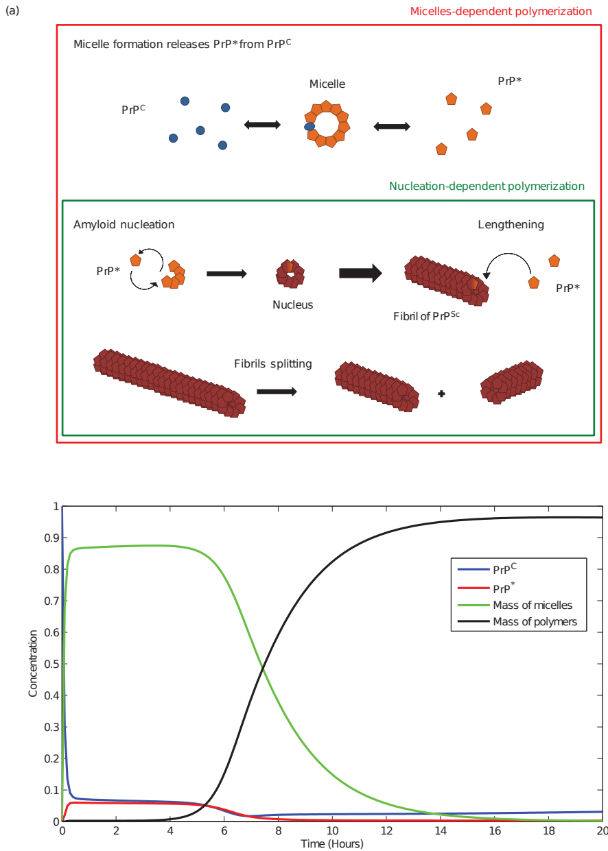
Figure 2.4: A mathematical model describing the micelle and amyloid dynamic. a, Schematic representation of the model associated to the kinetic equations in Table 1. The blue spheres represent the PrP C monomers. In yellow, the PrP* stabilized by micelles. In red, the PrP Sc polymers, binding PrP* at its ends and are able to split. b, Qualitative normalized dynamics of the model.
