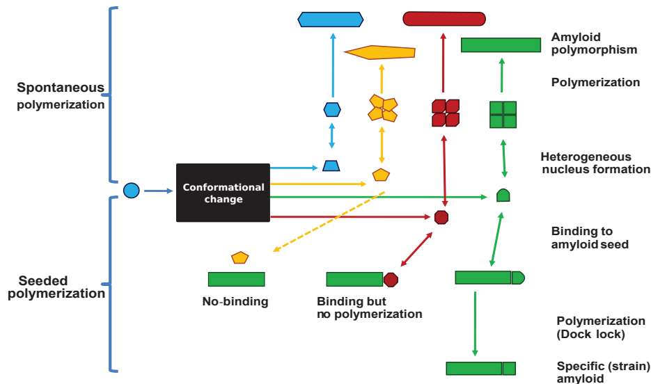
Figure 1.11: Model of prion amyloid formation. Amyloidogenesis of prion protein in vitro is a nucleation-dependent polymerization process. However, nucleation is not the main determinant of the lag time, another mechanism should be postulated to explain the weak dependency to the initial concentration of monomers and the residual lag time observed during seeded polymerization. This mechanism is symbolized by a black box and some hypotheses on its nature are proposed in the Discussion. The diversity of the amyloids obtained [207] with the same purified prion protein implies the genesis of different conformers of the monomer, but only the corresponding conformer can react with a precise amyloid used for seeding. This hypothesis would explain not only the heterogeneity of amyloids but also the perpetuation of the strains and results presented here (Figure 1.6 panel C) that has shown an inverse dependency of the lag time with initial concentration at constant seed.
