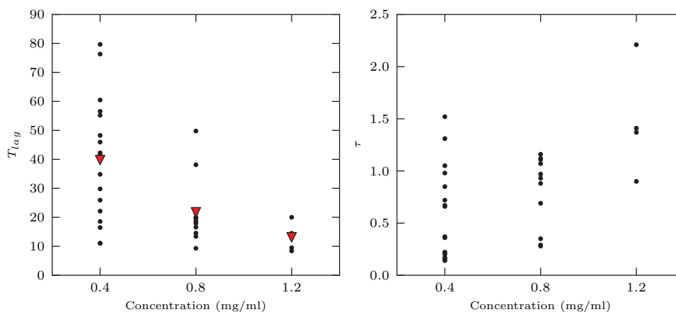
Figure 1.4: Lag time ( T_{lag} ) and rate ( \tau ) dependency of the initial concentration of monomeric rPrP. Kinetics analyses were performed as described in Section 1.2.3. Kinetics of amyloid polymerization of rPrP at different concentrations in buffer B at room temperature was obtained in a single experiment (a 96-well plate). T_{lag} was calculated according to (1.7) (on the left) and \tau was deduced directly from (1.6) (on the right).
