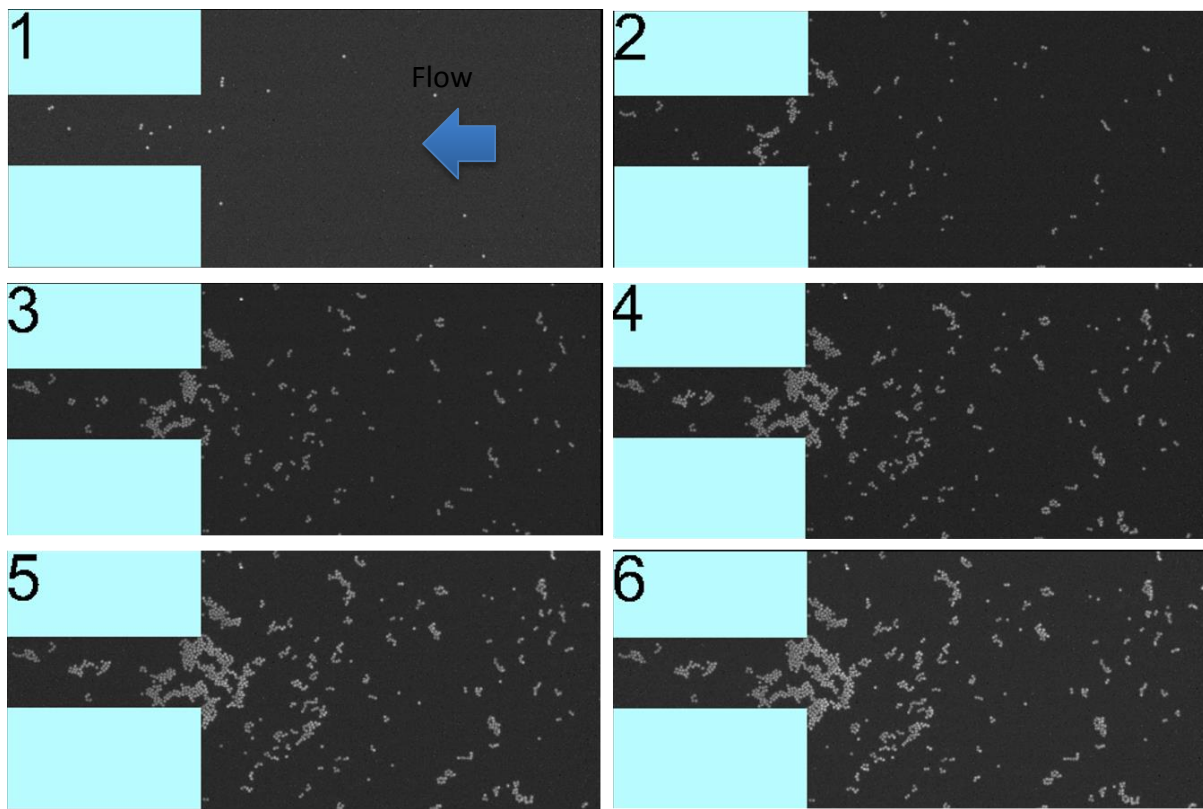
Figure 35: Consecutives images of a clog formation within a constriction in a 2d channel (the main channel height is equal to the pore height H=1.2D , D being the particle diameter). Blue rectangles represents the wall of the channel. Deposition of particles occurs everywhere and the clogging (image 6) occurs in the reservoir and not in the channel.
