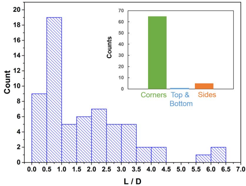
Figure 86: Distribution of the positions of the particles captured directly by the pore walls. Inset: repartition of the captured particles between sides of the pore.
