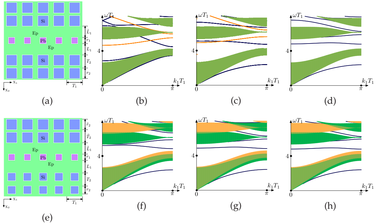
Figure 5.2: (a) Layer between two identical half-spaces. The spectra for (a) with (b) the uniform plate (c) L_1 = 0.6 mm; (d) L_1 = 0.7 . In Figs. (b) and (c), the black and grey (dark blue and orange online) lines are dispersion branches for symmetric and antisymmetric waves. (e) Layer between two dissimilar half-spaces. The spectra for (e) with (f) L_1 = 0.6 mm, (g) L_1 = 0.7 mm, (h) L_1 = 0.5 mm. The light grey and dark grey areas (yellow and dark green online) correspond to the spectra of the propagating waves in the upper and lower substrate, correspondingly. The grey areas (light green online) correspond to the superposition of these spectra.
