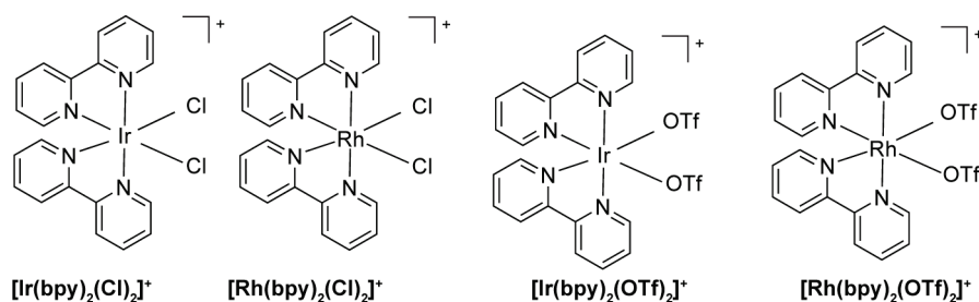
Figure I-24 Scheme of compounds studied by Bolinger et al. in 1988 (OTf = trifluoromethanesulfonate).
