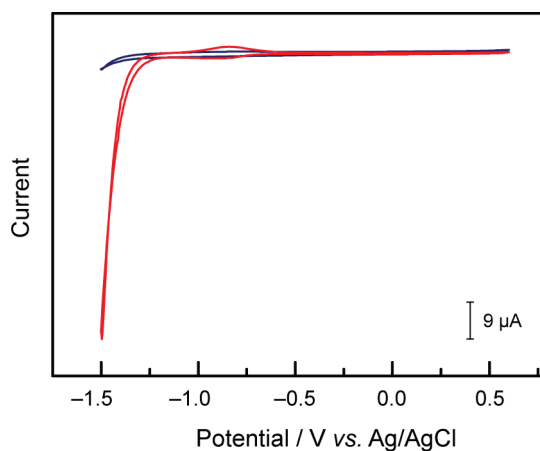
Figure V-21 Comparison of the cyclic voltammograms under Ar in water in a phosphate buffer (pH = 7) of a tpy-modified glassy carbon electrode after metallation with CoCl 2 (— red) and a polished bare glassy carbon electrode (— blue). ‡
