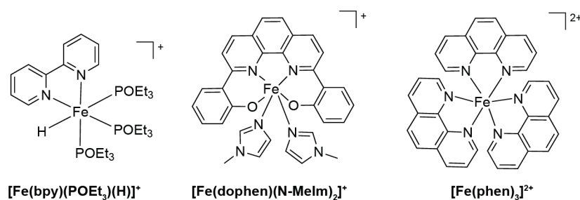
Figure I-40 Structure of Fe catalysts studied by Chen et al. in 2010 (left), Pun et al. in 2002 (centre) and Durand in 1988 (right).
