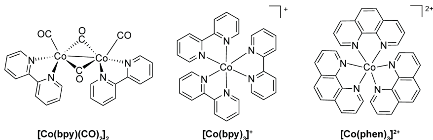
Figure I-43 Structures the catalysts studied by Sutin and of the proposed Co dimer (reference 111).
