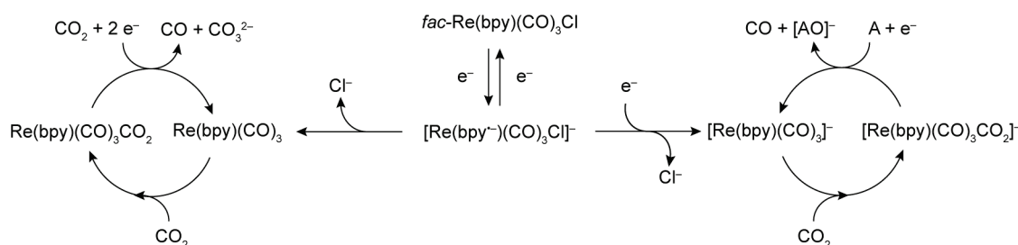
Figure I-29 One- and two-electron pathway mechanisms proposed by Meyer in 1985. “A” is an oxide ion acceptor.
