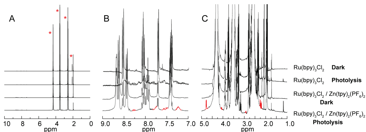
Figure III-28 1 H NMR spectra for the photolysis of experiments of 1.0 mM Zn-tpy in the presence of 2.0 mM Ru(bpy) 3 Cl 2 (H 2 O) 6 in a CO 2 -saturated 5:1 volumetric ratio of acetonitrile-d 3 to triethanolamine. From top to bottom, the spectra represent Ru(bpy) 3 Cl 2 (H 2 O) 6 in the dark; Ru(bpy) 3 Cl 2 (H 2 O) 6 photolysed for 6h; both Ru(bpy) 3 Cl 2 (H 2 O) 6 and Zn-tpy in the dark; and both Ru(bpy) 3 Cl 2 (H 2 O) 6 and Zn-tpy photolysed for 6h. (a) The full spectra are shown with the intense peaks associated with TEOA marked by *. (b) Aromatic resonances are shown with peaks only observed post-photolysis of Zn-tpy presented in red. (c) Aliphatic resonances are shown with peaks only observed post-photolysis of Zn-tpy presented in red. §
