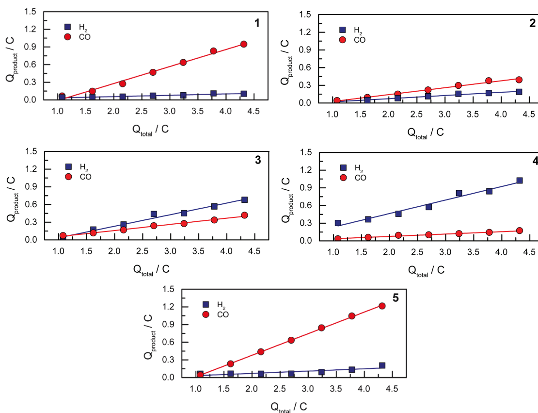
Figure IV-18 Charge corresponding to the products measured (H 2 : blue squares, CO: red circle) vs. the total charge passed during the electrolyses of 1-5 as described in Figure IV-17. The slopes of the linear fits, corresponding to the faradic efficiencies, are given in Figure IV-19.†
