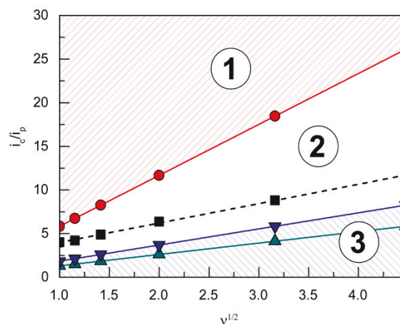
Figure IV-12 Theoretical values for i_c/i_p^0 for 3 in the presence of 60 mM acetic acid and various scan rates plotted using equation IV-9. Red circles represent values where k_{cat} = k_1 = 1100 \text{ M}^{-1}\text{sec}^{-1} . Blue triangles represent values where k_{cat} = k_2 = k_1/10 = 110 \text{ M}^{-1}\text{sec}^{-1} . Green triangles represent values where k_{cat} = k_2 = k_1/20 = 55 \text{ M}^{-1}\text{sec}^{-1} .
