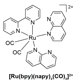
Figure I-22 Structure of the CO 2 reduction catalyst reported by Tanaka and Mizukawa (see reference 58).
