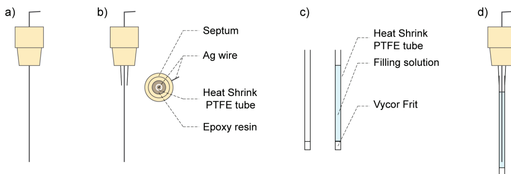
Figure II-9 Schematic representation of the process implemented to make reference electrodes used for bulk electrolysis as described within the text.
