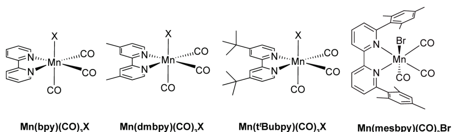
Figure I-37 Structure of the various Mn-based catalysts studied by Deronzier and Kubiak (X = Cl or Br).
