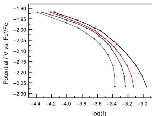
Figure III-31 Plot of applied potential vs. log(current(A)) extracted from the experiments described in Figure III-30 (black squares: 2 mM, red circles: 1 mM, blue triangles: 0.75 mM and green triangles: 0.5 mM of Co-tpy ). At all Co-tpy concentrations, the slope of the linear fit (not represented) of the -1.9 V to -2.1 V region is ~135 mV/dec). §
