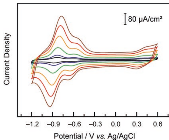
Figure V-13 Cyclic voltammograms under Ar in DMF, TBAPF 6 0.1 M, of a glassy carbon electrode modified with the tpy ligand and freshly metallated with CoCl 2 and rinsed at 50 (— black), 100 (— blue), 250 (— green), 500 (— orange), 750 (— red) and 1000 (— brown) mV/s.
