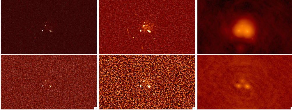
Figure 5.2: Dirty maps resulting from simulated observations of the model cluster at z=0.5 for Cases A, B and C (from left to right ). Top panels show results for SKA1-MID, bottom panel for SKA1-SUR.
