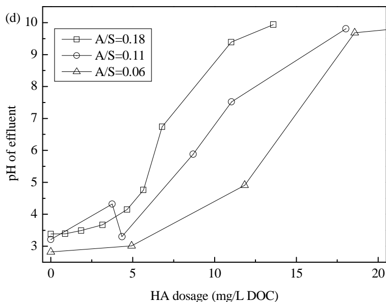
Fig. 3.19. Comparison of DAF performance under different A/S ratios: (a) TNP removal efficiency; (b) residual DOC; (c) zeta potential; (d) pH values.
