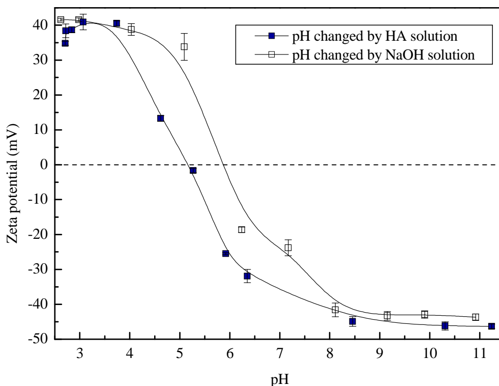
Fig. 3.2. Zeta potential as a function of in the presence and in the absence of HA.
