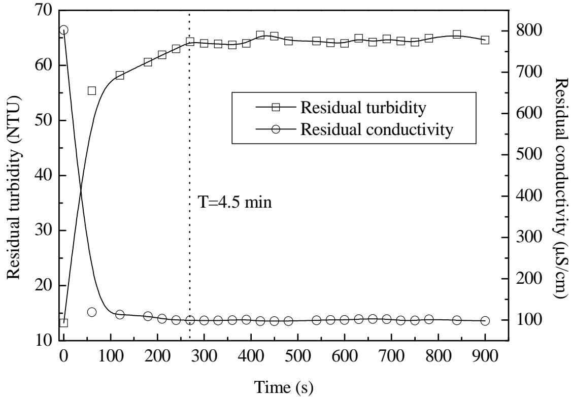
Fig. 3.13. Residual turbidity and residual conductivity varying with the flotation time.
