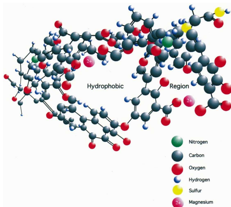
Fig. 1.7. Portion of the proposed “type” structure of HA (Wandruszka, 2000).
