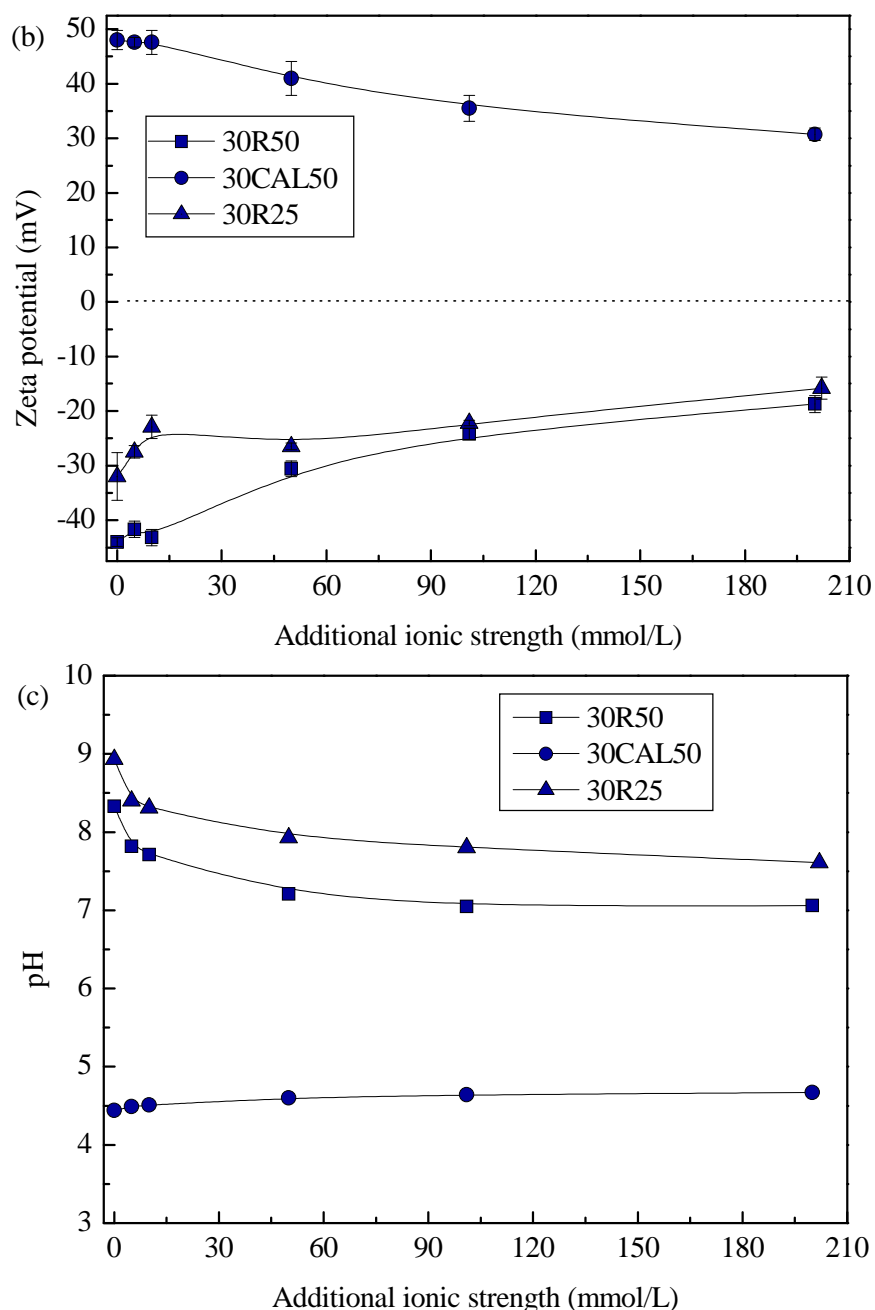
Fig. 2.17. Effect of additional IS on properties of SNP suspension: (a) particle size, (b) zeta potential; (c) pH value.
