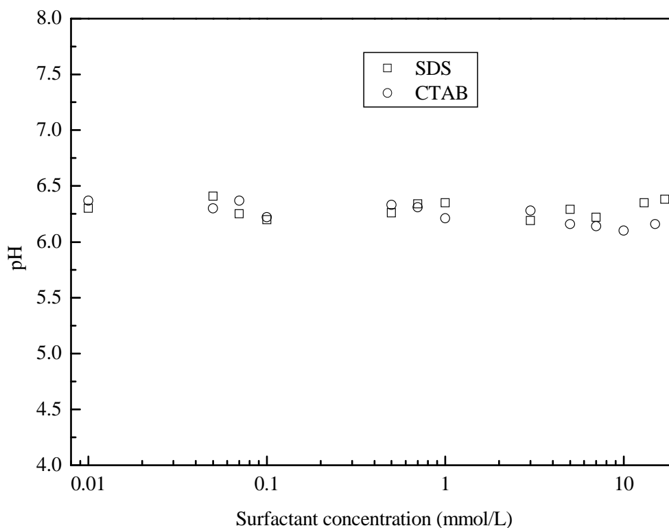
Fig. 2.20. The pH value of surfactant solution varying with surfactant concentrations.
