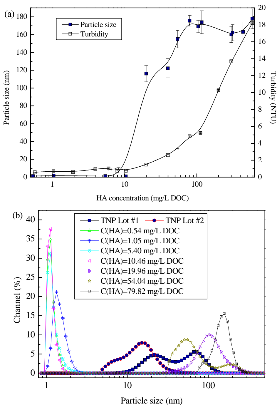
Fig. 2.10. (a) Particle size and turbidity varying with HA concentrations; (b) PSD patterns of TNPs and HA.
