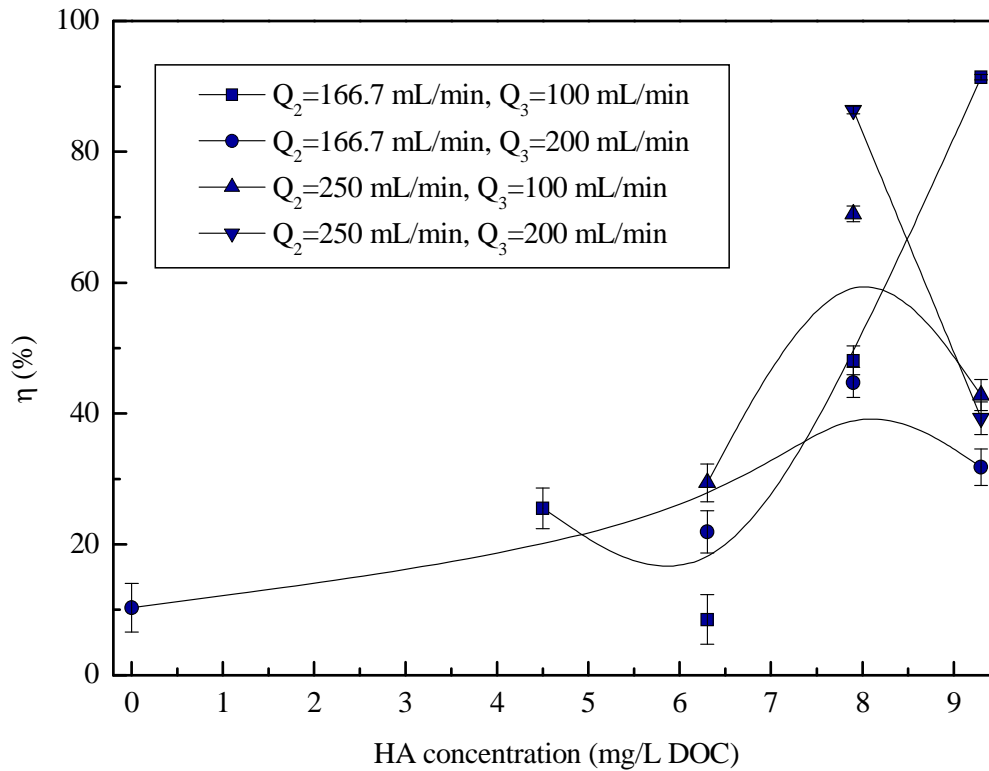
Fig. 3.14. Effect of HA concentration on TNP removal efficiency.
