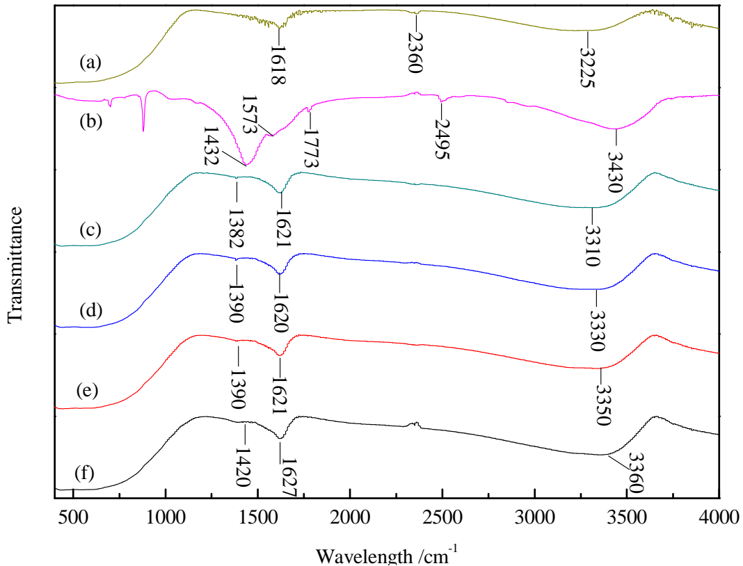
Fig. 3.6. FT-IR spectra of TNPs before and after surface modification by HA with various additive contents: (a) TNPs, (b) HA, (c) TNPs + 6.10 mg/L DOC HA, (d) TNPs + 7.06 mg/L DOC HA, (e) TNPs + 8.02 mg/L DOC HA, (f) TNPs + 9.15 mg/L DOC HA.
