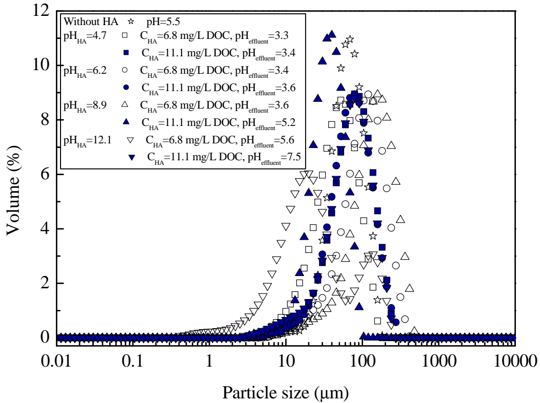
Fig. 3.23. Aggregate size distribution under different conditions.
