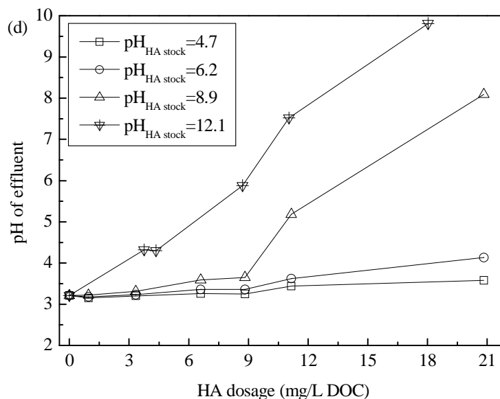
Fig. 3.18. Flotation behavior varying with HA dosage (The pH value of HA stock solution was adjusted to 4.7, 6.2, 8.9 and 12.1, respectively): (a) TNP removal efficiency, (b) HA removal, (c) zeta potential, and (d) pH of effluent.
