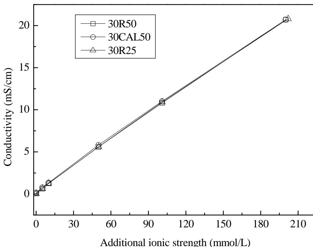
Fig. 2.16. Conductivity of SNP suspension varying with additional IS.
