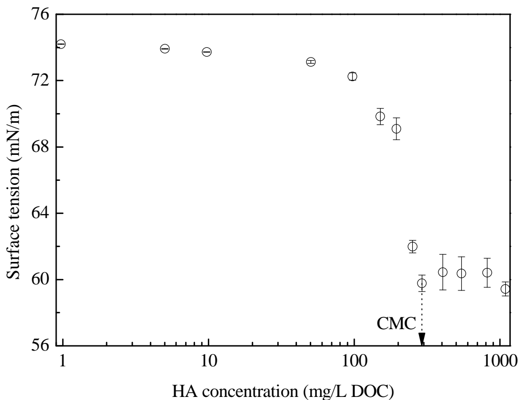
Fig. 2.9. Determination of CMC by surface tension measurement.
