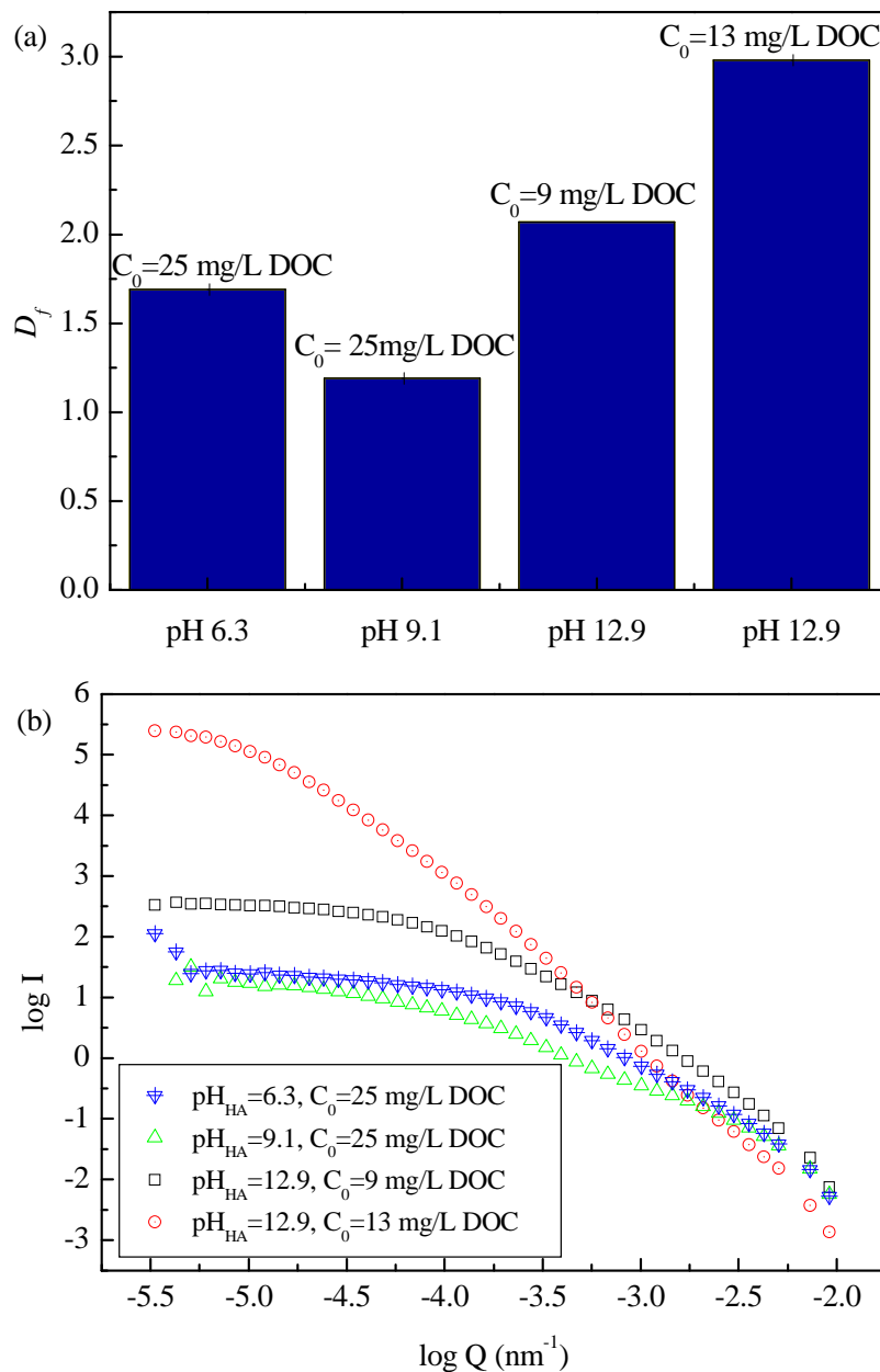
Fig. 3.11. Fractal dimension of TNP-HA aggregates at different pH of HA stock solution: (a) D_f variation; (b) \log I as a function of \log Q .
