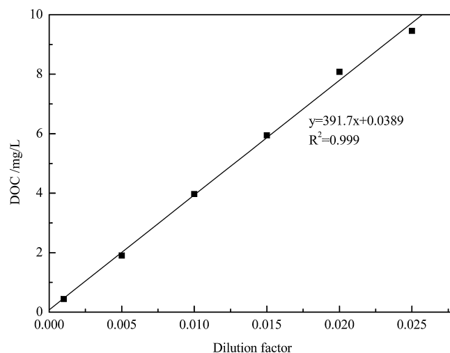
Fig. 1. DOC as a function of dilution factor of HA stock solution.
