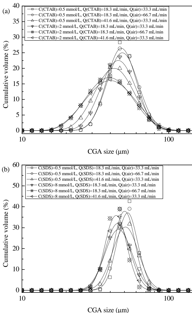
Fig. 4.20. CGA size distribution patterns under different generation conditions: (a) CTAB-CGAs; (b) SDS-CGAs.
