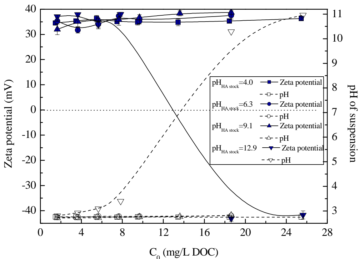
Fig. 3.9. Zeta potential and pH value of post-(adsorption-aggregation) suspension as a function of initial HA concentration.
