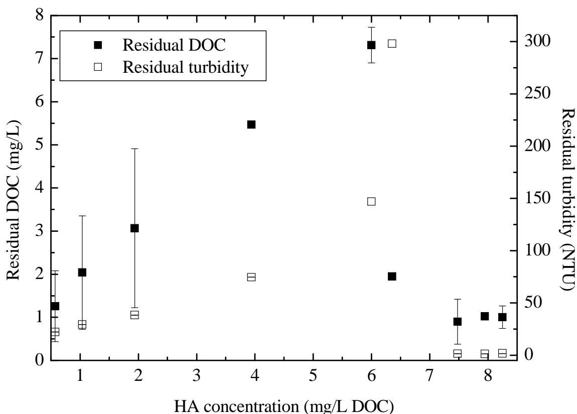
Fig. 3.7. Residual HA and residual turbidity as functions of HA concentrations.
