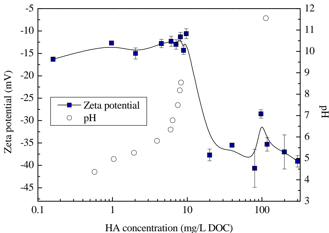
Fig. 2.11. Zeta potential and pH value varying with HA concentrations.
