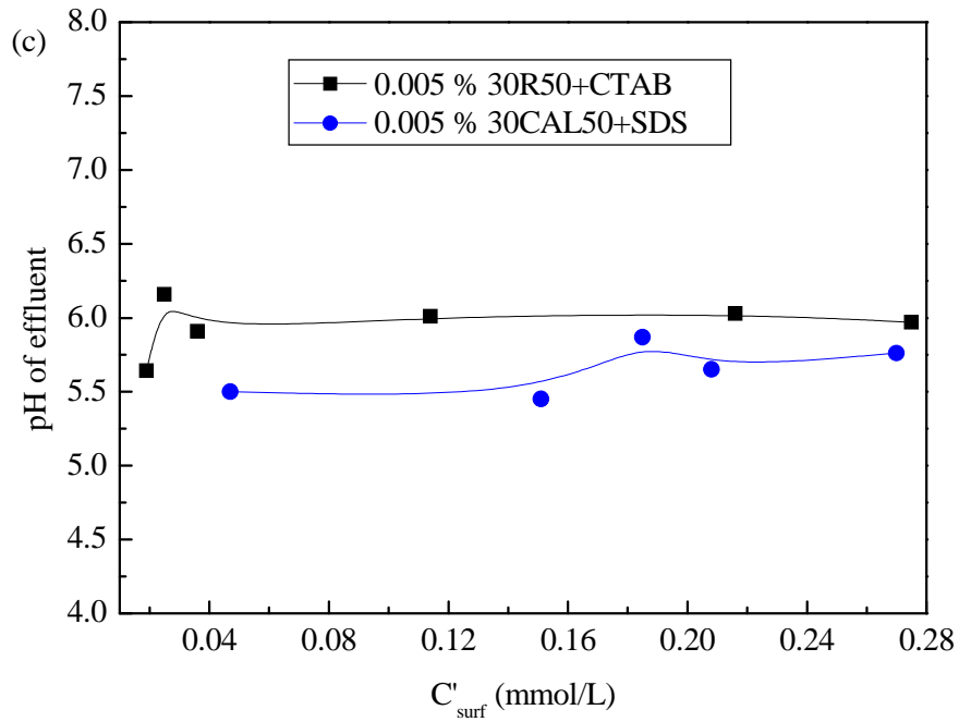
Fig. 4.27. Effect of surfactant concentration in the contacting zone of flotation cell on the performance of CGA-flotation: (a) SNP removal efficiency and zeta potential; (b) residual turbidity; (c) pH value after flotation.
