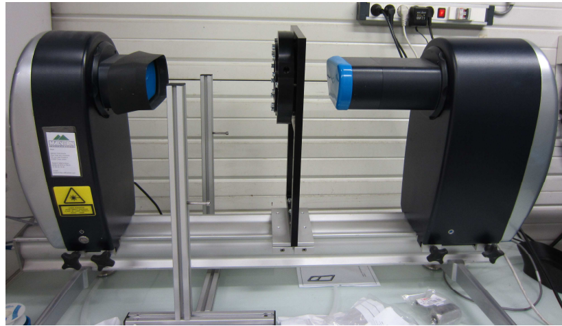
Fig. 4.10. Spraytec apparatus with measurement cell for size analysis.
