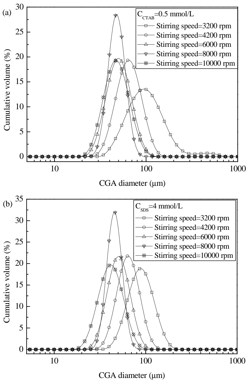
Fig. 4.15. Bubble size distribution of CGAs under different stirring speeds.
