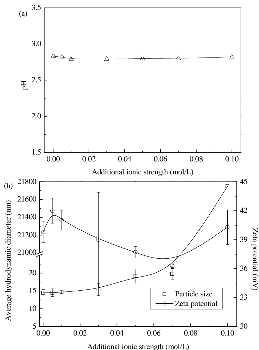
Fig. 2.6. Properties of TNP suspension varying with different additional IS: (a) pH; (b) particle size and zeta potential.
