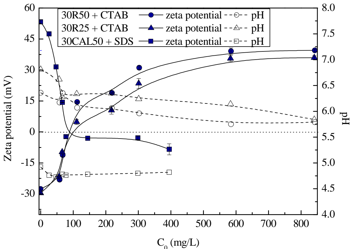
Fig. 4.24. Zeta potential and pH value of post-(adsorption-aggregation) suspension as a function of initial surfactant concentration.
