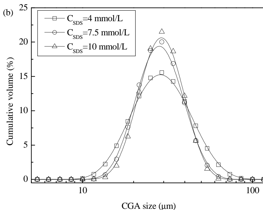
Fig. 4.17. CGA size distribution at different surfactant concentrations in the batch generation mode: (a) CTAB-CGAs and (b) SDS-CGAs.
