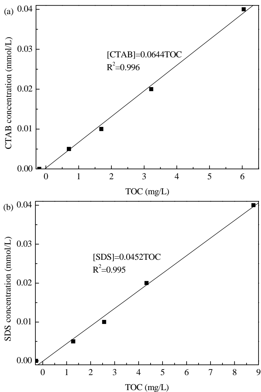
Fig. 4.22. Variation of surfactant concentration with TOC: (a) CTAB; (b) SDS.
