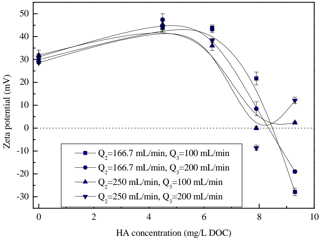
Fig. 3.15. Effect of HA concentration on zeta potential of treated TNP suspensions.
