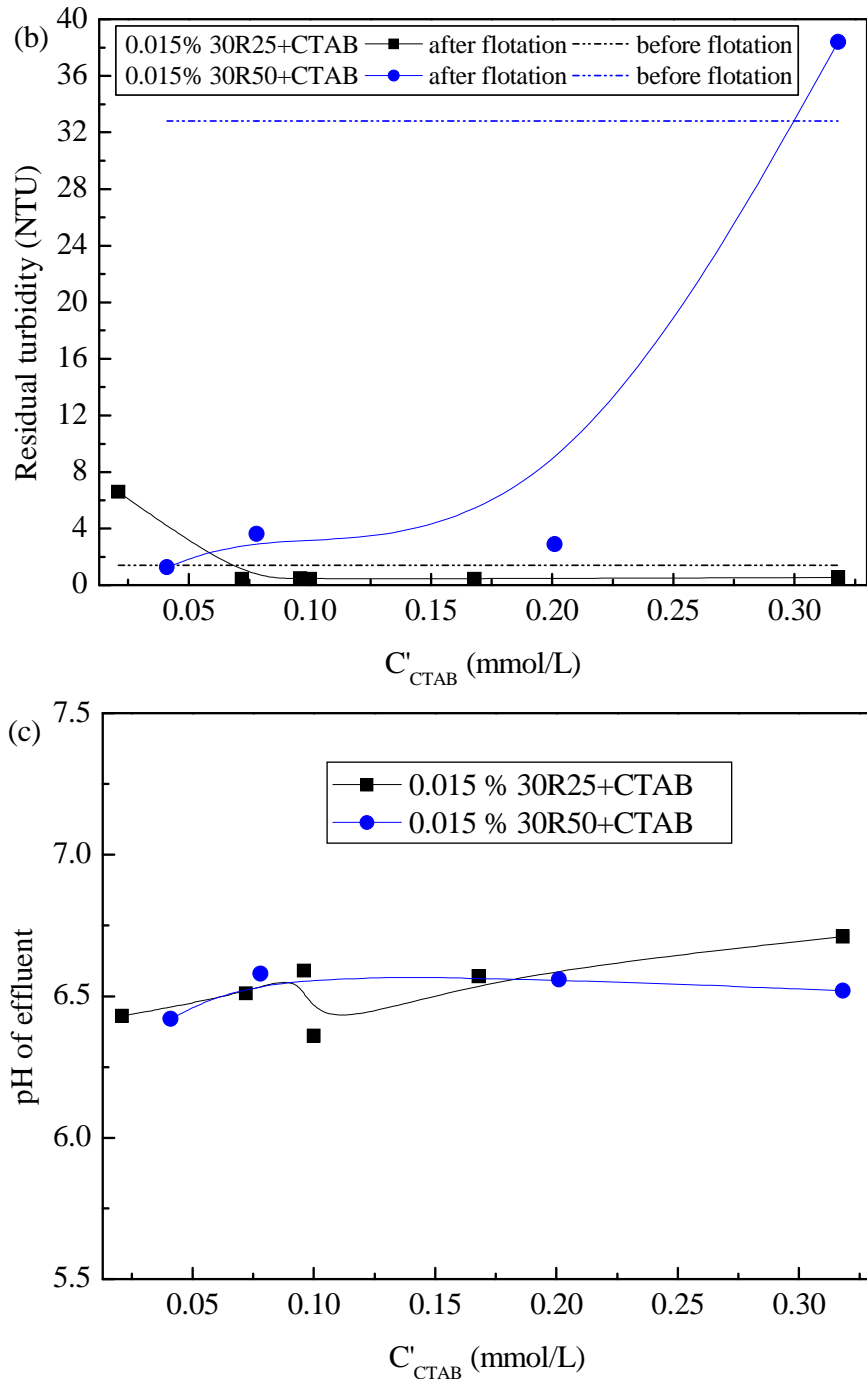
Fig. 4.29. Effect of NP size on the performance of CGA-flotation: (a) SNP removal efficiency and zeta potential; (b) residual turbidity; (c) pH value after flotation.
