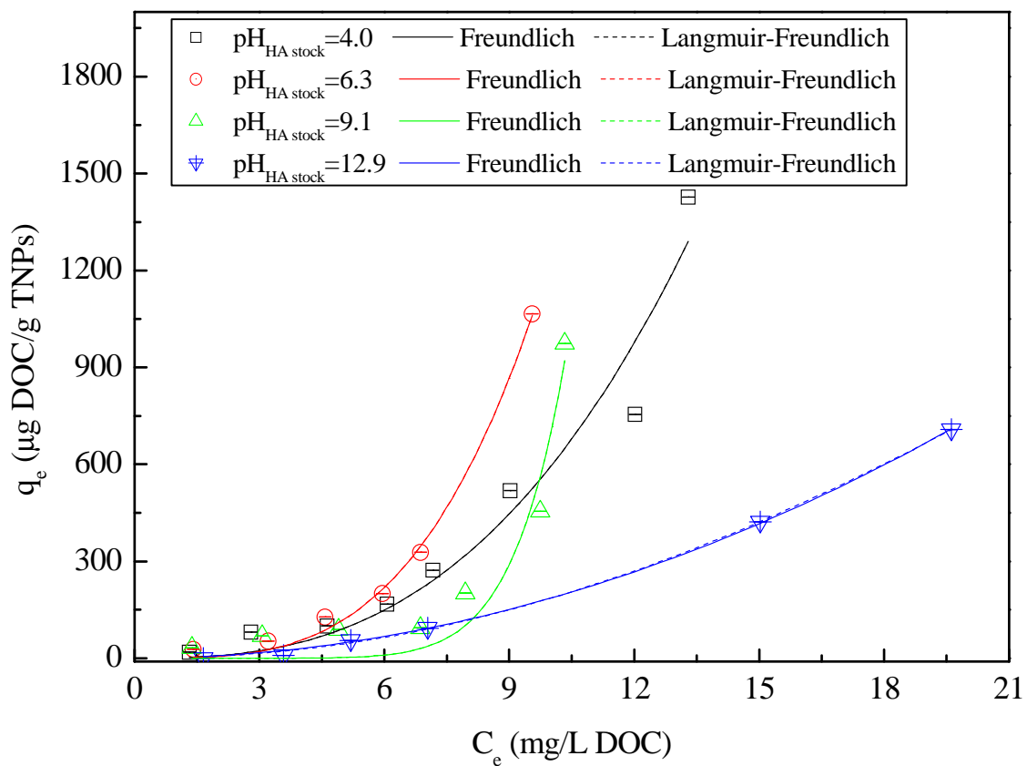
Fig. 3.8. Experimental data and fitting curves of Freundlich and L-F adsorption results of 0.15 wt.% TNP+HA.
