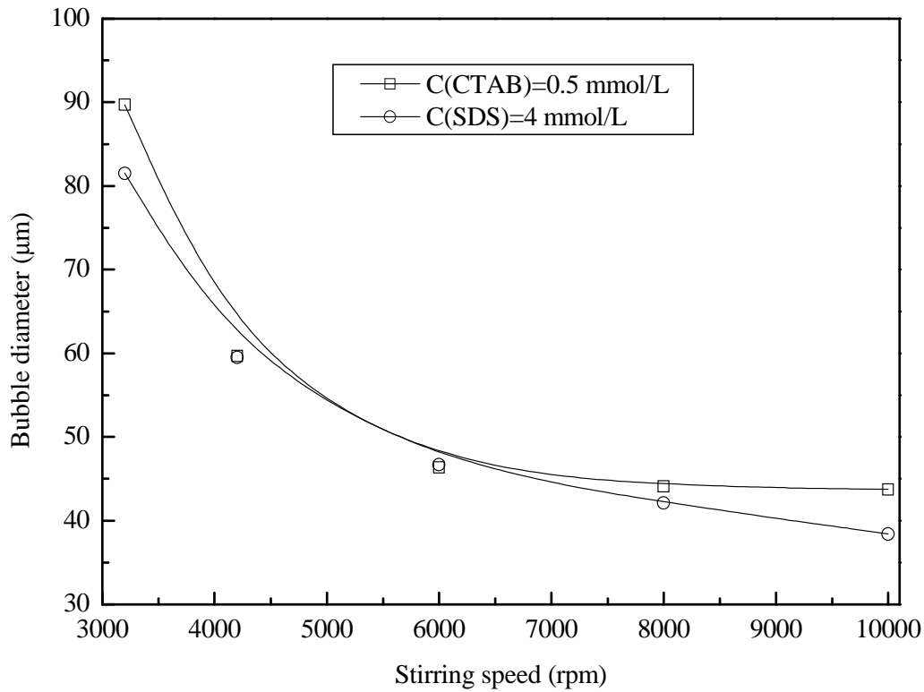
Fig. 4.16. Relationship between bubble size and stirring speed.
