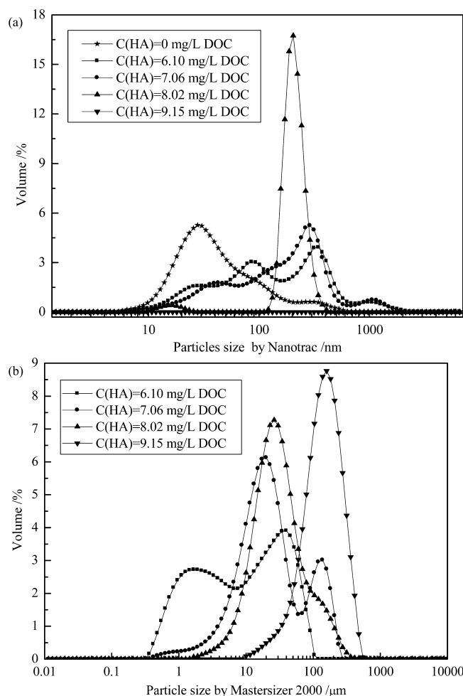
Fig. 9. Particle size distribution of surface modified TNP suspensions: (a) supernatant by Nanotracs; (b) precipitates/flocs by Mastersizer 2000.
