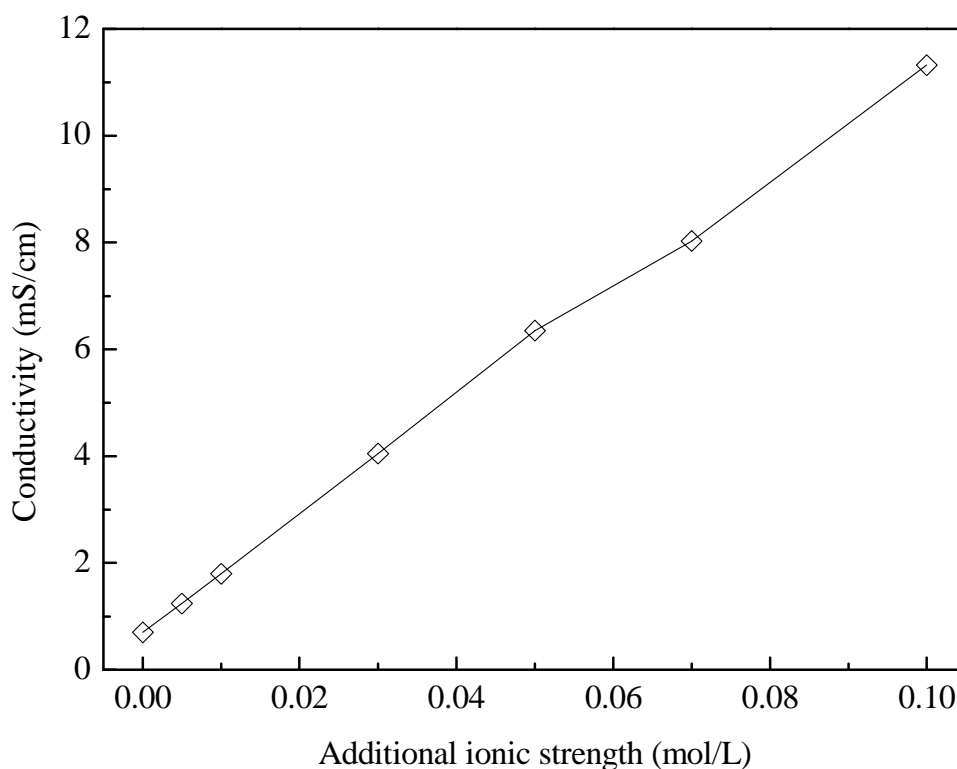
Fig. 2.5. Conductivity of TNP suspension varying with different additional IS.
