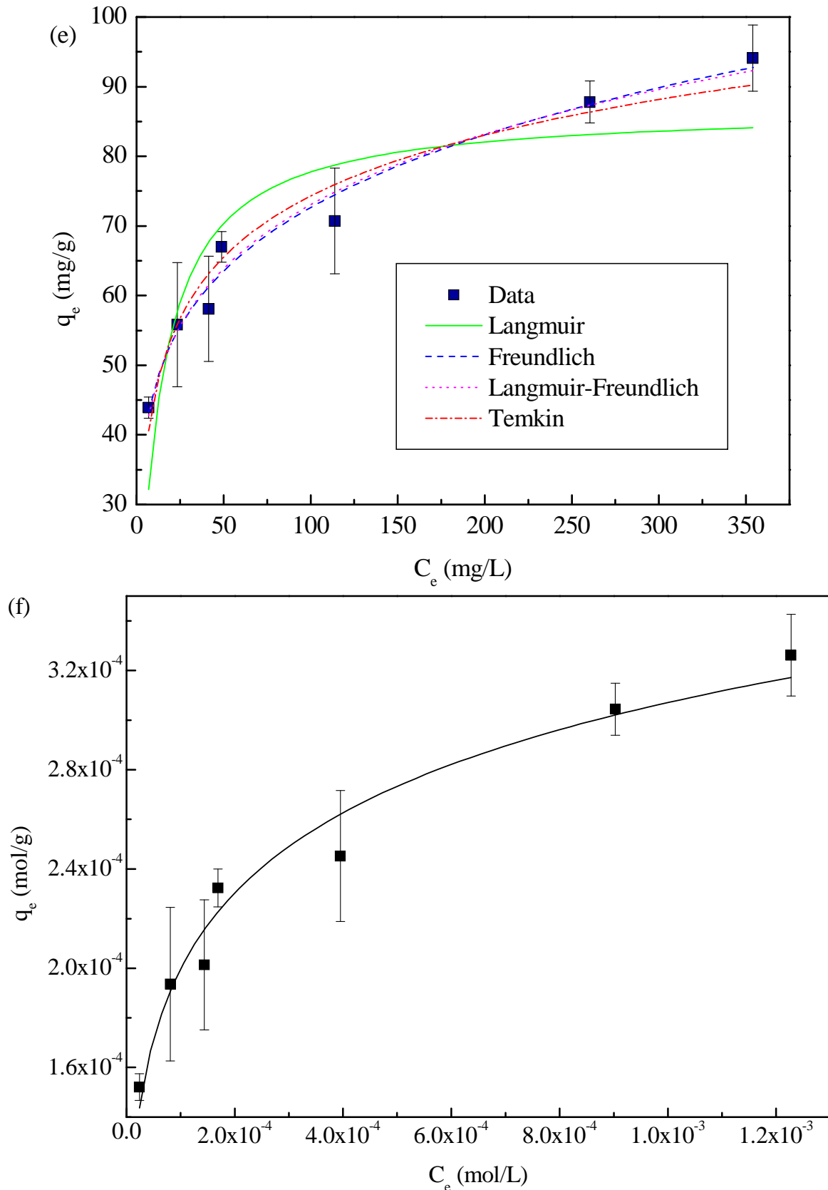
Fig. B. Adsorption results of 0.015 vol.% SNP+surfactant: (a), (c) and (e) experimental data and fitting curves of Langmuir, Freundlich, L-F and Temkin isotherms for 30R50+CTAB, 30R25+CTAB, and 30CAL50+SDS, respectively, (b), (d) and (f) experimental data and fitting curve of D-R isotherm for 30R50+CTAB, 30R25+CTAB, and 30CAL50+SDS, respectively.
