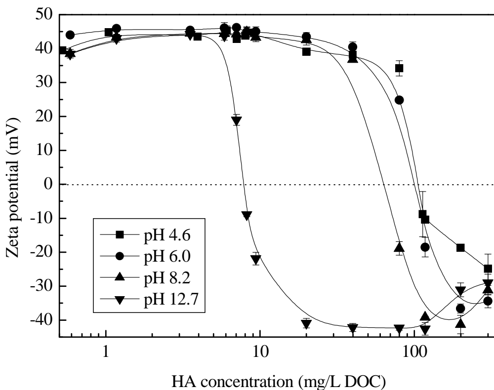
Fig. 3.3. Zeta potential as a function of HA concentration under different pH conditions.
