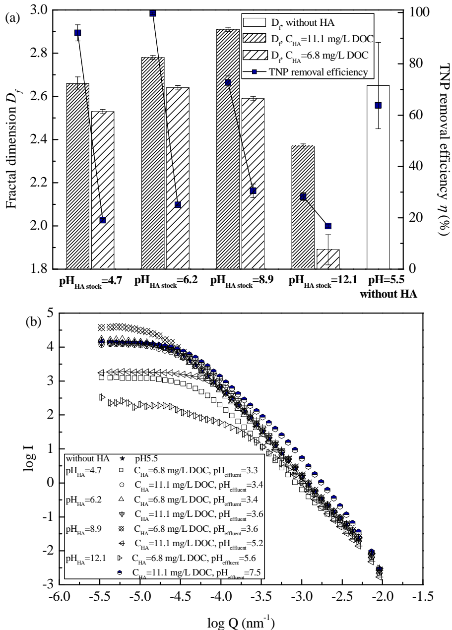
Fig. 3.24. (a) Comparison of fractal dimension values of flotation aggregates under different conditions (corresponding to Fig. 3.23); (b) Static light scattering plots of flotation flocs formed in different physiochemical conditions.
