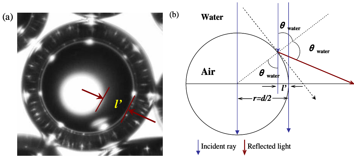
Fig. 4.6. Formation of the “dark layer” on the bubble image of optic microscope: (a) CGA photo; (b) schematic calculation of the dark-layer thickness.
