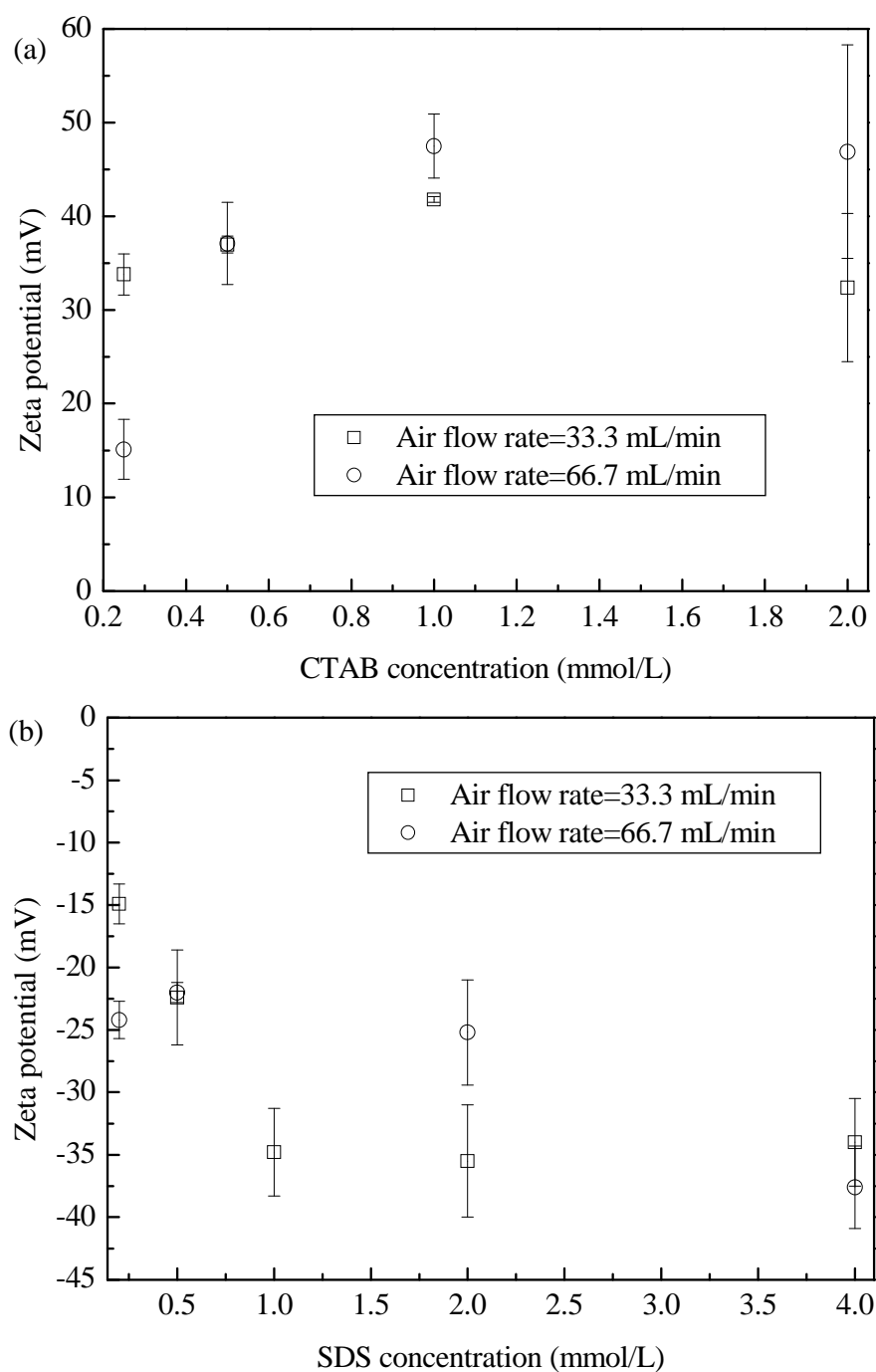
Fig. 4.21. Average CGA zeta potentials varying with the surfactant concentration at different air flow rate: (a) CTAB-CGAs;(b) SDS-CGAs.
