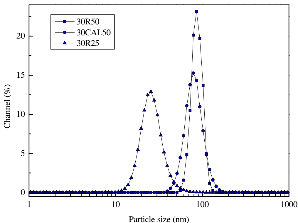
Fig. 2.12. Particle size distributions of different SNPs.
