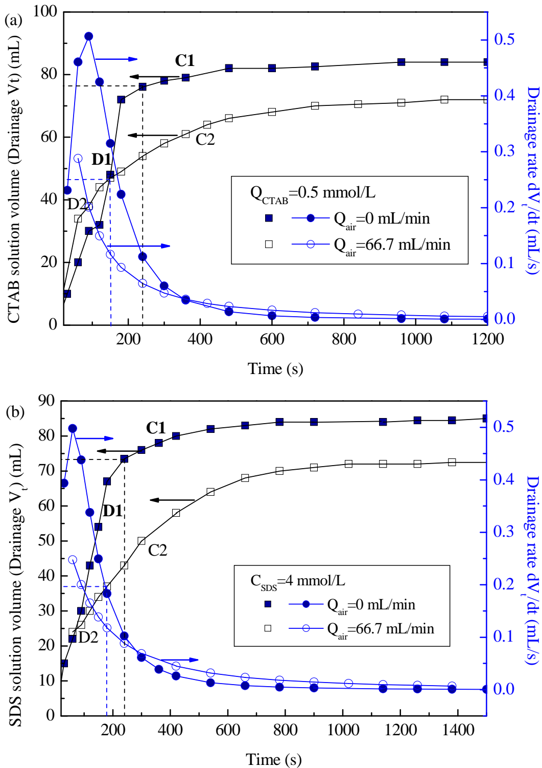
Fig. 4.9. Liquid drainage rate as a function of time: (a) CTAB-CGAs; (b) SDS-CGAs ( C_{\text{surf}} \approx 0.5\text{CMC} ). Arrows indicate corresponding axis.
