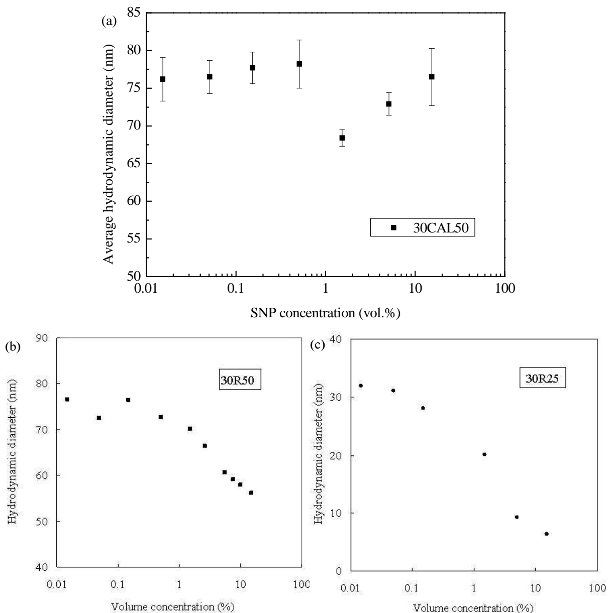
Fig. 2.13. Particle size varying with SNP concentration: (a) 30CAL50 (measured in this study), (b) 30R50 and (c) 30R25 (measured by Liu (2010)).
