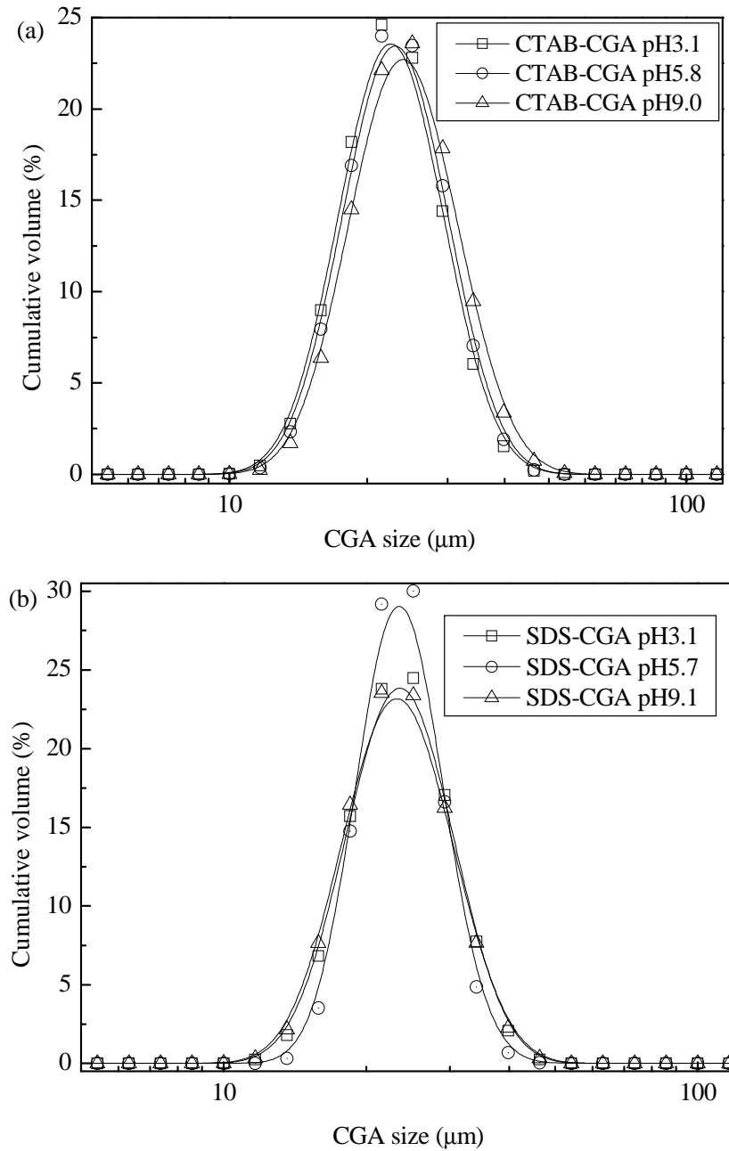
Fig. 4.19. CGA size distribution at different pH values ( C_{surf} \approx 0.5\text{CMC} , C_{CTAB} = 0.5 \text{ mmol/L} , C_{SDS} = 4 \text{ mmol/L} ) of surfactant solutions in the batch generation mode: (a) CTAB-CGAs and (b) SDS-CGAs.
