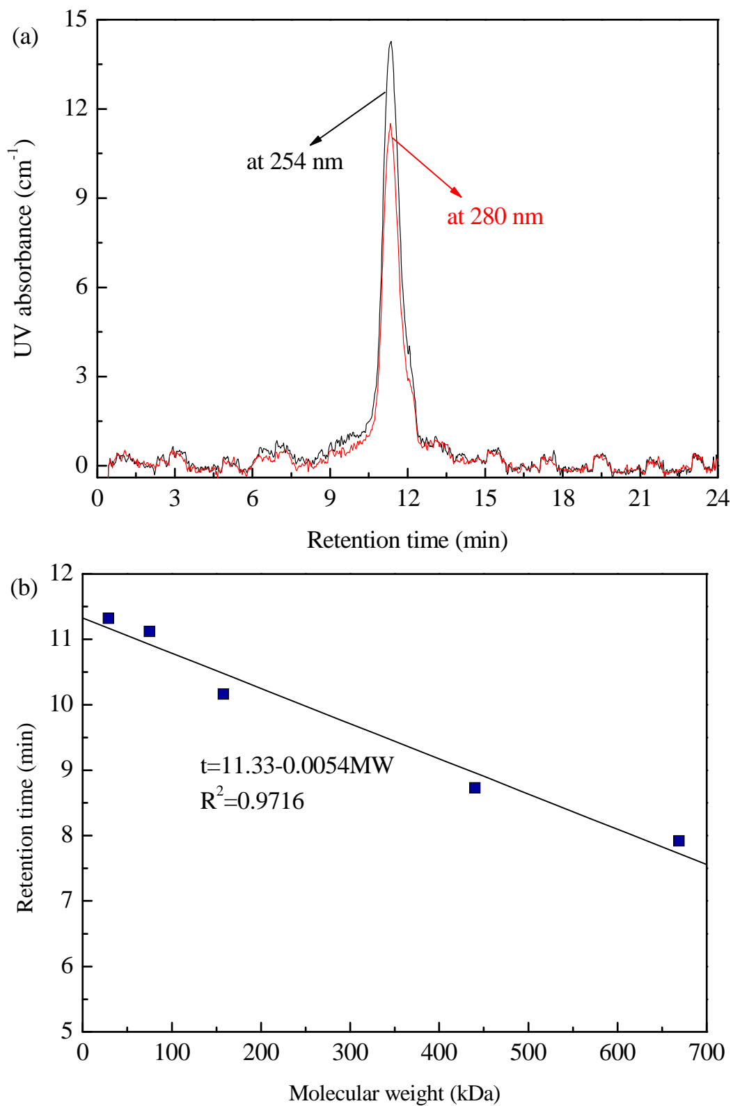
Fig. A. Determination of molecule weight by HPSEC: (a) high performance size exclusion chromatogram of HA used in this study; (b) retention time as a function of MW.
