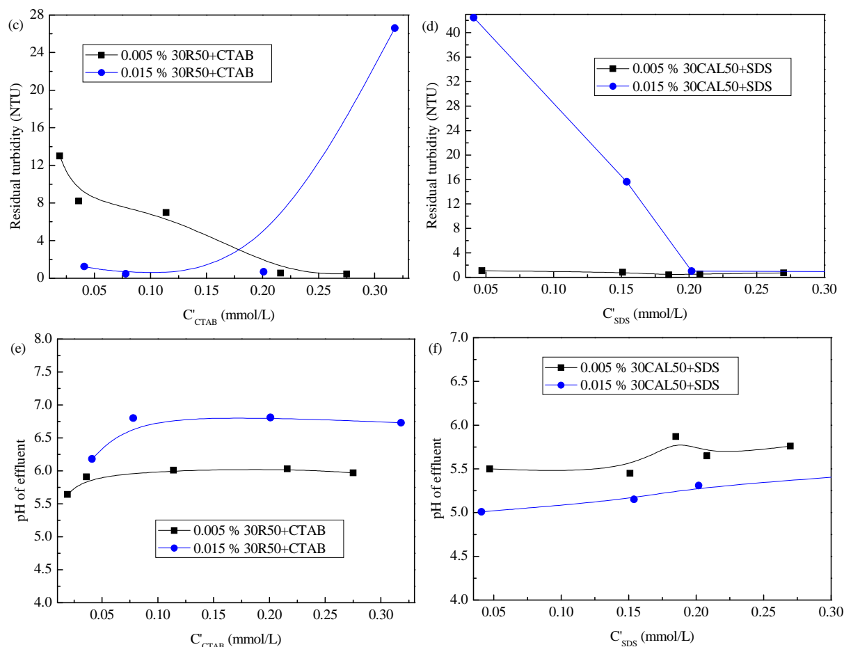
Fig. 4.30. Effect of initial SNP volume concentration on the performance of CGA-flotation: (a), (b) removal efficiency and zeta potential of 30R50 and 30CAL50, respectively; (c), (d) residual turbidity of 30R50 and 30CAL50, respectively; (e), (f) pH of 30R50 and 30CAL50, respectively.
