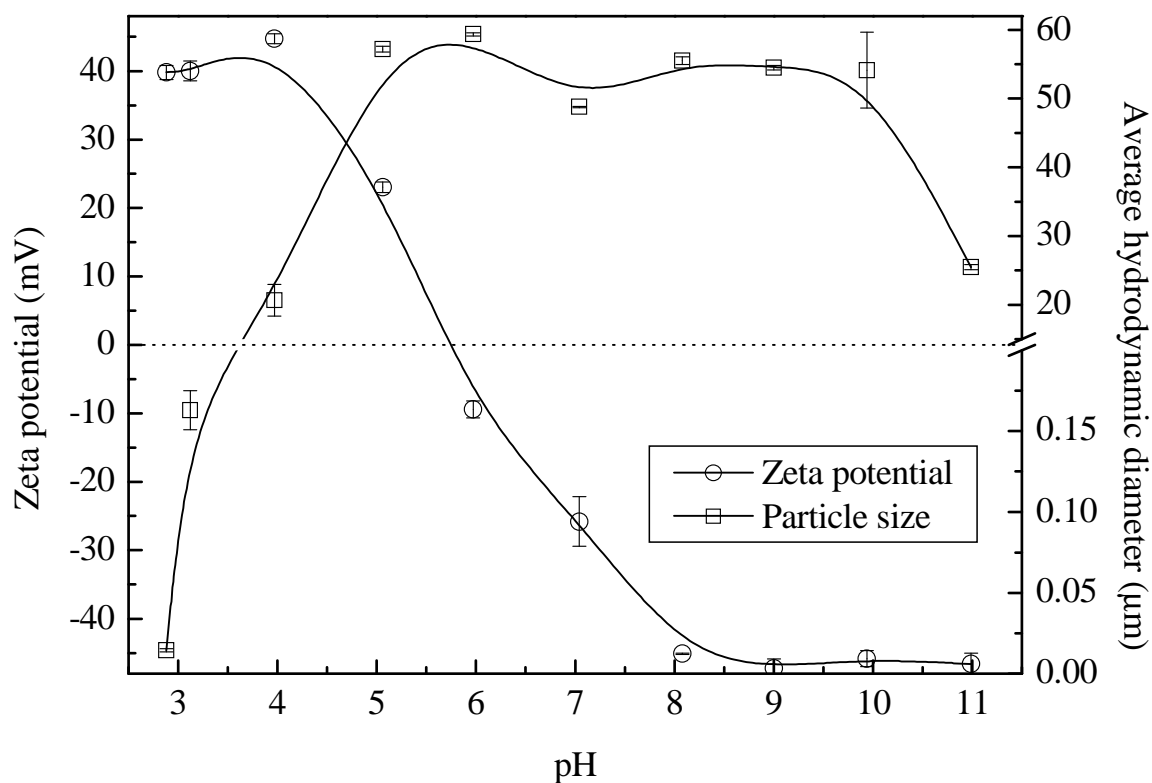
Fig. 2.4. Zeta potential and particle size varying with pH values of TNP suspension.
