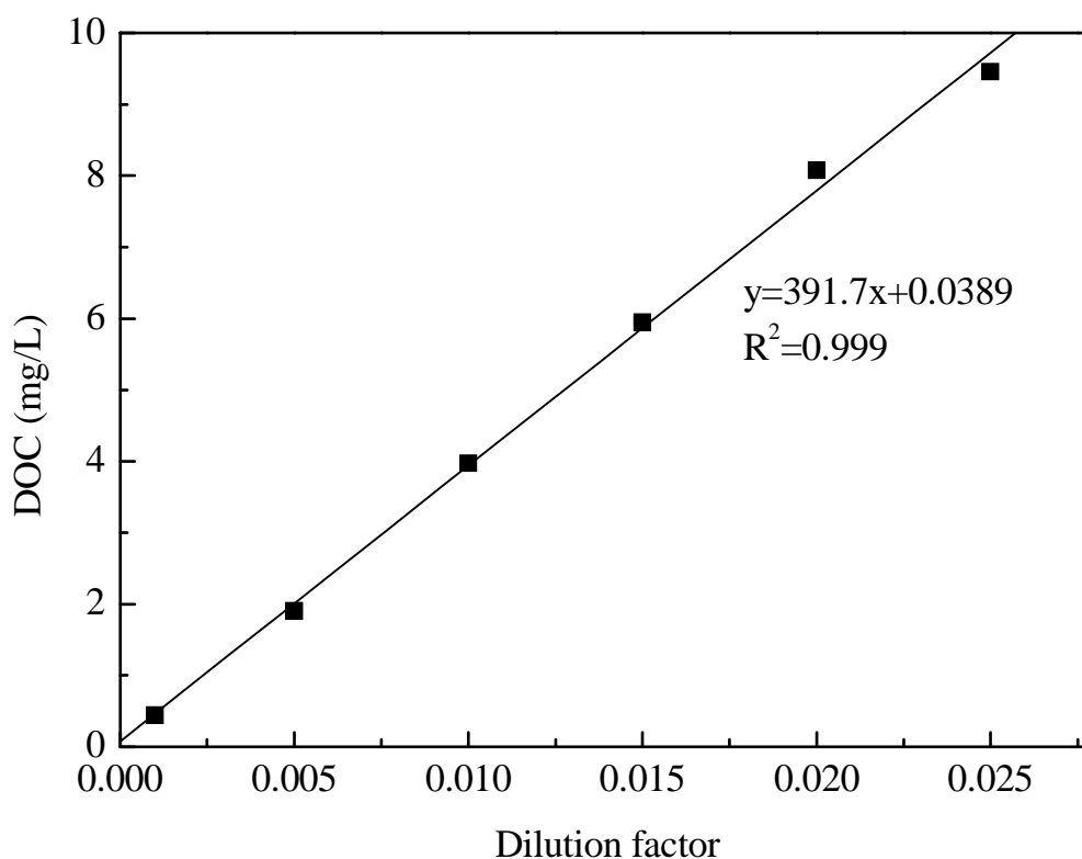
Fig. 2.7. DOC as a function of HA concentration.
