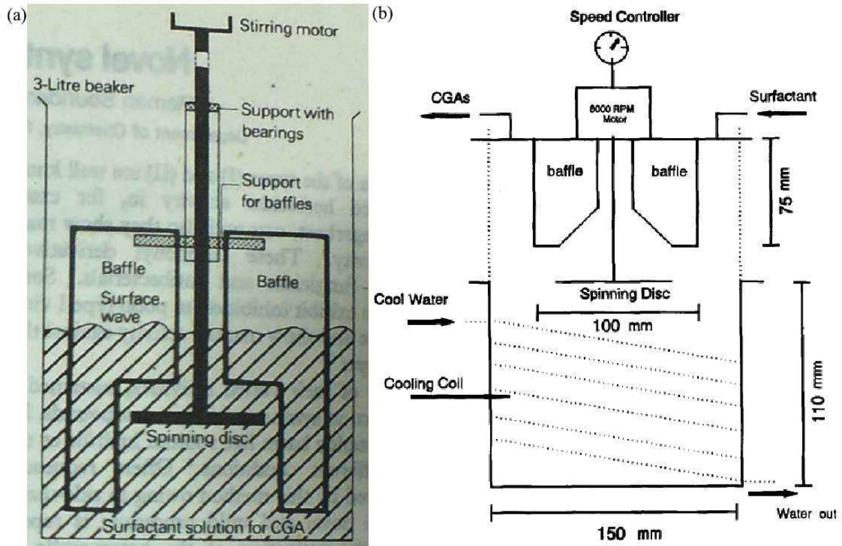
Fig. 1.9. Typical CGA generators: (a) Spinning disc generator by F. Sebba (1985); (b) generator designed by Chaphalkar et al. (1993; 1994).
