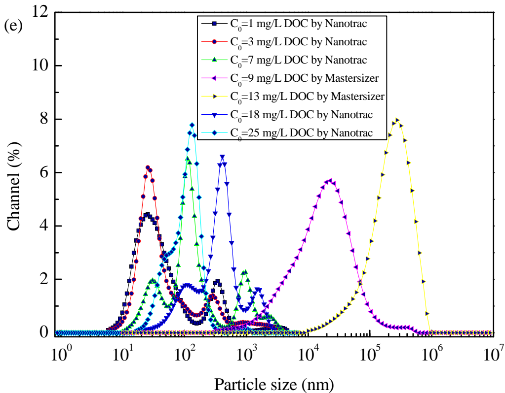
Fig. 3.10. Particle size measurement of TNP-HA aggregates after adsorption-aggregation: (a) variation of particle size with initial HA concentration; PSD patterns at different pH values of HA stock solution (b) \text{pH}_{\text{HA}}=4.0 , (c) \text{pH}_{\text{HA}}=6.3 , (d) \text{pH}_{\text{HA}}=9.1 , (e) \text{pH}_{\text{HA}}=12.9 .
