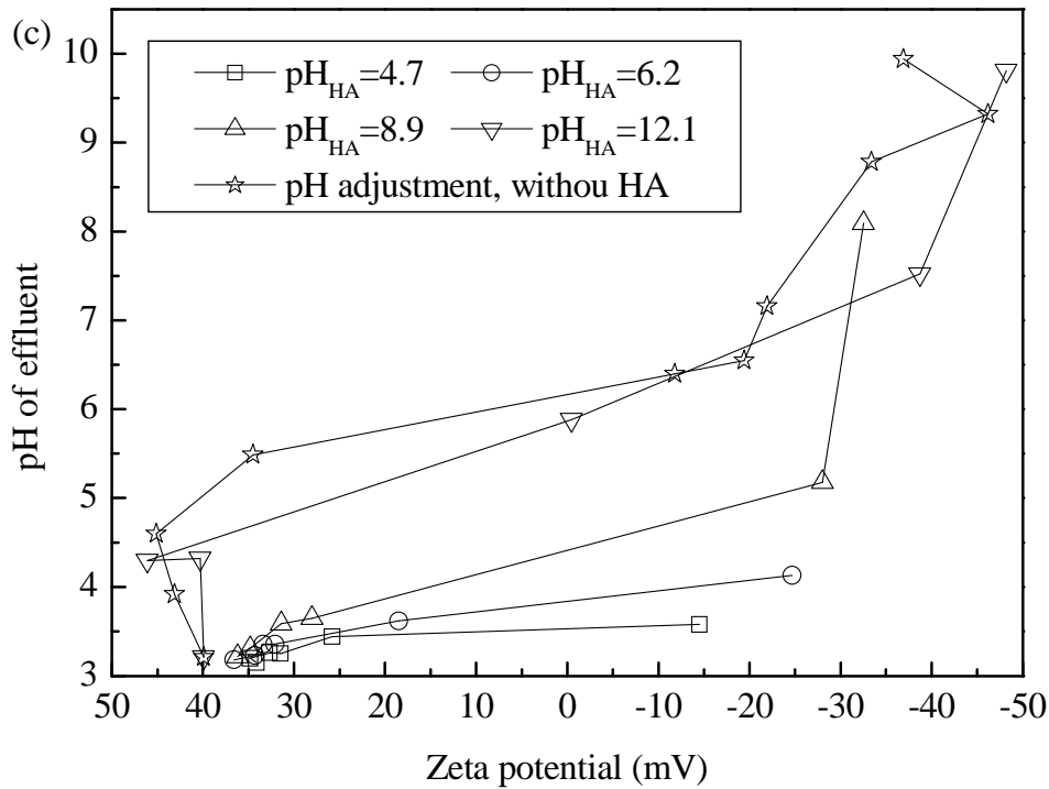
Fig. 3.22. Relationship between DAF performance and zeta potential of flotation suspension: (a) TNP removal efficiency, (b) HA removal, and (c) pH of effluent.
