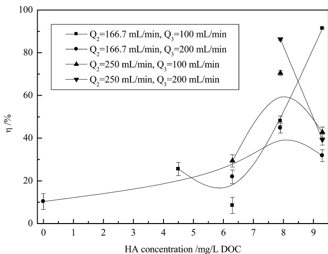
Fig. 12. Effect of HA concentration on TNP removal efficiency. (Negative efficiencies are omitted.).
