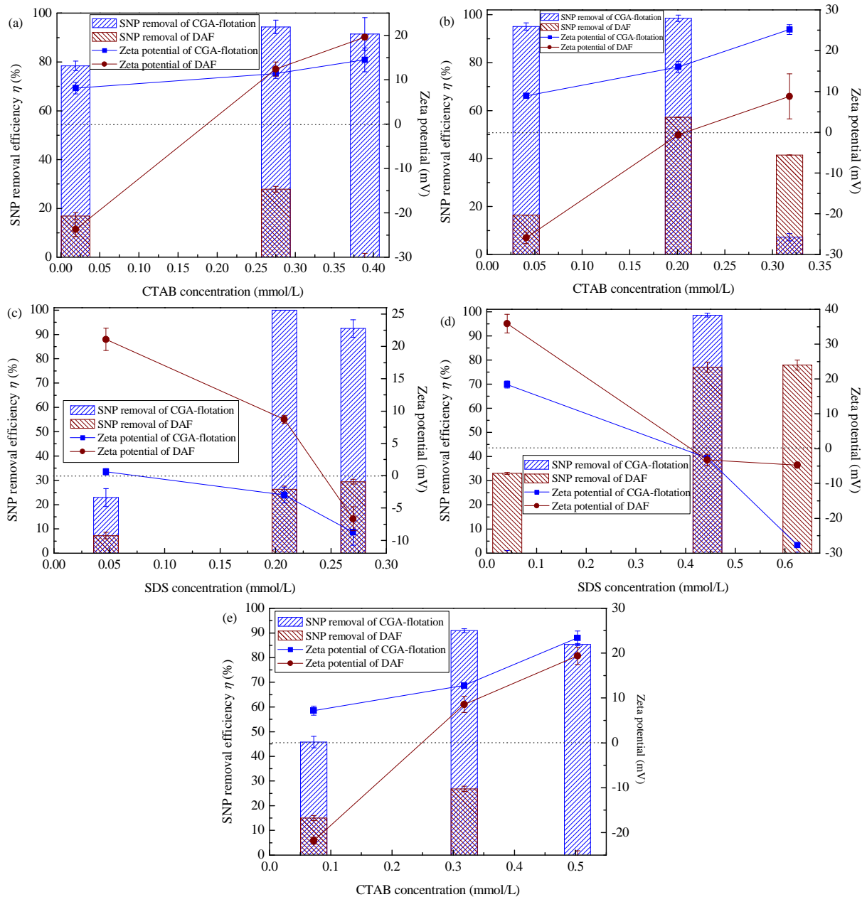
Fig. 4.31. Comparison of SNP removal efficiency and zeta potential between CGA involved flotation and surfactant assisted DAF: (a) 30R50 0.005 %; (b) 30R15 0.015 % (c) 30CAL50 0.005 %; (d) 30CAL50 0.015 %; (e) 30R25 0.015 %.
