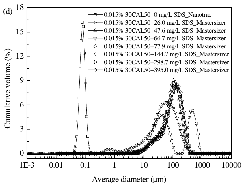
Fig. 4.25. Particle size measurement of SNP-surfactant aggregates after adsorption-aggregation: (a) variation of particle size with initial surfactant concentration; (b), (c) and (d) PSD patterns of 0.015 vol.% 30R50+CTAB, 0.015 vol.% 30R25+CTAB; and 0.015 vol.% 30CAL50+SDS, respectively.
