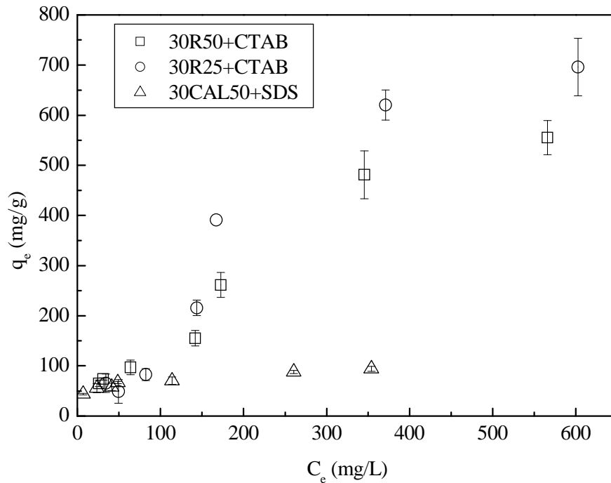
Fig. 4.23. Experimental results of SNP-surfactant adsorption-aggregation.
