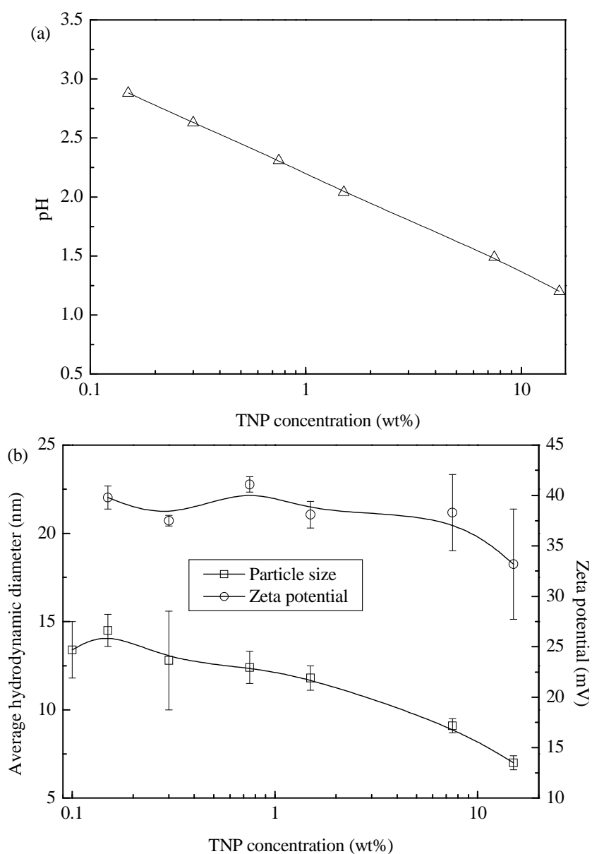
Fig. 2.3. Properties of TNP suspension varying with different TNP concentrations: (a) pH; (b) particle size and zeta potential.
