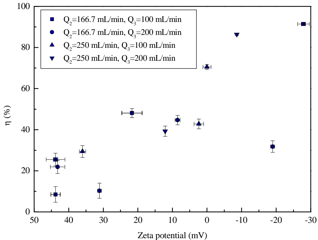
Fig. 3.16. Relationship between TNP removal efficiency and zeta potential of the flotation suspension. (Negative efficiencies are omitted.)
