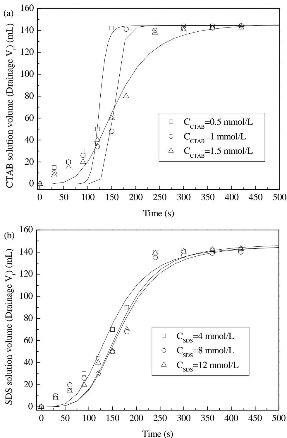
Fig. 4.7. Comparison between experimental data (scatters) and fitting drainage curves (curve) at different surfactant concentrations: (a) CTAB-CGAs, (b) SDS-CGAs.
