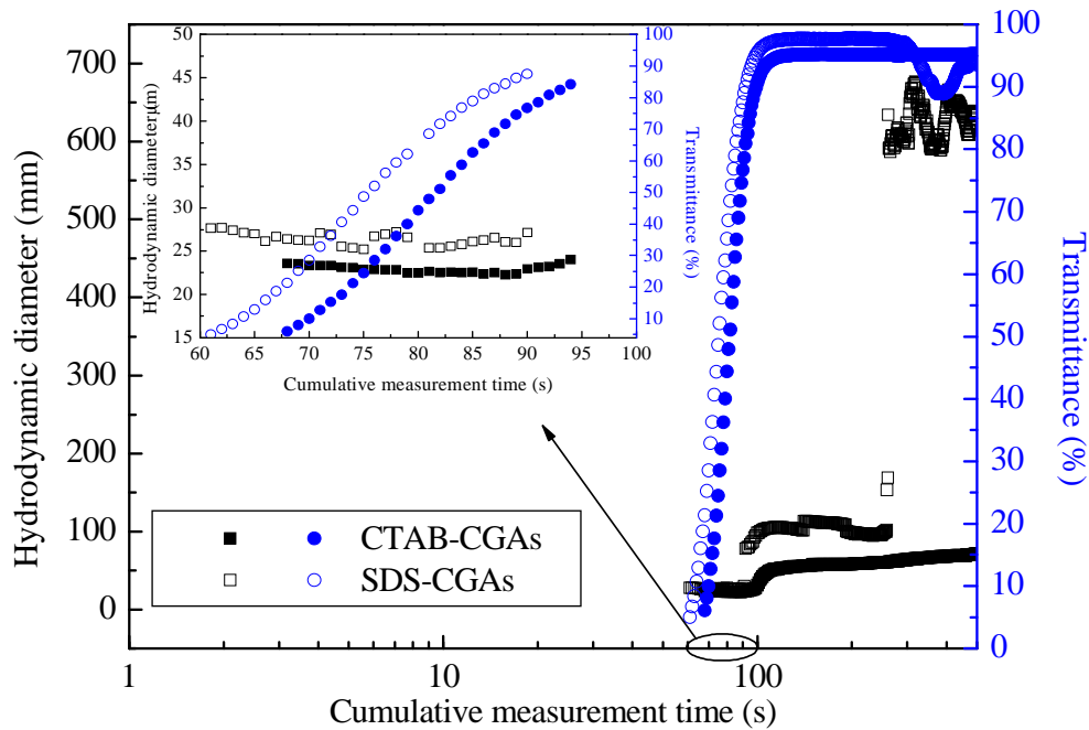
Fig. 4.14. Spraytec measurement at 30 s after the measurement began.
