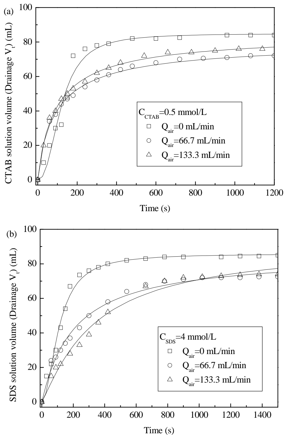
Fig. 4.8. Comparison between experimental data (scatters) and fitting drainage curves (curve) at different air flow rates: (a) CTAB-CGAs, (b) SDS-CGAs.
