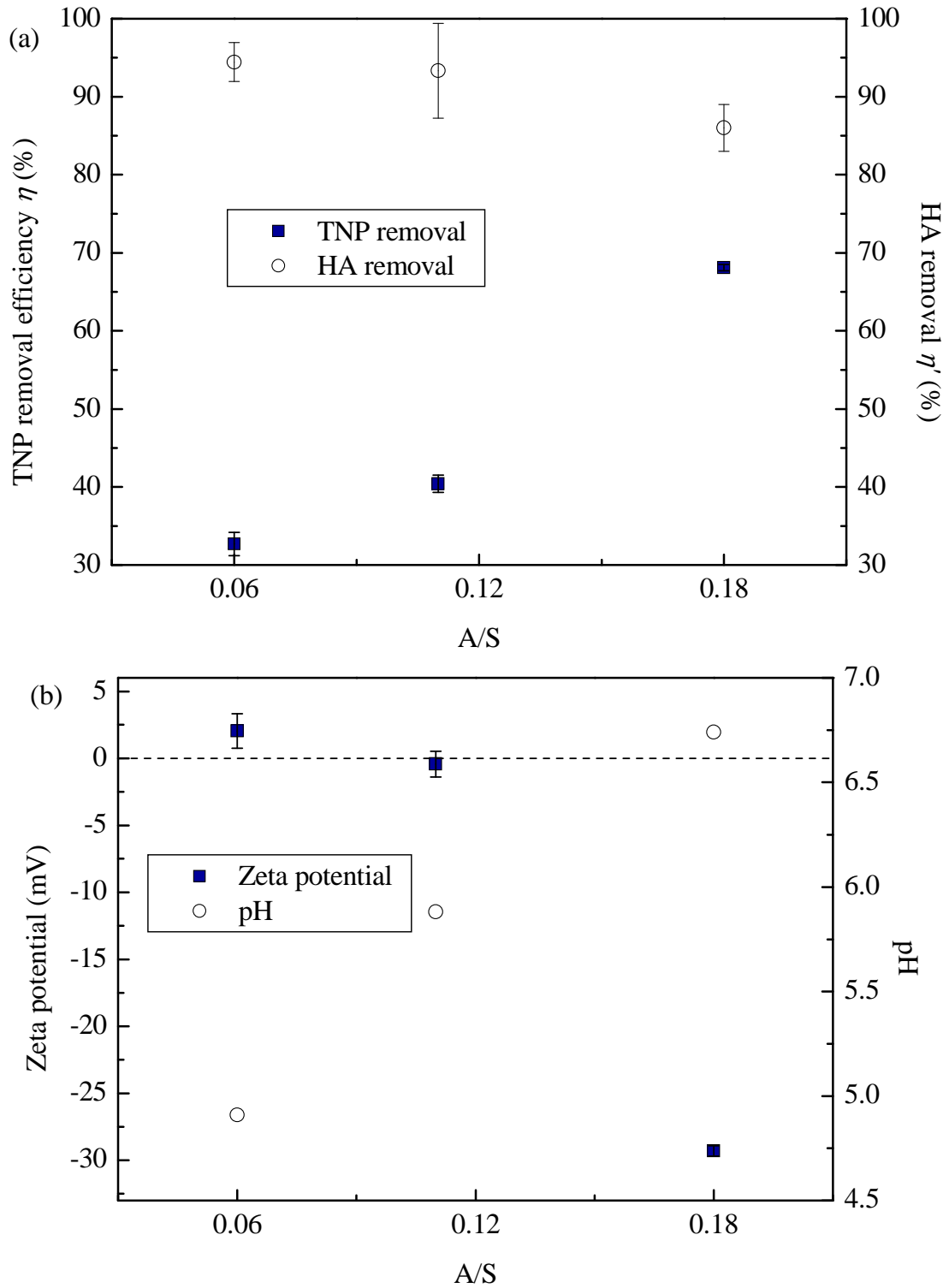
Fig. 3.20. Comparison of flotation performances at different A/S ratios: (a) TNP and HA removal, (b) Zeta potential and pH of effluent.
