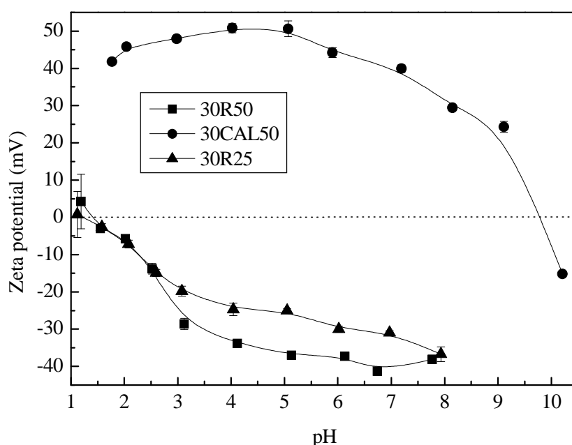
Fig. 2.14. Zeta potential of suspensions varying with pH value at the SNP concentration of 0.15 vol.%.
