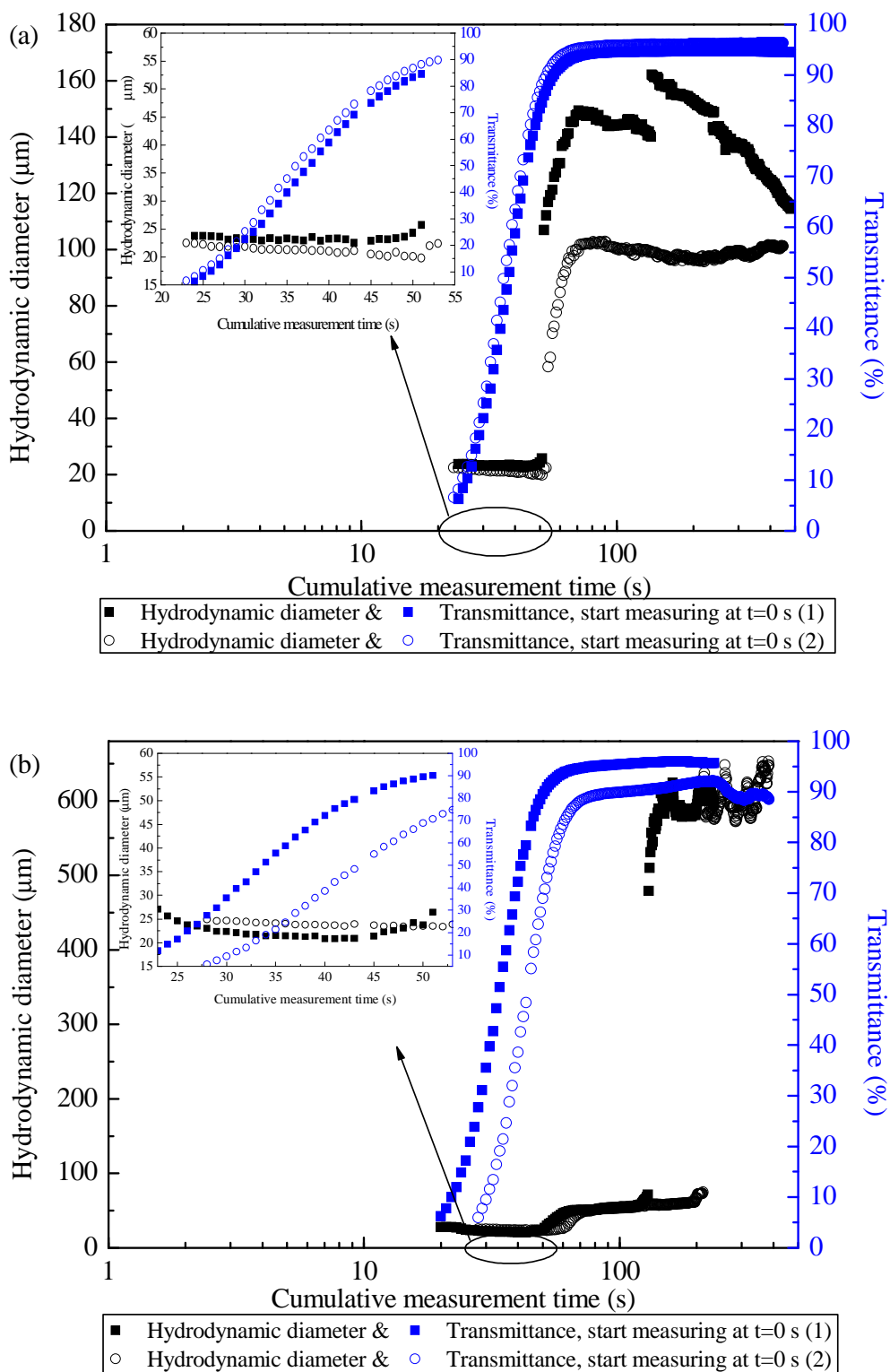
Fig. 4.12. Spraytec measurement immediately after the measurement began: (a) CTAB-CGAs; (b) SDS-CGAs. (Experiments were replicated.)
