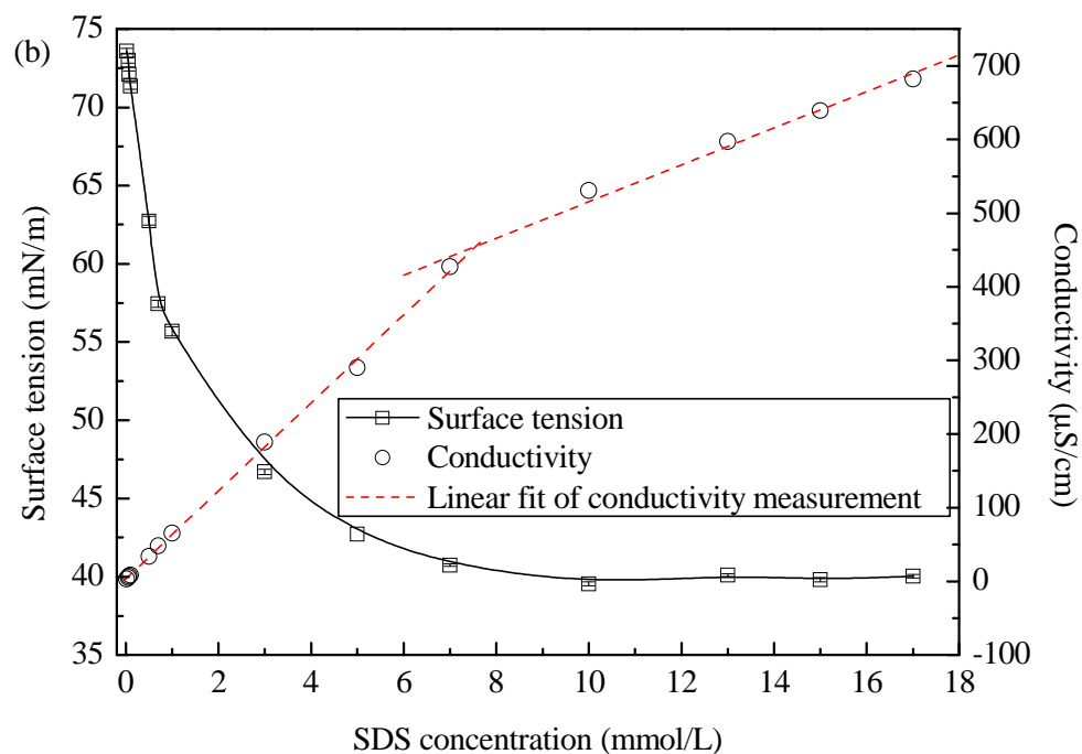
Fig. 2.19. Determination of CMCs by measuring surface tension and conductivity: (a) CTAB; (b) SDS.
