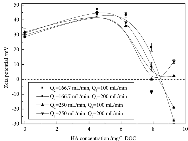
Fig. 13. Effect of HA concentration on Zeta potential of treated TNP suspensions.
