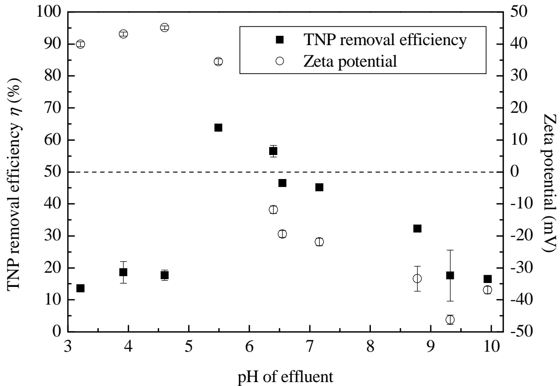
Fig. 3.17. TNP removal efficiency and zeta potential varying with pH of effluent.
