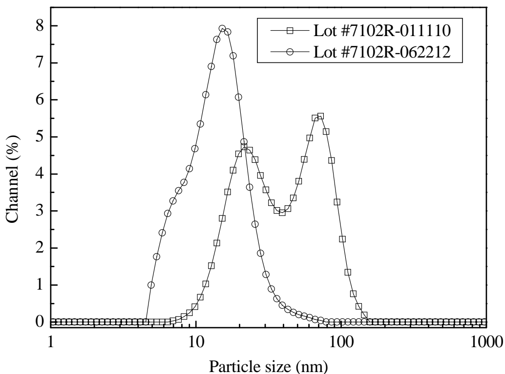
Fig. 2.1. Particle size distributions of two TNP suspensions (Lot #1 and Lot #2).
