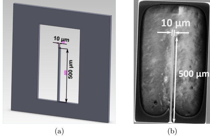
Figure 5.6: Silicon microparts used for the experiments.
