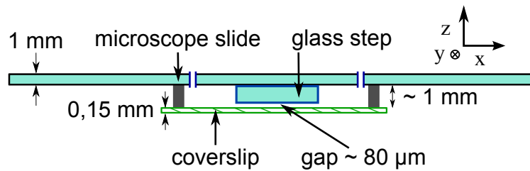
Figure 2.2: Schematic representation of the cell used to trap particles dispersed in water (view from the side). The central part has a smaller gap than the rest of the cell.
