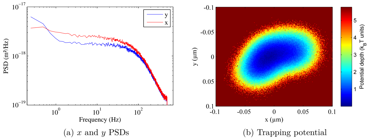
Figure 5.16: a) Measured Power Spectral Densities of x and y -displacement of the trapped particle in the fluid flow. b) Trapping potential estimated by the distribution of particle's positions.
