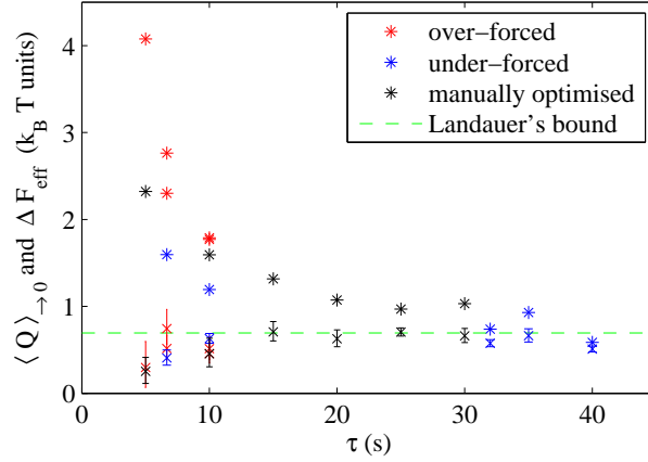
Figure 2.10: Mean dissipated heat (*) and effective free energy difference ( \times ) for several procedures, with fixed \tau and different values of f_{\text{max}} . The red points have a force too high, and a P_{S\text{force}} \geq 99\% . The blue points have a force too low and 91\% \leq P_{S\text{force}} < 95\% (except the last point which has P_{S\text{force}} \approx 80\% ). The black points are considered to be optimised and have 95\% \leq P_{S\text{force}} < 99\% .
