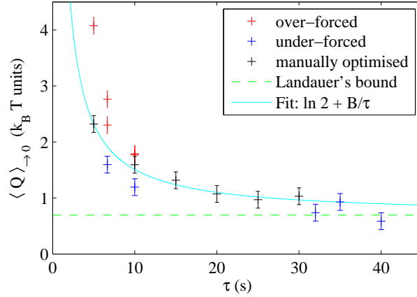
Figure 2.8: Mean dissipated heat for several procedures, with fixed \tau and different values of f_{\text{max}} . The red points have a force too high, and a P_{S \text{ force}} \geq 99 \% . The blue points have a force too low and 91 \% \leq P_{S \text{ force}} < 95 \% (except the last point which has P_{S \text{ force}} \approx 80 \% ). The black points are considered to be optimised and have 95 \% \leq P_{S \text{ force}} < 99 \% . The error bars are \pm 0.15 k_B T estimated from the reproducibility of measurement with same parameters. The fit \langle Q \rangle_{\rightarrow 0} = \ln 2 + B/\tau is done only by considering the optimised procedures.
