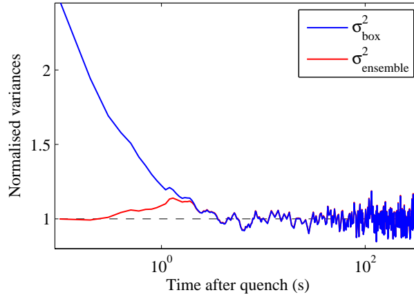
Figure 3.15: Ensemble and boxed variances computed for a \delta t = 1 s and normalised by the equilibrium value k_{\text{B}}T/k . The boxed variance clearly shows an anomalous increase at small times after the quench, which is the effect reported in previous works.
