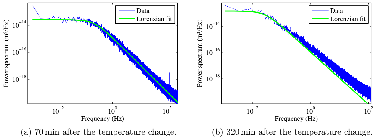
Figure 3.9: Power Spectral Density of the position of one particle trapped in gelatin solution kept at 28.5 °C (after being melt at 37 °C for 30 min). The PSD is estimated over a time window of 1 h. Shortly after switching the temperature the gelatin solution is still a Newtonian fluid and the PSD is Lorentzian. After some time, visco-elastic effects appear and the PSD is no longer Lorentzian.
