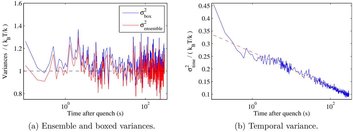
Figure 3.14: Different variances computed for \delta t = 0.1 s and normalised by the equilibrium value k_{\text{B}}T/k . The ensemble and boxed values are nearly equal and seem to be close to the equilibrium value at any time after the quench. Whereas the temporal value is clearly below the equilibrium value and decreases logarithmically with time after the quench.
