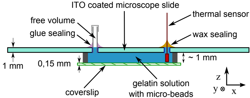
Figure 3.4: Schematic representation of the cell used to trap particles in gelatin solution (view from the side). The microscope slide is ITO-coated, which enables us to heat the cell by sending an electrical current through the glass surface.
