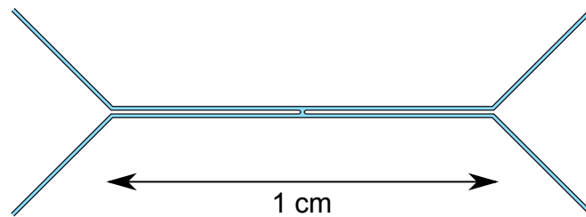
Figure 5.3: Example of pattern that needs to be engraved in a flat material to create the mould used to create microfluidic cells. The depth of engravement must be of \sim 100\mu\text{m} and the design needs to have a good resolution at the micro-scale.
