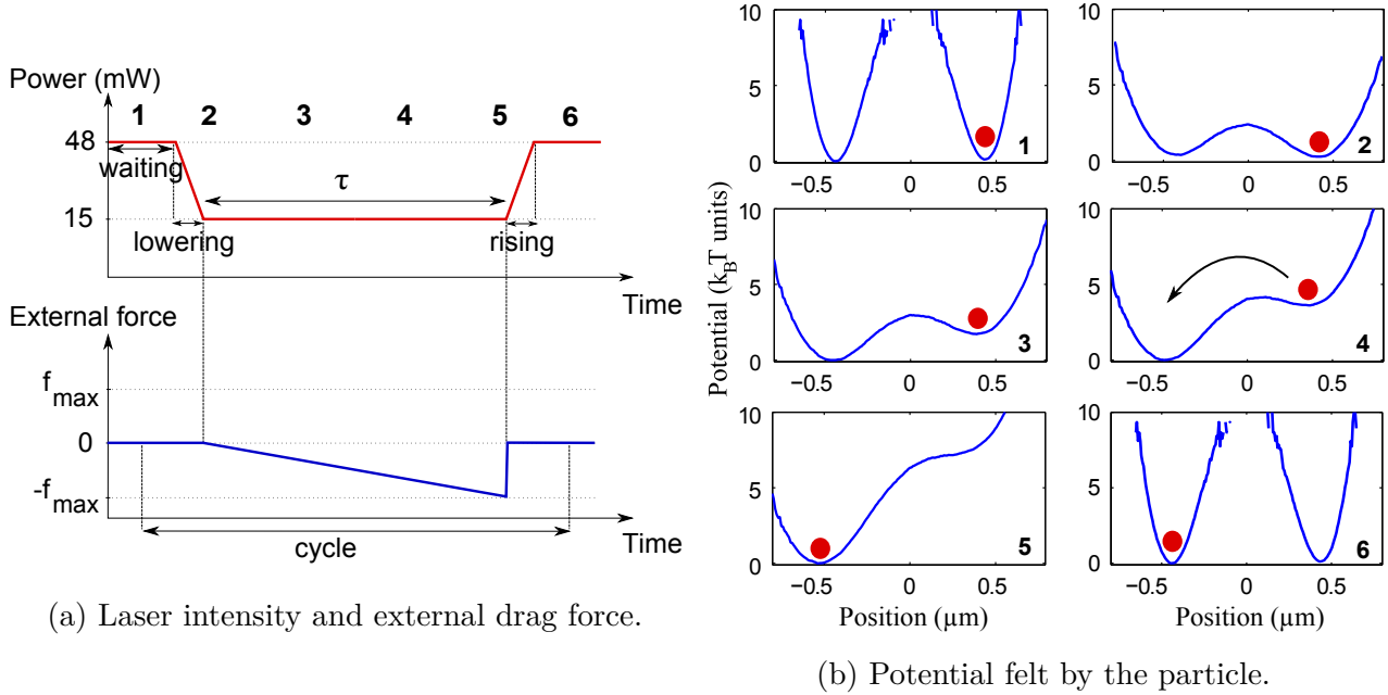
Figure 2.5: Schematic representation of the erasure procedure. The potential felt by the trapped particle is represented at different stages of the procedure (1 to 6). For 1 and 2 the potential U_0(x, I) is measured. For 3 to 5 the potential is constructed from U_0(x, I_{\text{low}}) knowing the value of the applied drag force.
