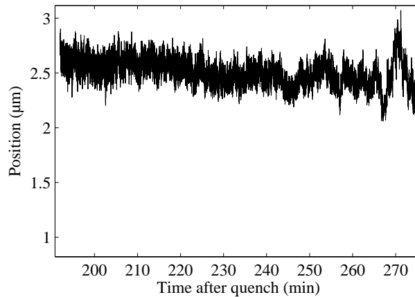
Figure 3.8: Evolution of the position of one trapped particle, in gelatin solution kept at 28.3 °C (after being melt at 37 °C for 20 min). At the end of the trajectory, gelation occurs and the particle is moved away from the optical trap.
