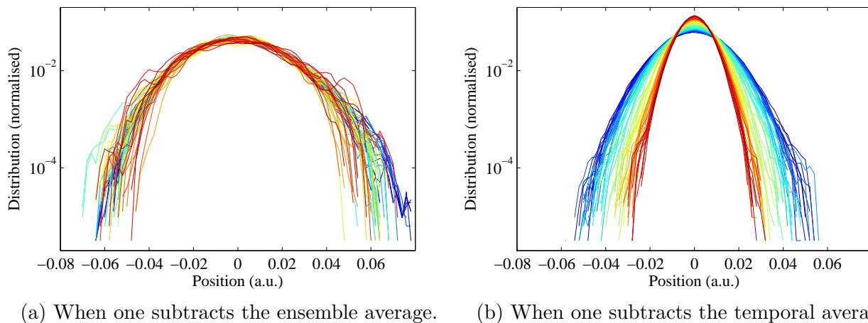
Figure 3.16: Evolution of the Probability Distribution Function of the position fluctuation \delta x depending on the definition taken for the subtracted average. The PDFs are computed on a time-window \delta t = 0.5 s for different times after the quench, going from t = 0 s (blue curves) to t = 540 s (red curves).
