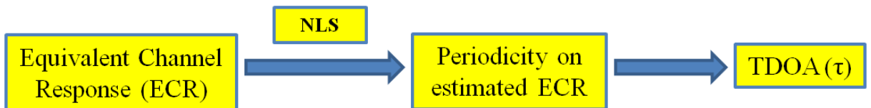
Figure 3.14: TDOA estimation algorithm using NLS applied on ECR
