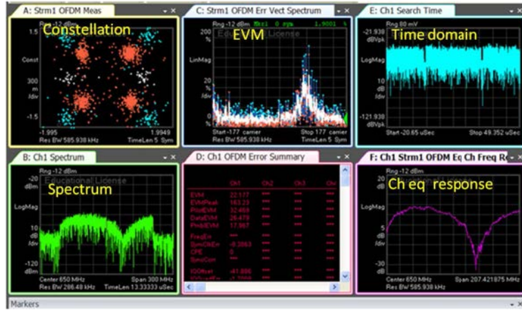
Figure 4.11: An example of measurement results using Vubiq and DSO with open waveguides, QAM OFDM, EVM= 24%, baseline= 18 cm.
