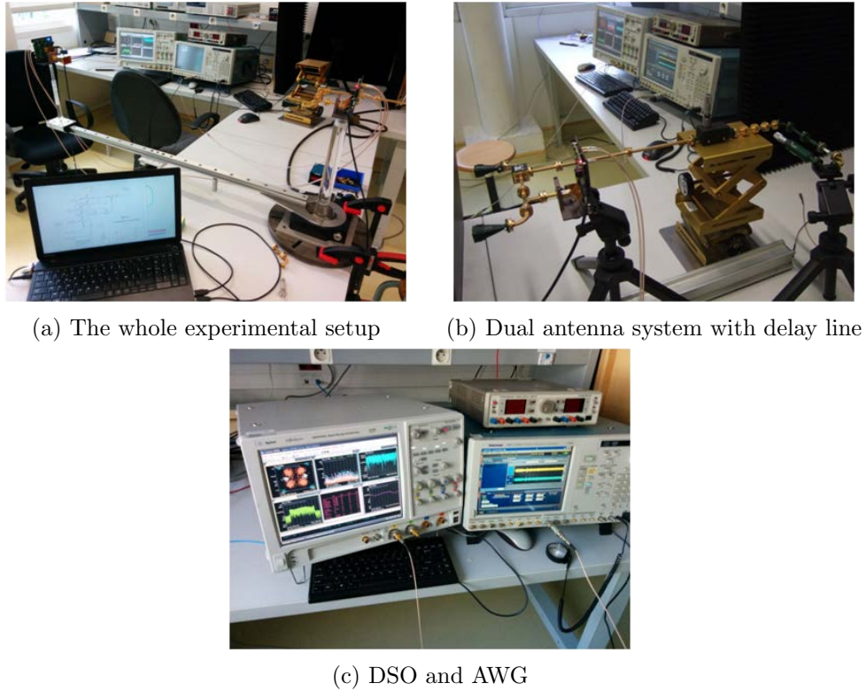
Figure 4.10: Measurements using Vubiq and DSO with open waveguides
