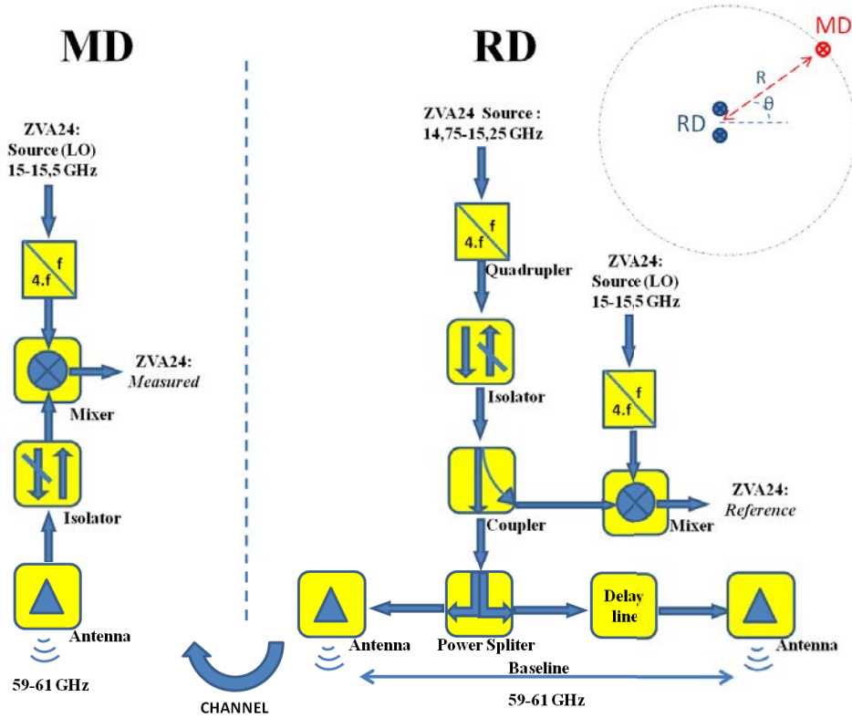
Figure 4.1: VNA (ZVA24) Measurement configuration schematic.
