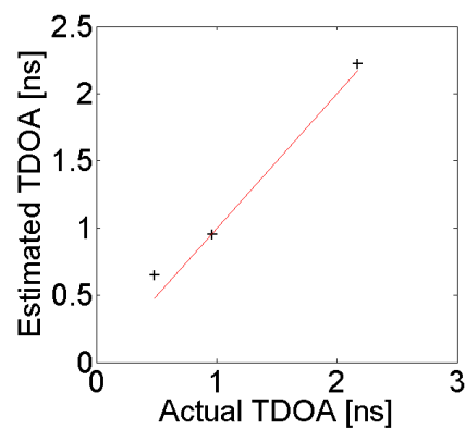
Figure 4.22: TDOA Measurements results using multi-band approach with base-band signals.
