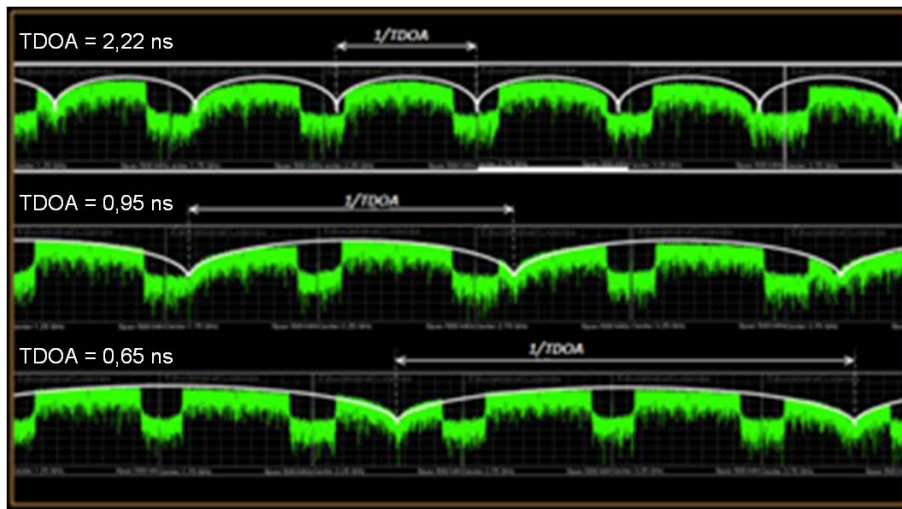
Figure 4.21: Concatenated multi-band received signals in three different cases.
