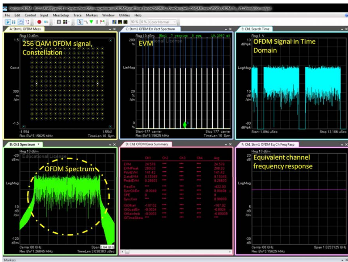
Figure 4.9: General display of the received OFDM signal using digital storage oscilloscope (DSO) with vectorial signal analyzer (VSA).
