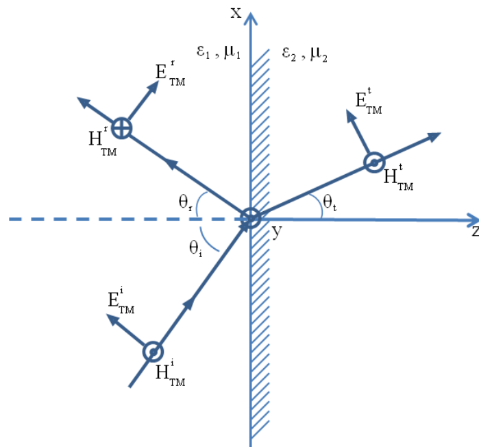
Figure 2.3: TM mode.
