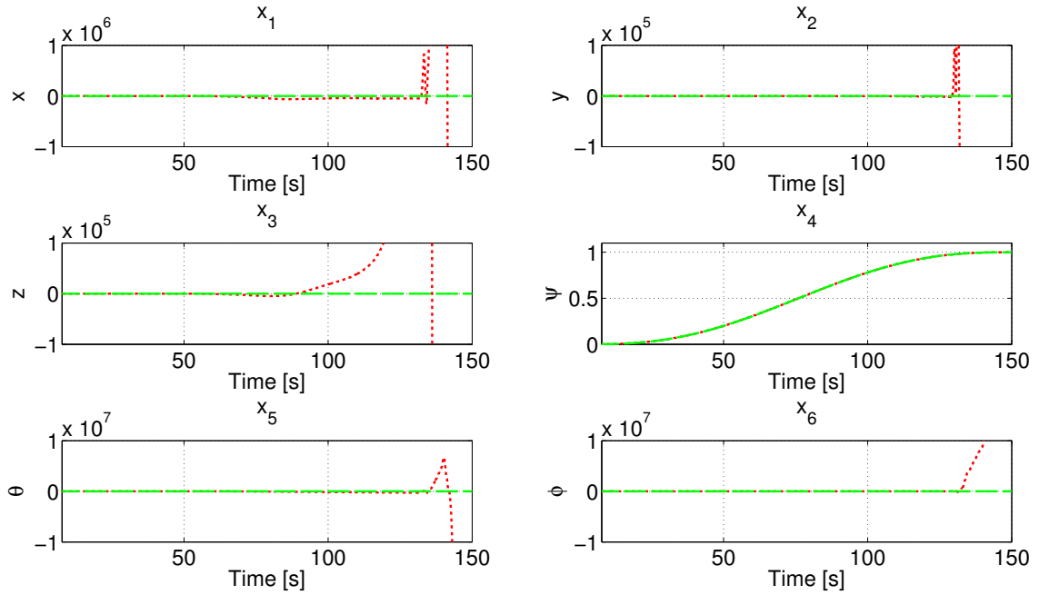
Figure 3.12: Fault affecting x_5 . No-reconfiguration ( \cdots ). Nominal ( --- ).
