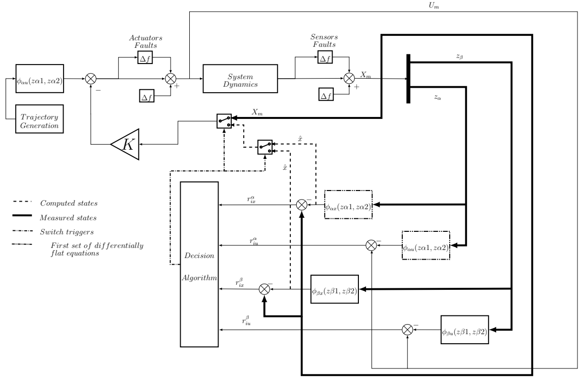
Figure 2.4: Reconfiguration diagram
