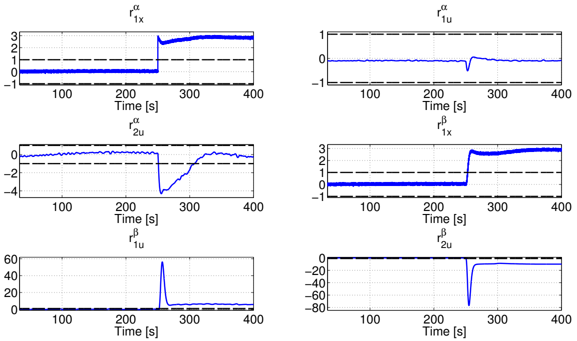
Figure 3.33: Additive fault measure x_2 normalized ( z_\alpha and z_\beta set)
