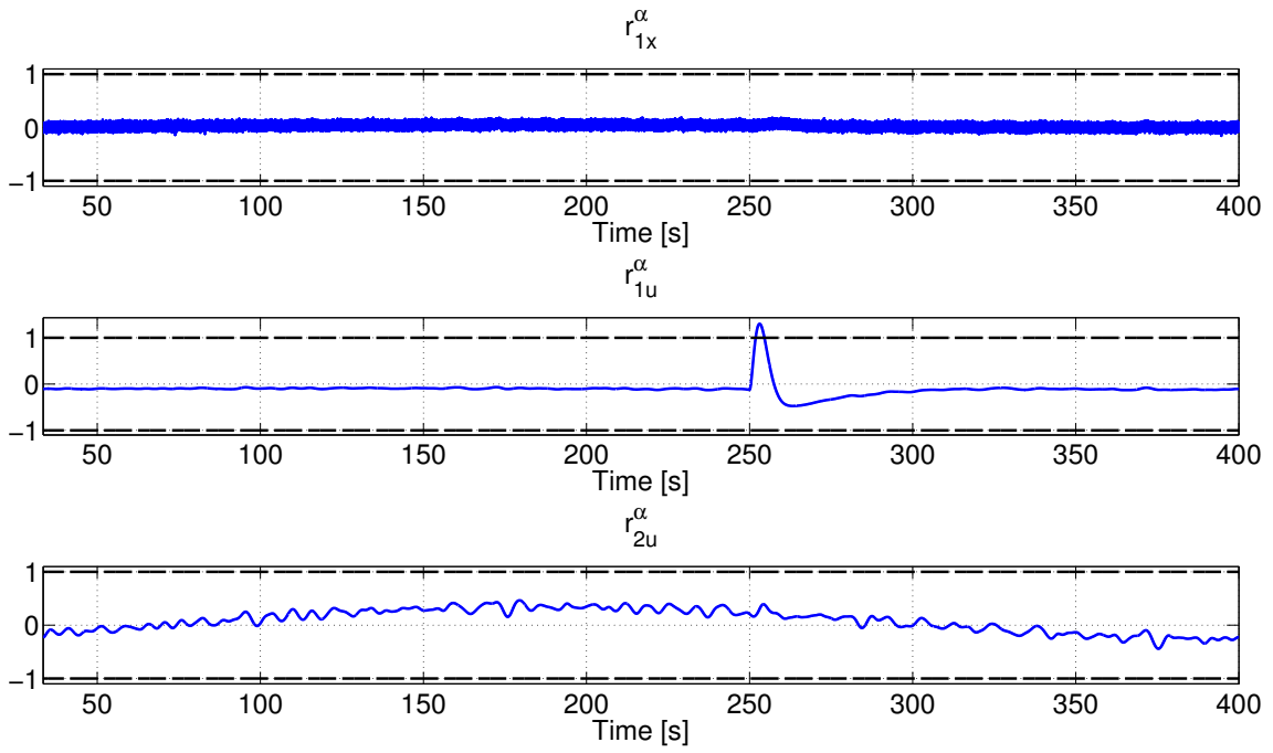
Figure 3.19: Additive fault in flow pump u_1 normalized ( z_\alpha set)
