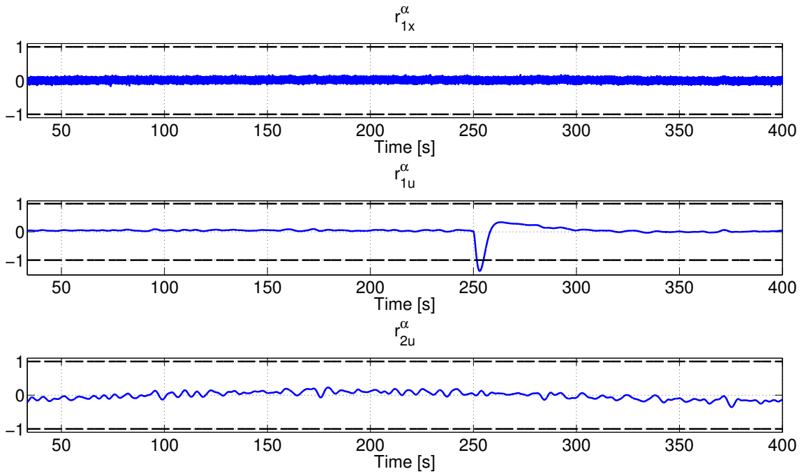
Figure 3.21: Multiplicative fault in flow pump u_1 normalized ( z_\alpha set)
