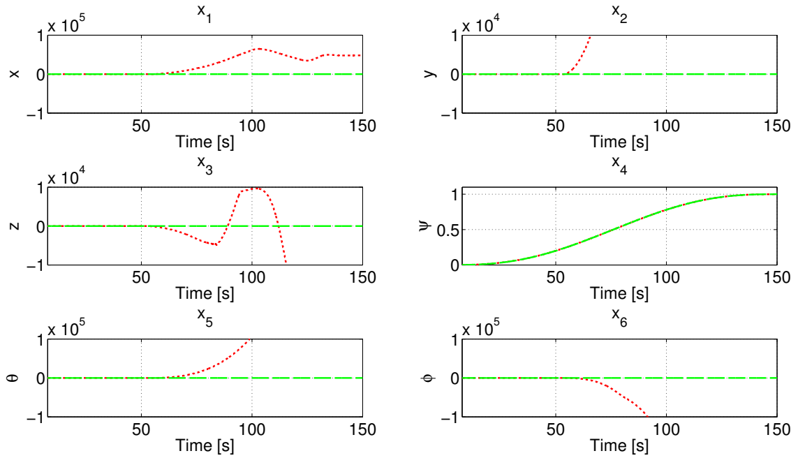
Figure 3.13: Fault x_6 . No-reconfiguration ( \cdots ). Nominal ( --- ).
