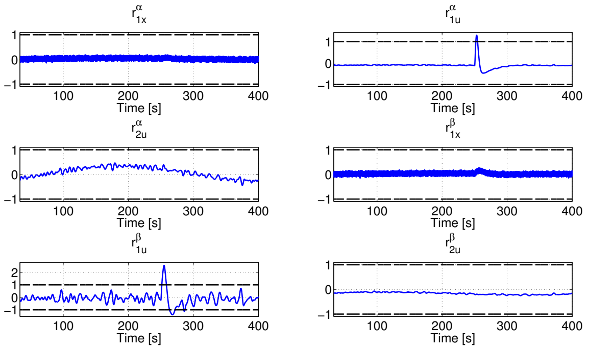
Figure 3.27: Additive fault in flow pump u_1 normalized ( z_\alpha and z_\beta set)
