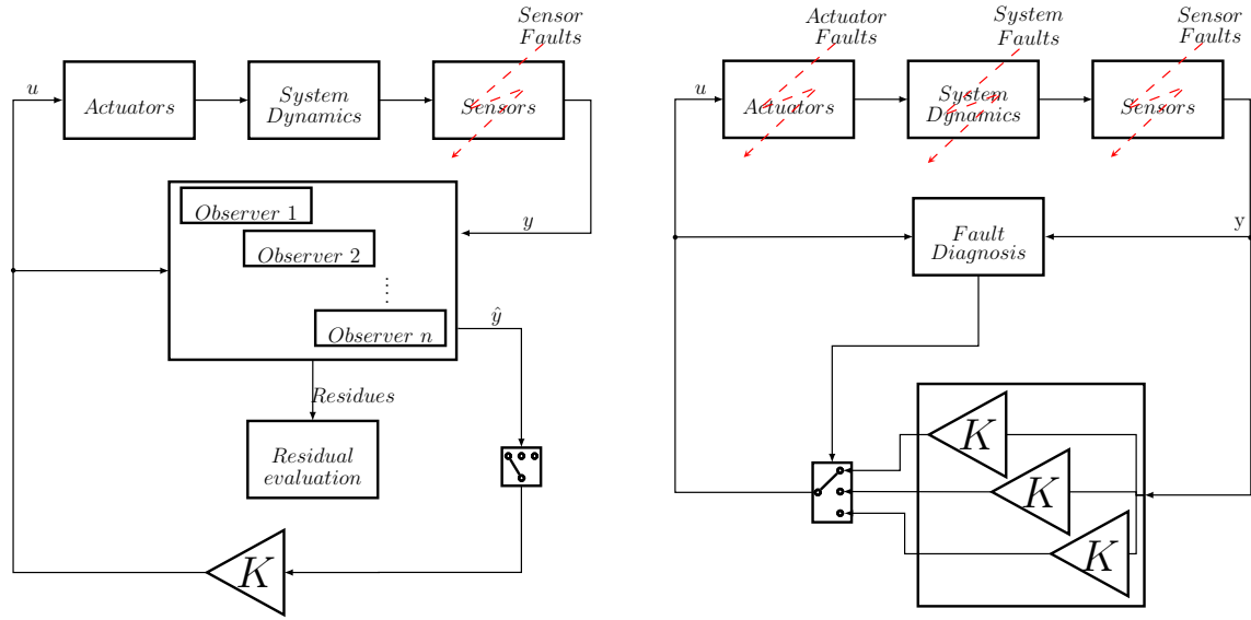
Figure 1.10: Banks of observers and controllers [52]
