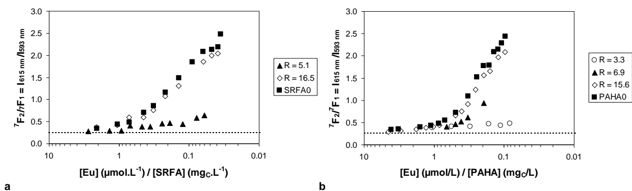
Figure 5-11. Evolution of the {}^7F_2/{}^7F_1 ratios as a function of [Eu(III)]/TOC ( \mu\text{mol}_{Eu} \text{L}^{-1}/\text{mg}_C \text{L}^{-1} ) for the Suwannee River fulvic acid (SRFA, a) and purified Aldrich HA (PAHA, b), for different values of R_{HS} , pH 4, I = 0.1 \text{ mol kg}^{-1} : the dashed and dotted are the {}^7F_2/{}^7F_1 ratios of Eu^{3+} at pH 4 – from [15] © 2008 American Chemical Society].
