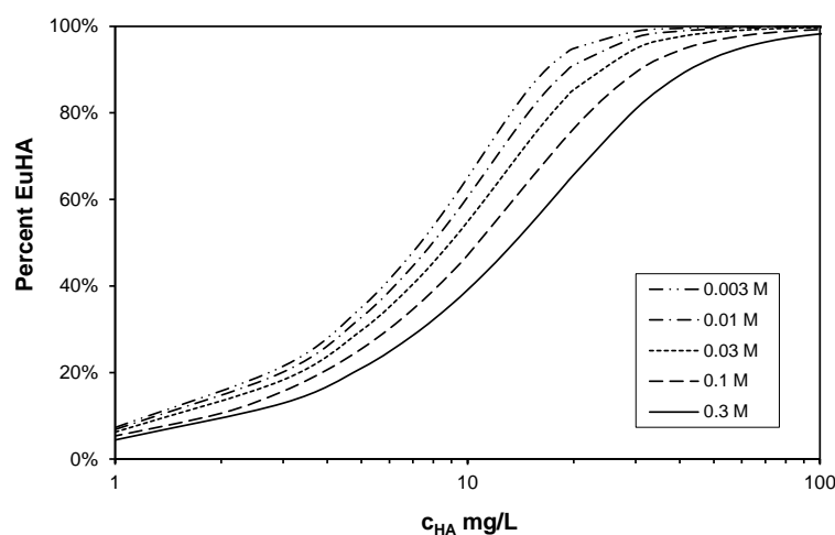
Figure 4-17. Influence of ionic strength on the proportion of 10 \mu\text{mol}_{Eu} L -1 fixed to the generic humic acid defined by MILNE et al. (2003) at pH 4.
