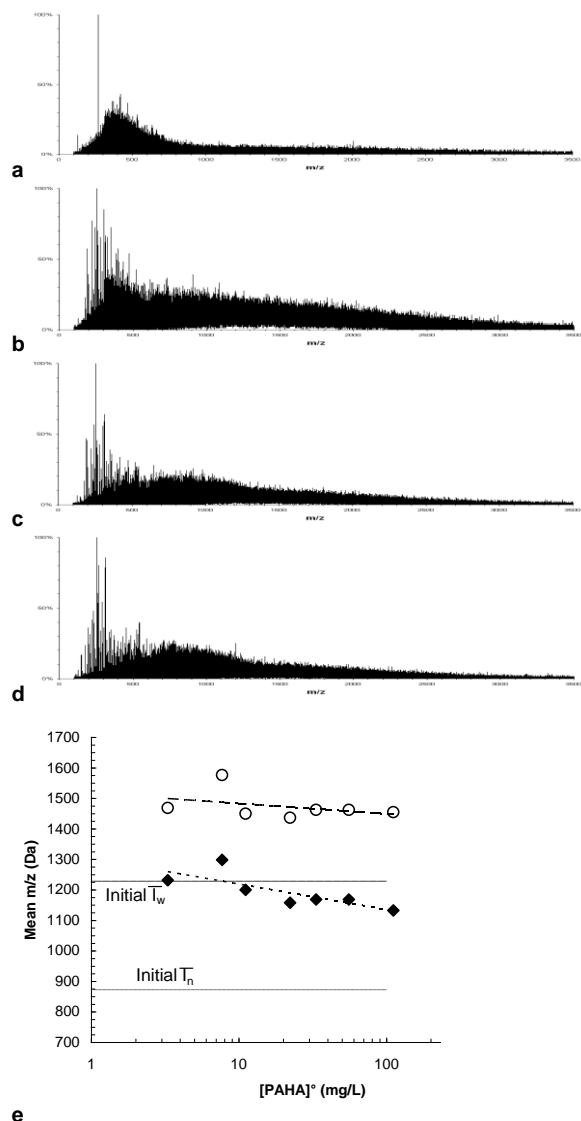
Figure 5-9. ESI Q-ToF Mass spectra of negative ions of purified Aldrich humic acid (PAHA) pH ≈ 7 (a) before adsorption: c(\text{HA}) = 11 \text{ mg L}^{-1} ; (b-d) in the supernatant experiment c(\alpha\text{-Fe}_2\text{O}_3) = 500 \text{ mg L}^{-1} , for different initial concentrations of PAHA: c(\text{HA}) = 33 \text{ mg L}^{-1} (b), 11 \text{ mg L}^{-1} (c), 3.3 \text{ mg L}^{-1} (d), and evolution of the number- and weight-averaged « molecular masses » – from [20] © 2006 American Chemical Society].
