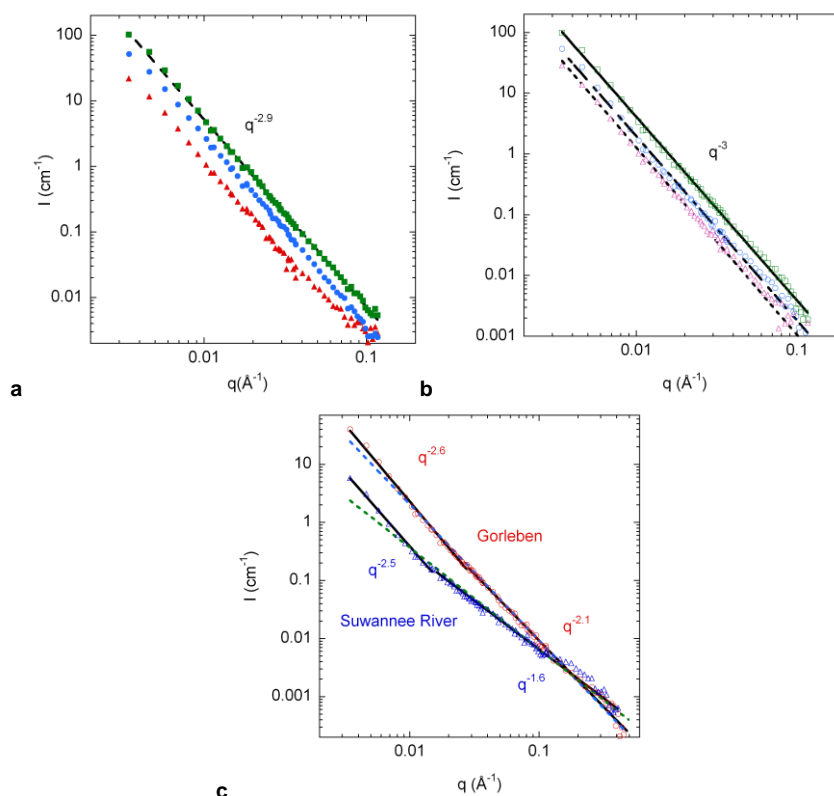
Figure 3-6. SANS patterns of PAHA (a), LHA (b), SRHA and Gorleben HA (c) in D 2 O, pD 5, I = 5 mM NaNO 3 . (a) and (b) for three different initial concentrations (squares) 8 g L -1 (circles) 3 g L -1 (triangles) 1 g L -1 , and (c) ( \Delta ) SRHA and ( \circ ) GoHyHA at 8 g L -1 [47]. Black lines are the fits obtained with the function A \cdot q^{-n} with two q range domain (i.e. a q_{\text{cut off}} ), the obtained value q^{-n} are indicated on the graph. The dashed lines are the fits obtained with only one q range domain for the function A \cdot q^{-n} .
