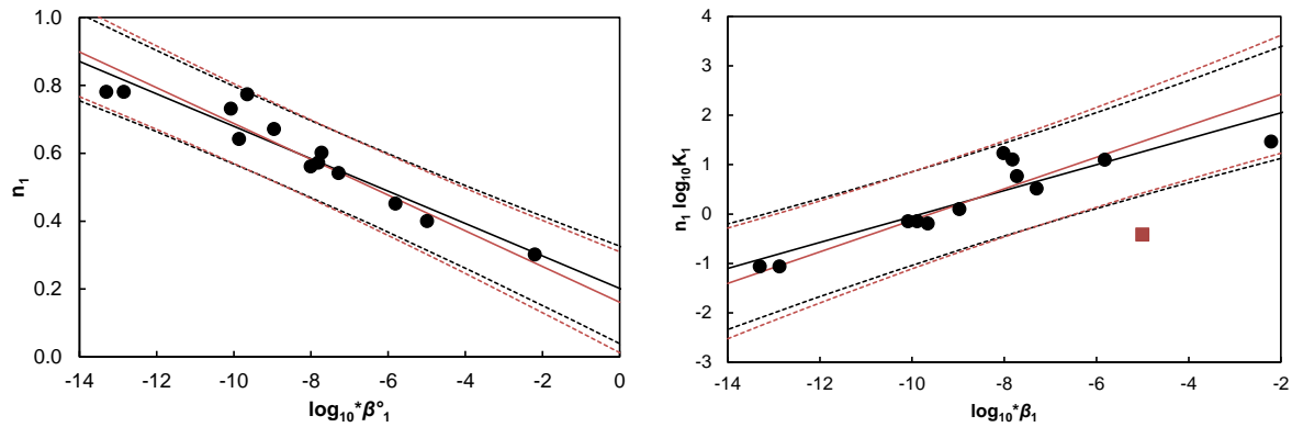
Figure 4-14. Correlation between n_{i,1} and \log_{10}^*\beta_1^o (a) and n_{i,1} \log_{10}\tilde{K}_{i,1} (b) for the case of humic acids, digitized from MILNE et al. (2003). The black lines are the original correlations, and the red lines are estimated in the document. Confidence hyperboles are 2\sigma .
