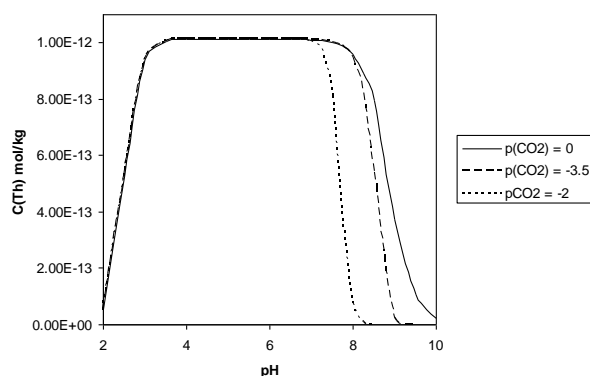
Figure 6-2. Influence CO 2 (g) partial pressure on the concentration of ThHA complex, [Th] = 10 -12 mol L -1 , C HA = 100 mg L -1 , and 5.4 mmol site L -1 , from Equation 4-8.
