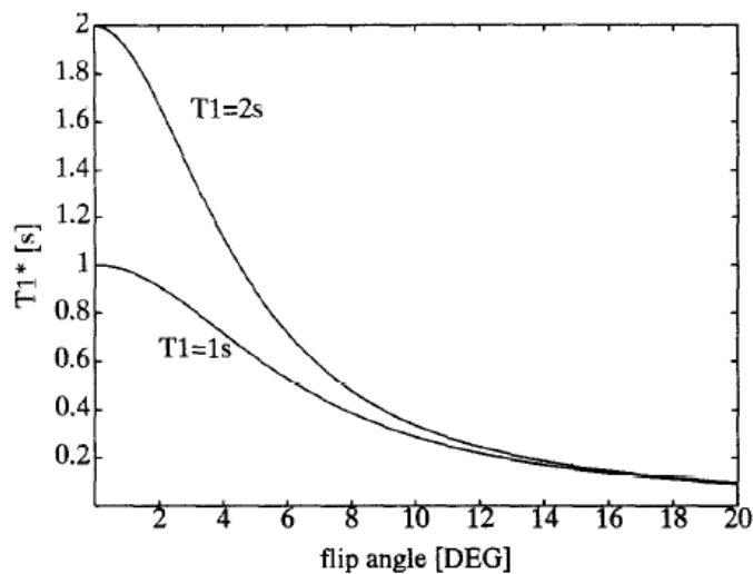
Figure 2.14. T_1^* dependence on the flip angle for two different relaxation times.
