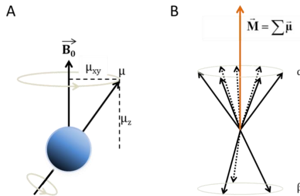
Figure 1.2. The net magnetization \mathbf{M} vector in an external magnetic field.
