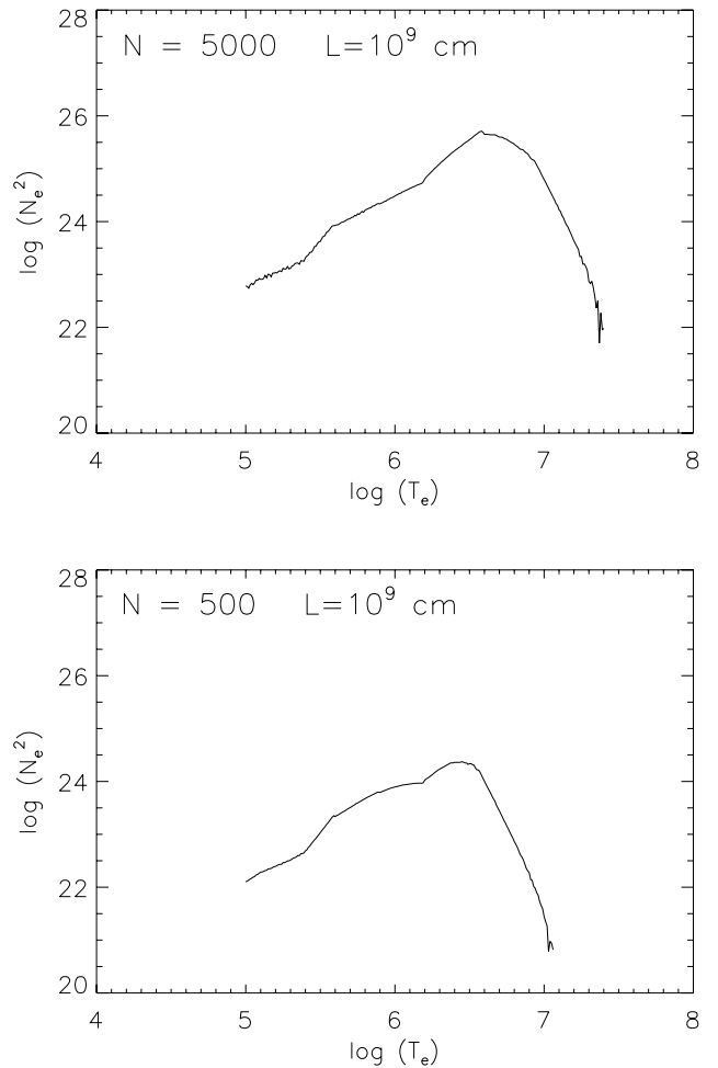
FIG. 4.—Logarithm of N_e^2 as a function of the logarithm of temperature, obtained with the parameters A_h = 8 \times 10^{13} \text{ cm}^2 , N = 5000 ( top ) and A_h = 8 \times 10^{14} \text{ cm}^2 , N = 500 ( bottom ).
