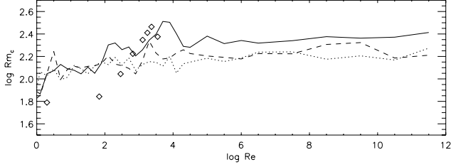
Fig. 2. Stability curves Rm_c(Re) for the local (plain line), weakly non-local (dashes), and strongly nonlocal (dots) models, and from Iskakov et al. (2007) (diamonds).
