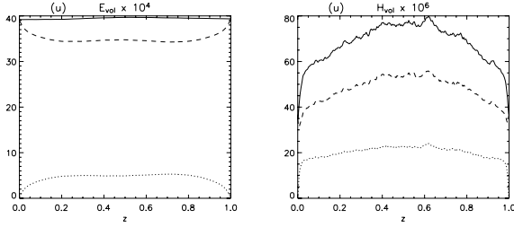
Fig. 2. Average profiles of the energy ( left ) and dissipation power ( right ) per unit volume, as a function of the position z along the loop, for run (u). The dotted lines are the kinetic energy or dissipation power, the dashed line the magnetic energy or dissipation power, and the plain line is the total.
