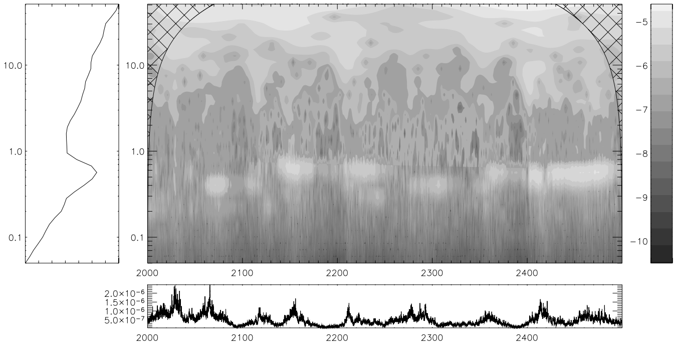
FIG. 14.—Center: Morlet wavelet timescale plane of the kinetic energy time series (logarithmic color scale). Oscillations of long but finite lifetime and of different frequencies can be seen at timescales (vertical axis) between 0.2 and 0.6. Left: Average wavelet spectrum. Bottom: Time series of total dissipation power. [See the electronic edition of the Journal for a color version of this figure.]
