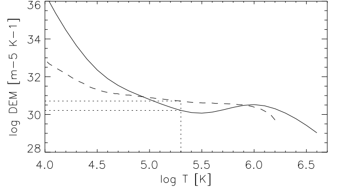
Fig. 4. Quiet Sun standard DEM from CHIANTI (plain line) and DEM computed from the Avrett & Loeser (2008) temperature and density profiles dashed lines. The dotted lines represent the DEMs for \log T = 5.3 , the maximum emission temperature of the S VI lines.
