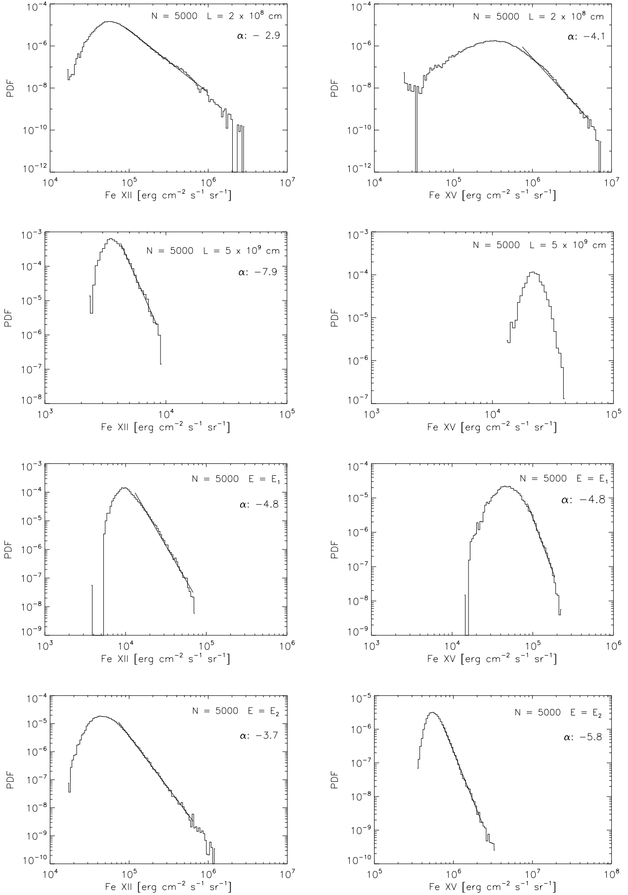
FIG. 6.—PDFs for Fe XII 195 Å ( left ) and Fe XV 284 Å ( right ). PDFs for different values of L ( top four panels ) and flare energy ( bottom four panels ). Here E_1 = 2.5 \times 10^{-4} ergs \text{cm}^{-3} \text{s}^{-1} and E_2 = 5 \times 10^{-3} ergs \text{cm}^{-3} \text{s}^{-1} .
