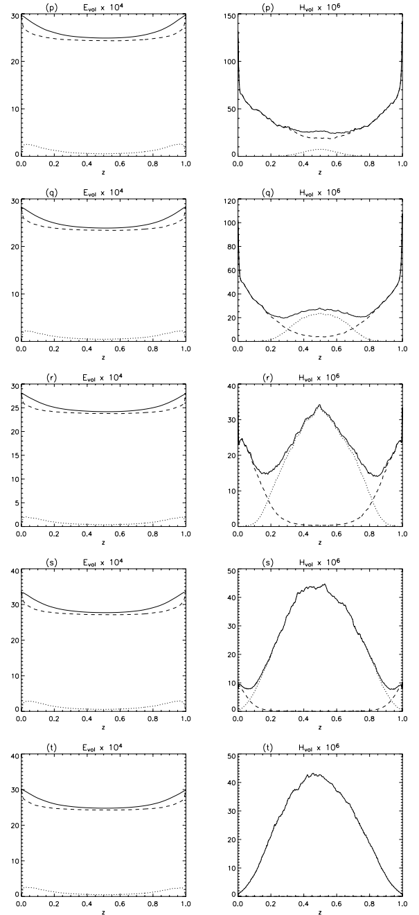
Fig. 8. Average profiles of the energy (left) and dissipation power (right) per unit volume, as a function of the position z along the loop, for runs (p), (q), (r), (s) and (t) (from top to bottom). The dotted lines are the kinetic energy or dissipation power, the dashed line the magnetic energy or dissipation power, and the plain line is the total (same as in Fig. 2).
