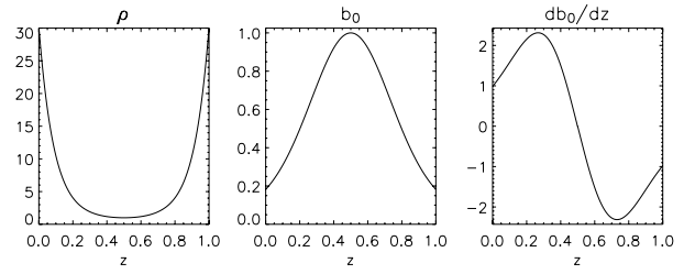
Fig. 4. Profiles of mass density \rho , Alfvén speed b_{\parallel} and gradient of Alfvén speed db_{\parallel}/dz for run (a), as a function of the position z along the loop.
