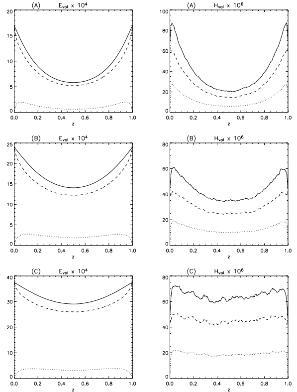
Fig. 6. Average profiles of the energy ( left ) and dissipation power ( right ) per unit volume, as a function of the position z along the loop, for runs (A), (B) and (C) ( from top to bottom ). The dotted lines are the kinetic energy or dissipation power, the dashed line the magnetic energy or dissipation power, and the plain line is the total (same as in Fig. 2).
