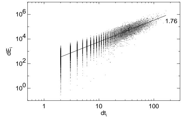
Fig. 8. Correlation between events duration and energy for parameters set (l).
