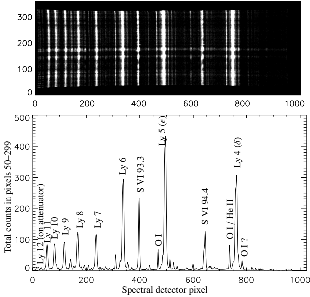
Fig. 1. Top: context spectrum (full detector A) taken on 4 May 1996 at 7 h 32 min UT. Bottom: total counts along slit between pixels 50 and 299. The S VI lines and the Lyman series of hydrogen (from Ly 4 to Ly 12) can be seen.
