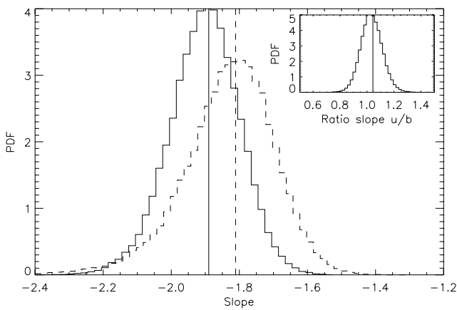
FIG. 8.— Distribution function of the slopes of the 1D perpendicular spectrum averaged along B_{\parallel} , for the kinetic ( solid line ) and magnetic ( dashed line ) fields. The median slopes are respectively -1.89 and -1.81 and are plotted as vertical lines. The distribution of the ratios between the slopes for kinetic and magnetic perpendicular spectra is shown in the inset, together with its median value of 1.044 .
