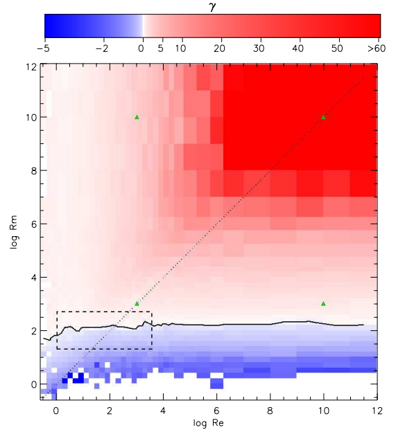
Fig. 1. Growth rate \gamma as a function of the Reynolds numbers Re and Rm (note that the color scale is different for positive and negative values of \gamma ), in the case of the weakly nonlocal Sabra model ( \alpha = -5/2 ). The stability curve, corresponding to the \gamma = 0 level line, is overplotted. The dashed rectangle corresponds to the range of parameters explored by the direct numerical simulations of Iskakov et al. (2007); the green triangles indicate the initial Reynolds numbers used in Fig. 4; the dotted line is where \mathrm{Pm} = 1 .
