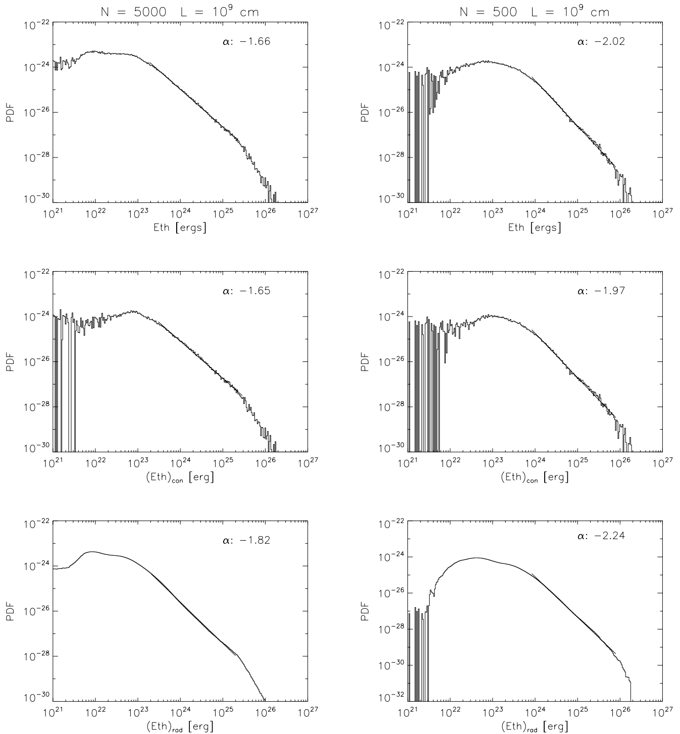
FIG. 3.—PDFs of total thermal energy ( top ); PDFs for the thermal energy during the conductive cooling phase ( middle ); and the PDF of the thermal energy during the radiative cooling phase ( bottom ). Left : A_h = 8 \times 10^{13} \text{ cm}^2 , N = 5000 . Right : A_h = 8 \times 10^{14} \text{ cm}^2 , N = 500 . For both cases L = 10^9 \text{ cm} . The index of the fitted power law is represented by \alpha .
