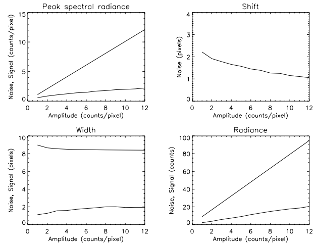
Fig. 3. Noise (lower curves) and signal (upper curves, when relevant) in each pixel as a function of the amplitude of the Gaussian profile used for the Monte Carlo simulations, for peak spectral radiance, line shift, line width, and line radiance.
