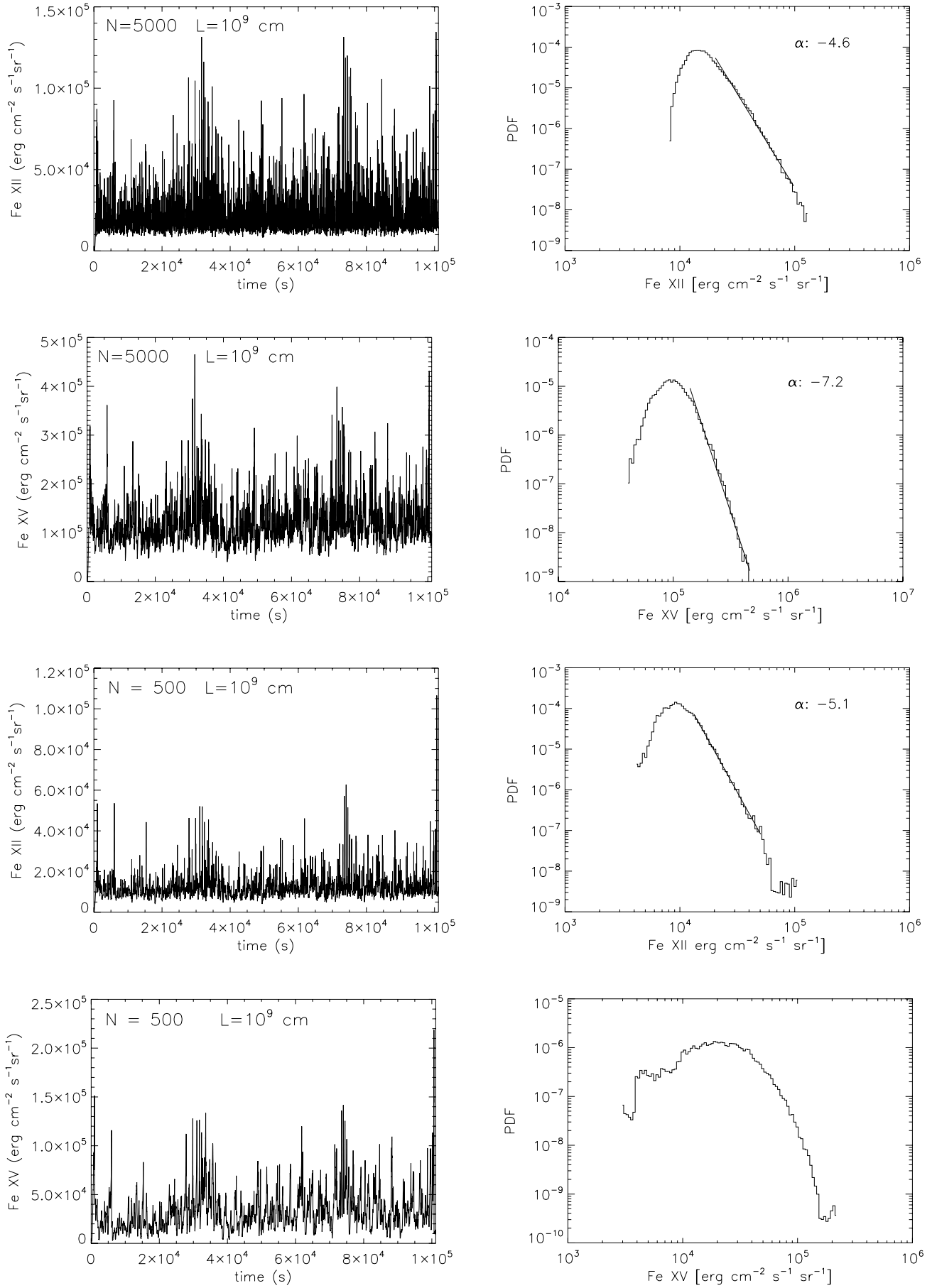
FIG. 5.—Total loop intensity as a function of time ( left ) for Fe XII 195 Å ( first and third panels ) and Fe XV 284 Å ( second and fourth panels ) and their PDFs ( right ). The parameters used for the simulation are the same as in Fig. 4.
