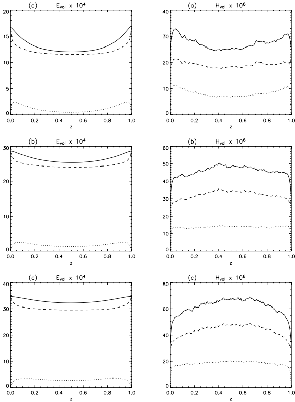
Fig. 5. Average profiles of the energy ( left ) and dissipation power ( right ) per unit volume, as a function of the position z along the loop, for runs (a), (b) and (c) ( from top to bottom ). The dotted lines are the kinetic energy or dissipation power, the dashed line the magnetic energy or dissipation power, and the plain line is the total (same as in Fig. 2).
