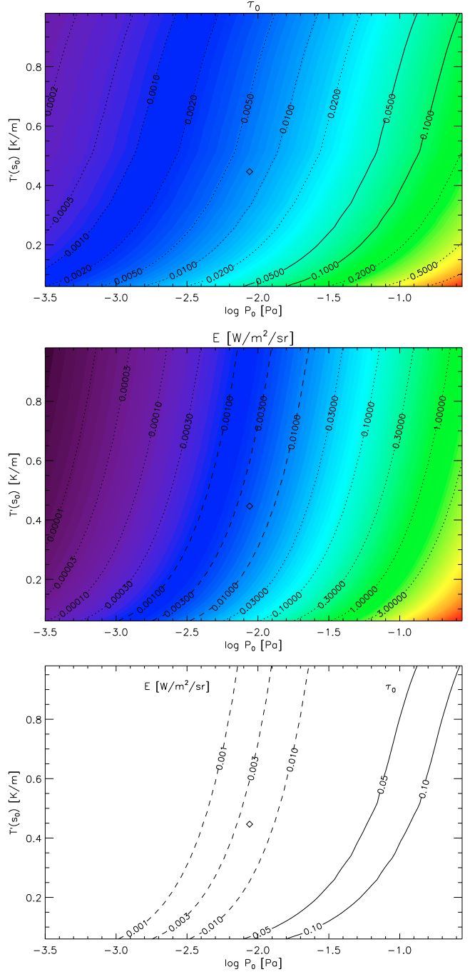
Fig. 6. S VI 93.3 nm opacity \tau_0 (top panel) and line radiance E (middle panel) as a function of model parameters P_0 and T'(s_0) . The level lines close to our actual observations are shown as plain lines for \tau_0 and as dashed lines for E . The bottom panel reproduces these level lines together in the same plot. The parameters (P_0, T'(s_0)) estimated from the Avrett & Loeser (2008) model at T = T_0 are shown with the diamond sign on each plot.
