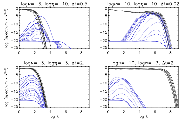
Fig. 4. Evolution of the spectra (compensated by k^{5/3} ) of kinetic energy (black) and magnetic energy (blue), for different sets of initial Reynolds numbers (Re, Rm) (shown as green triangles in Fig. 1), for the weakly nonlocal Sabra model. The spectra are averaged over ten independent runs and are plotted at time intervals shown as \Delta t in the plot titles. The different shades are a guide for understanding the direction of time (from black to gray and from dark to light blue, cycling every five spectra).
