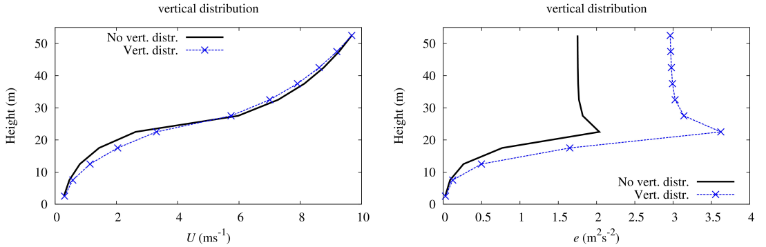
Fig. 8 Comparison of (a) the wind (in \text{m s}^{-1} ) and (b) e (in \text{m}^2 \text{s}^{-2} ) profiles computed with a vertical distribution of porosities (Vert. Distr) and with a regular array of cubes (No. vert. distr.). Altitude is in metres.
