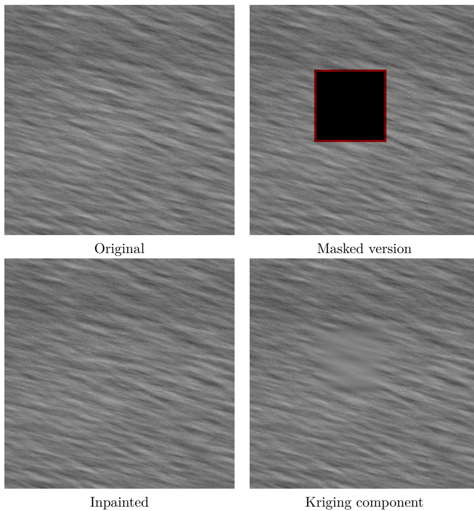
Figure 3.24: Conditional simulation. First row: original texture u (of size 512 \times 512 ) and the masked version with the conditioning points colored in red (the mask has size 151 \times 151 ). Second row: inpainted texture v (obtained in 18 seconds), and kriging component u^* .
