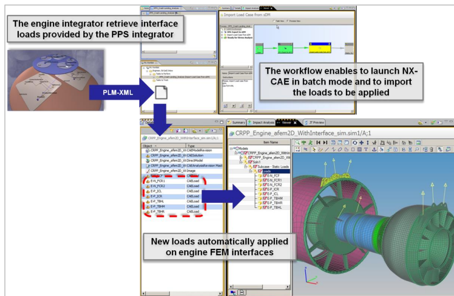
Figure 233: Engine interfaces loads automatically imported in TC4SIM and applied on engine FEM interfaces in NX-CAE
