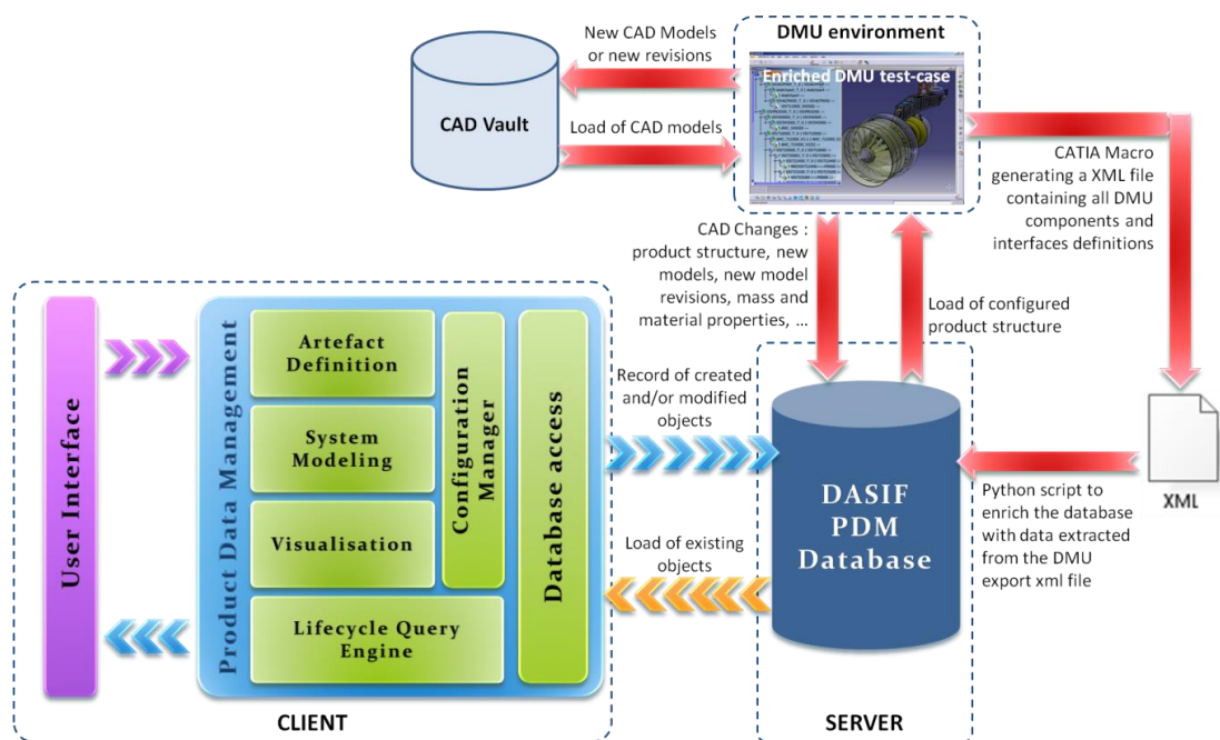
Figure 173: first DASIF prototype architecture
