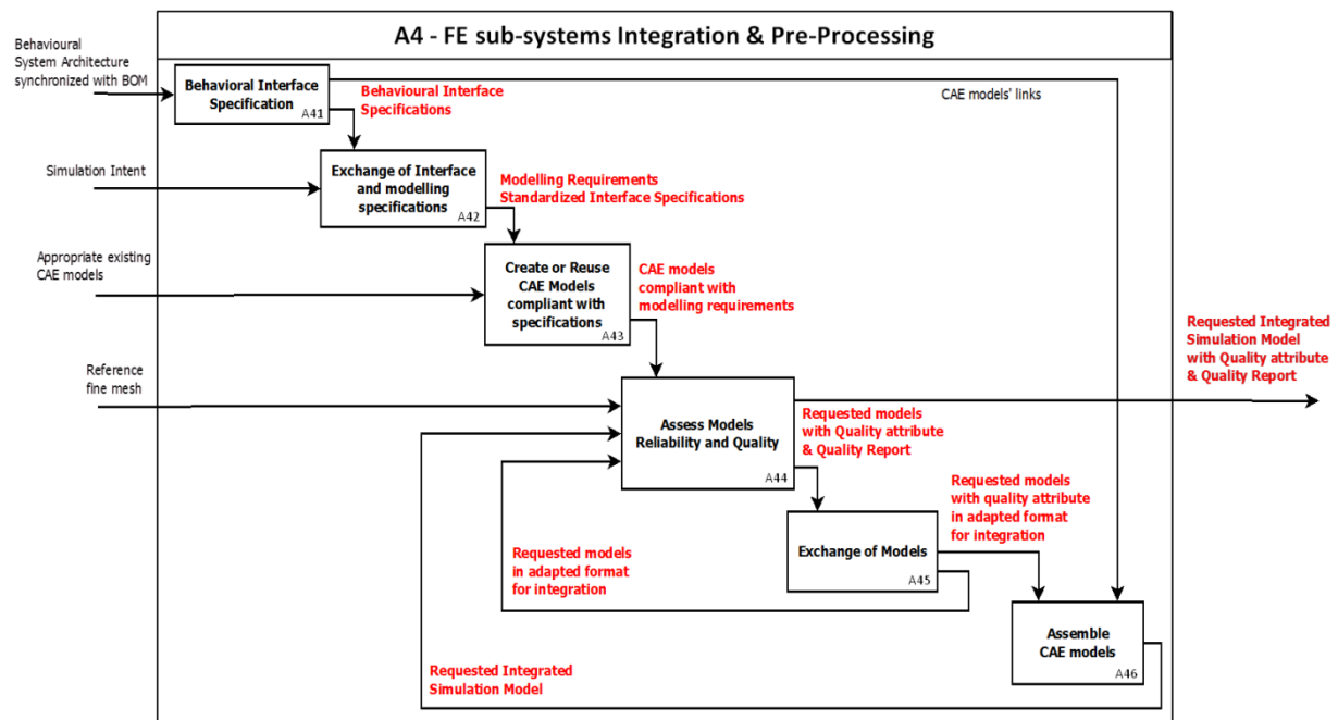
Figure 118: A4 SADT - SADT - FE Sub-systems Integration & Pre-Processing
