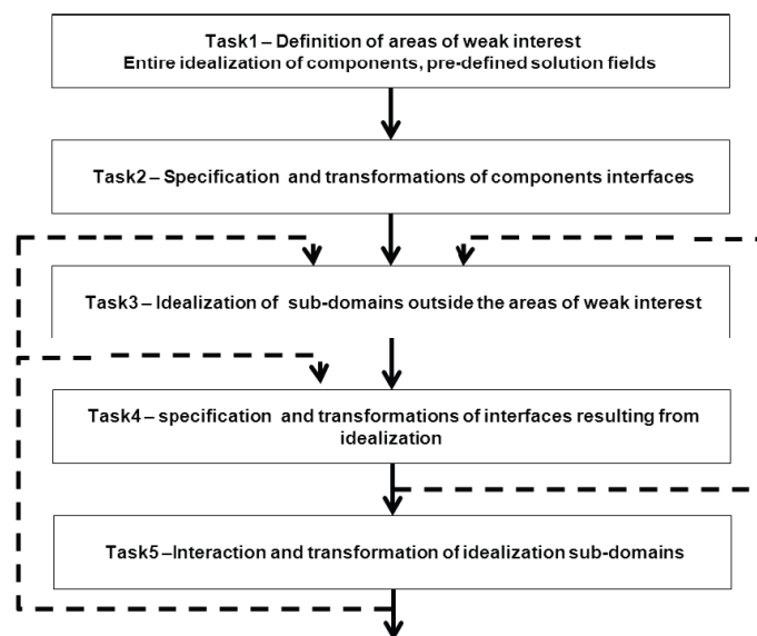
Figure 55: Structure of an assembly simulation preparation process [Boussuge et al., 2012]
