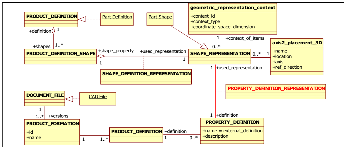
Figure 71a - Geometric model file related to part identification via property_definition_representation
