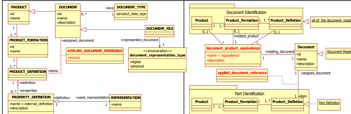
Figure 71b1 - Geometric model file related to part identification via applied_document_reference
