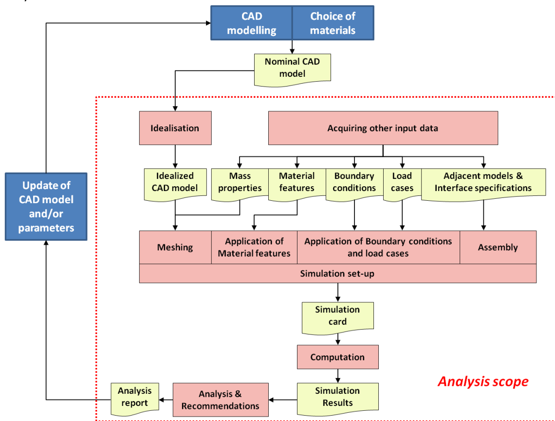
Figure 12: Design and Analysis data involved in a CAD-CAE loop process
