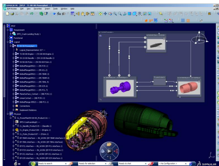
Figure 229: DDMU and corresponding BMU integrated in the RFLP environment
