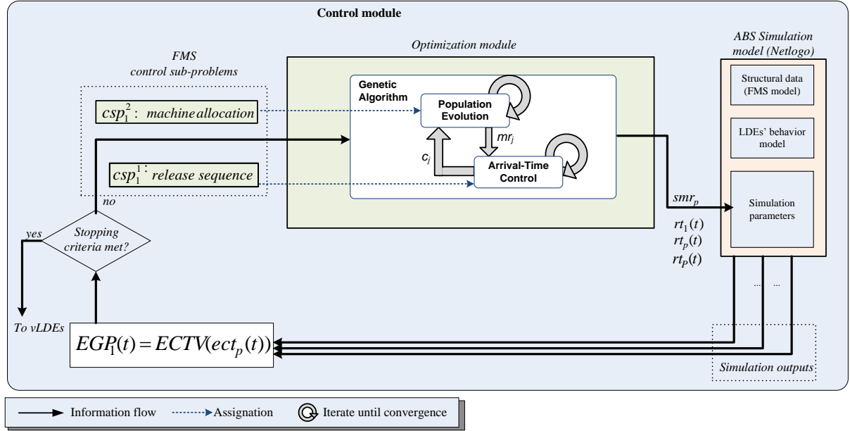
Figure V-16: The control module of pGDE_1 for problem instance C
