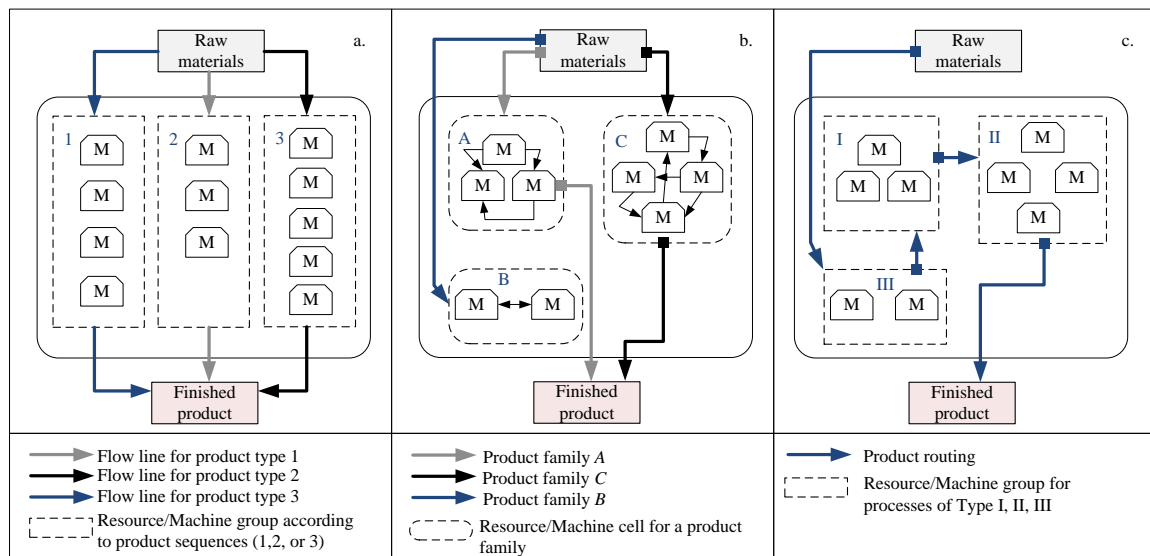
Figure A-2: a. Flow shop layout, b. Cellular system layout and c. Job shop layout
