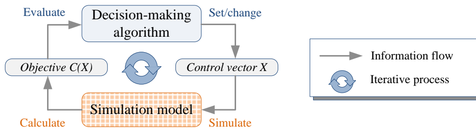
Figure II-2: Simulation-based optimization
