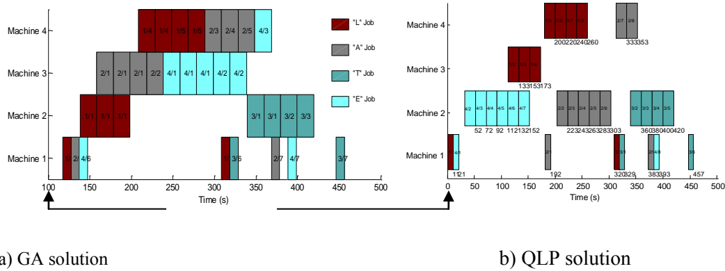
Figure H-4: Gantt charts for the scenario Sc0t01-02: 1 “LATE” order with a 388-second due date.
