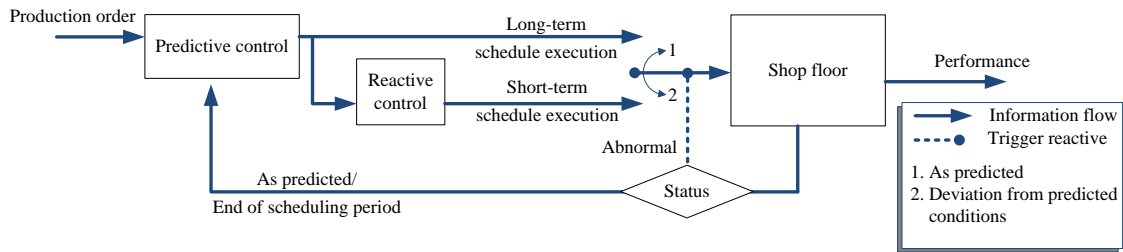
Figure D-2: Predictive-reactive control
