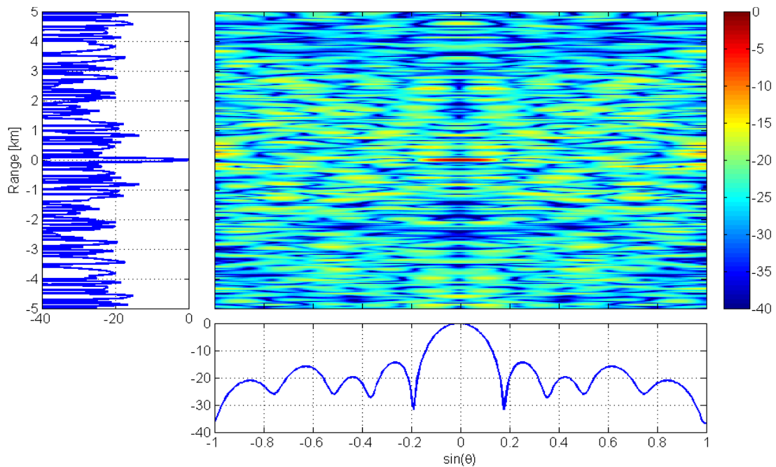
Figure B.3: Ambiguity functions (MF output) for a family of chaotic polyphase codes.
