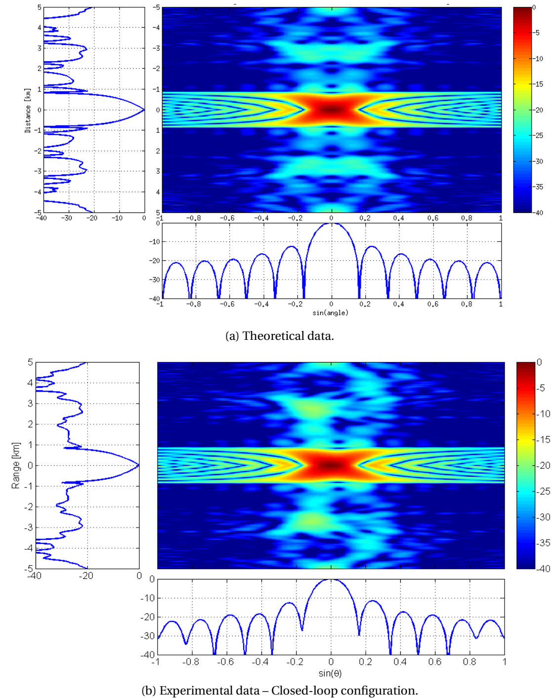
Figure B.4: Ambiguity functions (MF output) for a circulating Gold phase code.
