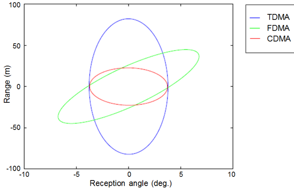
Figure 2.1: CLRB ellipses in range and reception angle for the TDMA, FDMA and CDMA waveforms.
