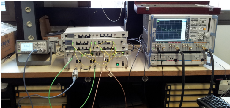
(a) Testbed: VNA on the right, delay line system on the left.
