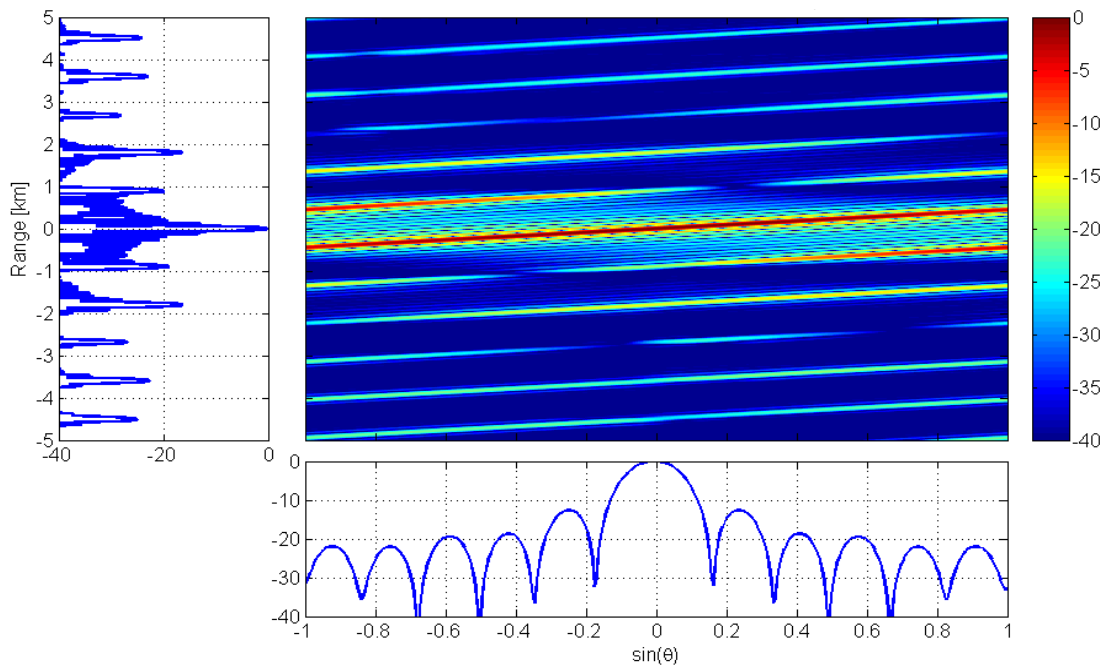
Figure B.8: Ambiguity functions (MF output) for a family of FDMA waveforms.
