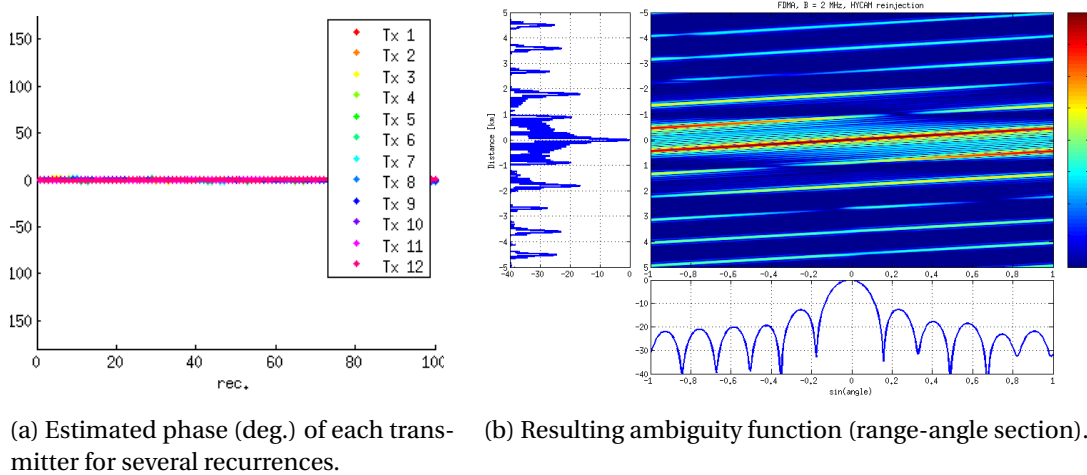
Figure 4.5: MIMO radar simulation with a family of 12 FDMA waveforms, random constant phase for each transmitter and Tx phase calibration after reception.
