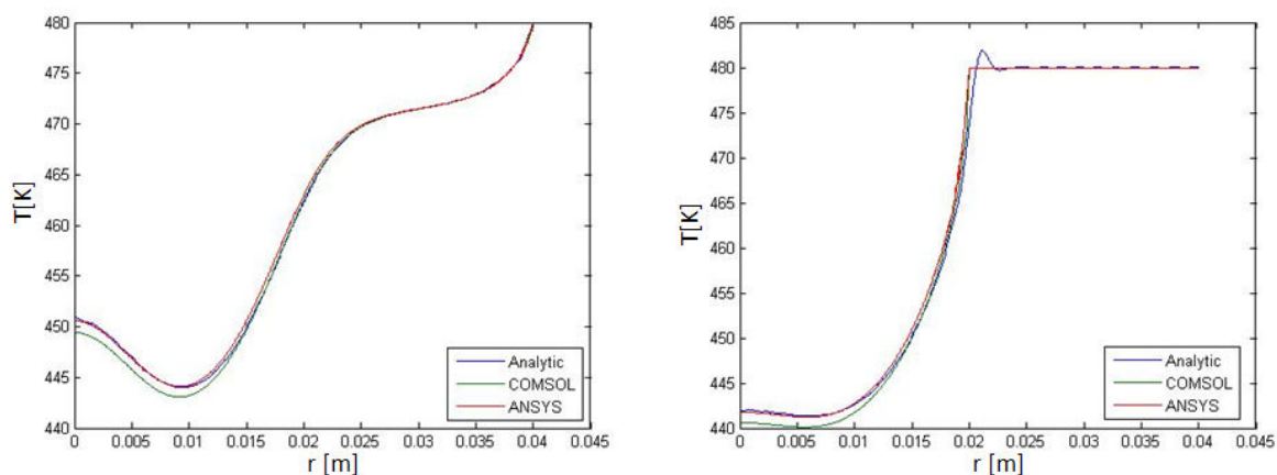
Figure 4.13: Temperature field validation for the TCS of section (4.5) - SIPHORE mirror geometry. Absorption coefficient 0.3ppm. Intracavity power 3MW. Environment temperature T_0=300 K, mirror edge temperature fixed at T_1=480 K, ring heater fixing the temperature of the mirror back surface between r = 0.02 m and r = 0.04 m at T_1=480 K. Left panel: mirror surface temperature inside the optical cavity. Right panel: mirror surface temperature outside the optical cavity.
