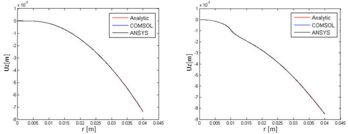
Figure 4.26: Displacement validation for the TCS of section (4.7) - SIPHORE mirror geometry. Absorption coefficient 0.3ppm. Intracavity power 3MW. Environment temperature T_0=300\text{K} . Mirror edge temperature fixed at T_1=500\text{K} . Ring heater fixing the temperature of the mirror back surface, between r = 0.01\text{m} and r = 0.04\text{m} , at T_1=500\text{K} . Central disk heater fixing the temperature of the mirror back surface at T_2=540\text{K} , between r = 0\text{m} and r = 0.01\text{m} . Left panel: mirror surface displacement inside the optical cavity. Right panel: mirror surface displacement outside the optical cavity.
