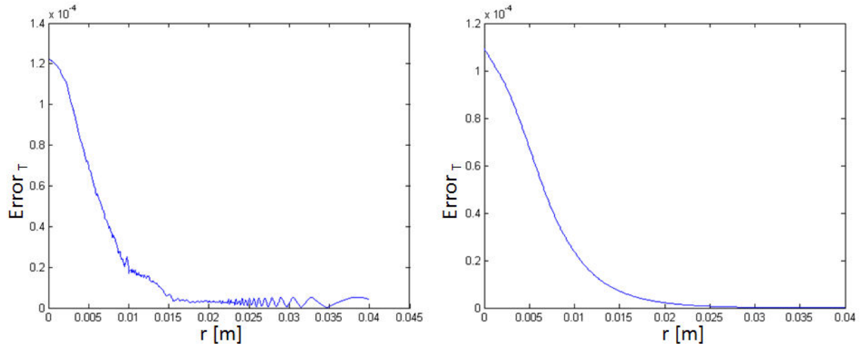
Figure 4.11: Percent error for the analytically calculated temperature field with respect to the numerically calculated one, for the TCS in section (4.4). Mirror front surface.
