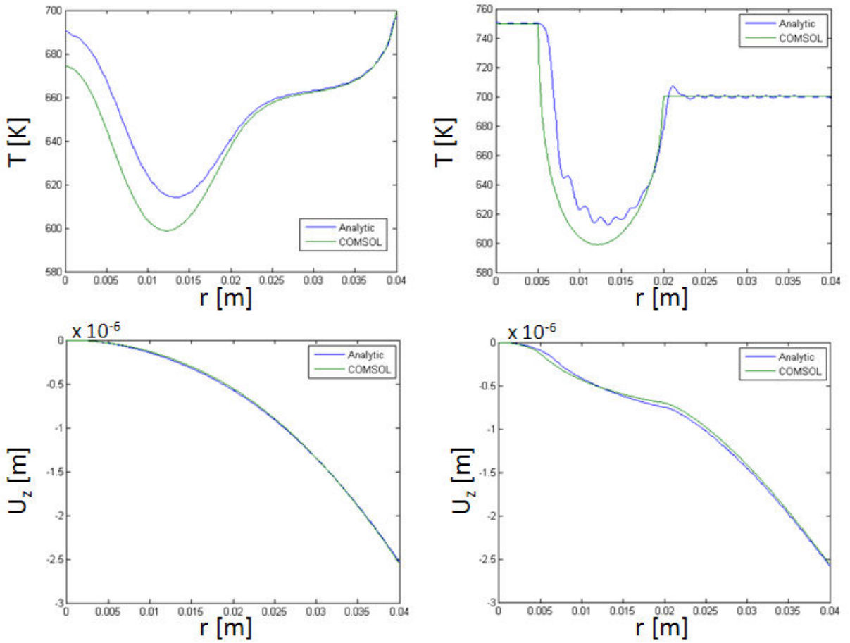
Figure 5.10: Mirror surface temperatures and distortions for a particular case of the TCS configurations in section (3.2.5) - Comparison between numerical and analytical simulations. Top panels: on the left, the mirror reflecting surface temperature is reported; on the right, the mirror rear side surface temperature is reported. The TCS parameter choice is described in section (5.3.4). Bottom panels: on the left, the displacement vector of the mirror reflection surface is reported; on the right, the displacement vector of the mirror rear side surface is reported. The TCS parameter choice is described in section (5.3.4)
