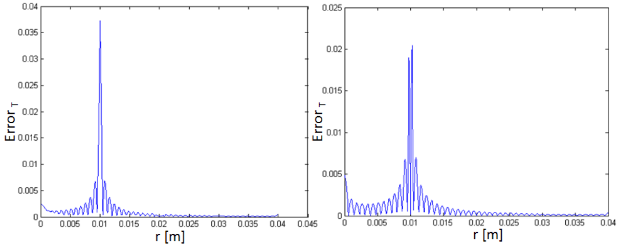
Figure 4.28: Percent error for the analytically calculated temperature field with respect to the numerically calculated one, for the TCS in section (4.7). Mirror rear surface.
