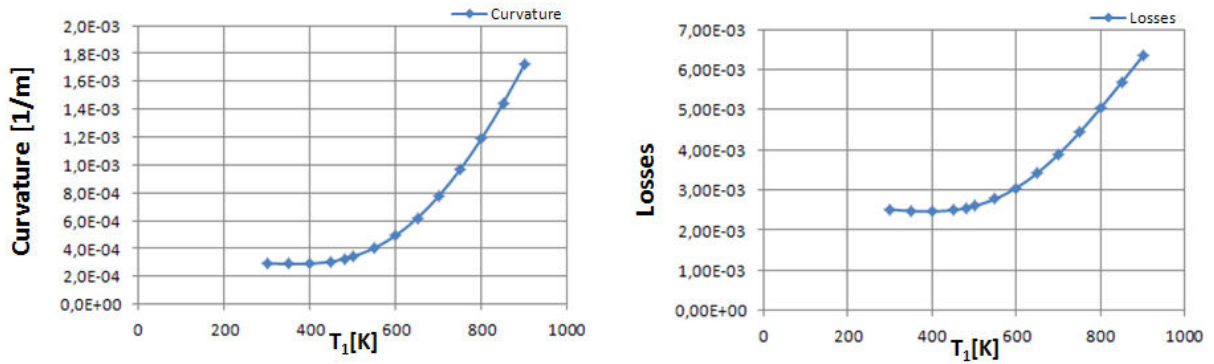
Figure 5.14: Loss and Curvature results for the TCS in section (5.3.6) - Left pannel: the mirror curvature resulting from the combination of the thermal effects and of the application of the considered TCS is showed, when the temperature, T_1 , fixed on the mirror is made to vary. Right pannel: the loss value for the mirror deformed by the combination of the thermal effects and of the application of the considered TCS is showed, when the temperature, T_1 , fixed on the mirror is made to vary.
