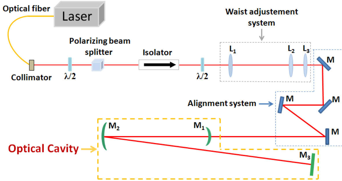
Figure 2.9: Scheme of the optical cavity - The complete scheme of the optical system before the resonator and of the optical cavity is showed. It is pointed out that the label \lambda/2 stands for half-wave plate; the index M indicates mirrors and L denotes lenses.
