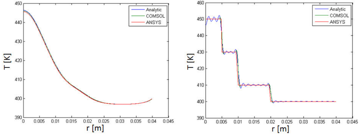
Figure 4.29: Temperature field validation for the TCS in section (4.8) - SIPHORE mirror geometry. Absorption coefficient 0.3ppm. Intracavity power 3MW. Environment temperature T_0=300\text{K} , edge mirror temperature fixed at T_1 = 400\text{K} ; one ring heater fixing the mirror temperature at T_1 = 400\text{K} , between r = 0.02\text{m} and r = 0.04\text{m} ; one ring heater fixing the mirror temperature at T_2 = 410\text{K} between r = 0.01\text{m} and r = 0.02\text{m} ; one ring heater fixing the mirror temperature at T_3 = 430\text{K} , between r = 0.005\text{m} and r = 0.01\text{m} ; a disk heater fixing the mirror temperature at T_4 = 450\text{K} , between r = 0\text{ m} and r = 0.005\text{m} . Left panel: mirror surface temperature inside the optical cavity. Right panel: mirror surface temperature outside the optical cavity.
