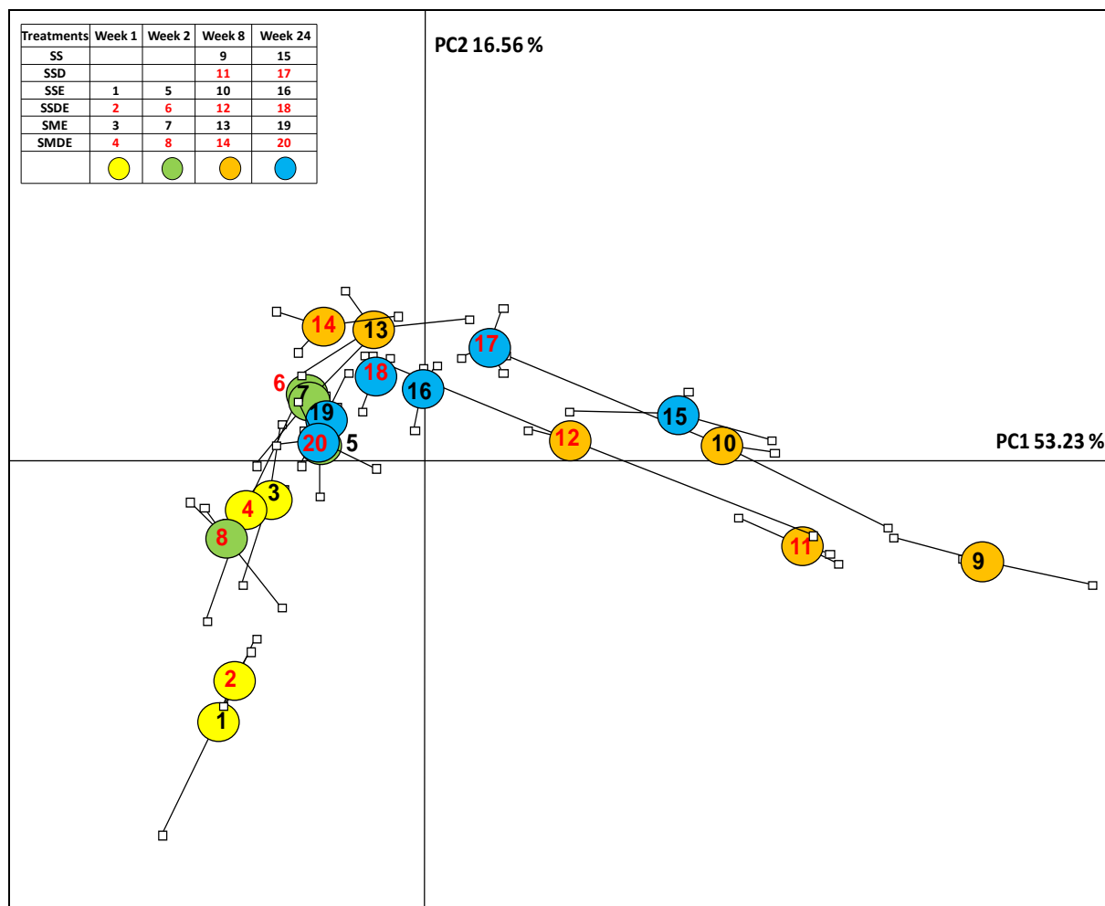
Fig. 4: Principal component analysis of T-RFLP data set in the two dimensional diagram from all the treatments for the fungal community structure. Each number represents the mean of 3 biological replicate for one treatment at a specific time period. For each biological replicate, 3 technical replicates were performed and provided non significantly different results. The red colour numbers represents the presence of DON. SS=Straw at the Surface, SSD= SS+DON, SSE= SS+Earthworms, SSDE= SSD+Earthworms, SME= Straw Mixed with the soil+Earthworms, SMDE=SMDE+DON.
