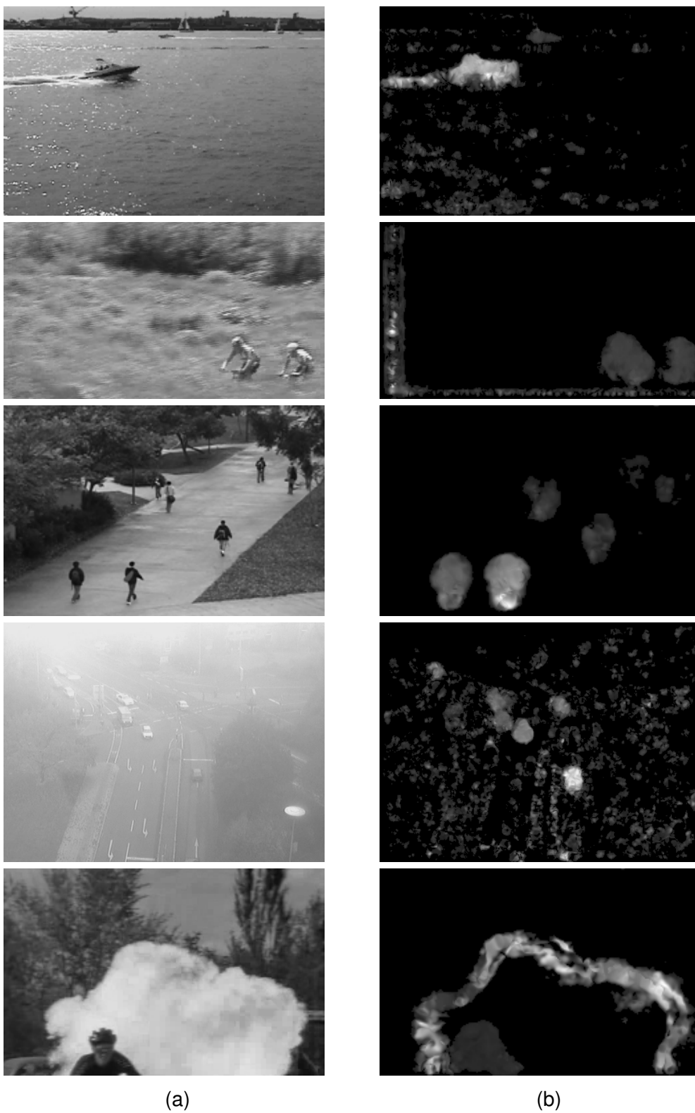
FIGURE 3.6 – Examples of dynamic saliency detection. (a) Original frame (b) Dynamic saliency
