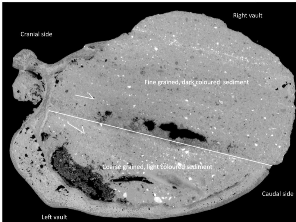
Figure 7.16. Cross-section (view from the top, see image of the top illustrating where the orthoslice is taken from) of the skull showing the sediments inside the vault (the white line indicates the limit between the two types of sediments, and the white arrows indicate the inclination of the sedimentary laminae) (images: courtesy of K. Carlson, modified).
