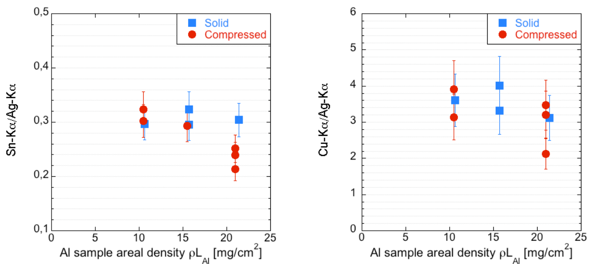
Figure 4.15: Evolution of the \text{Sn-K}_\alpha/\text{Ag-K}_\alpha (left) and \text{Cu-K}_\alpha/\text{Ag-K}_\alpha ratios as a function of the aluminum propagation layer areal density.
