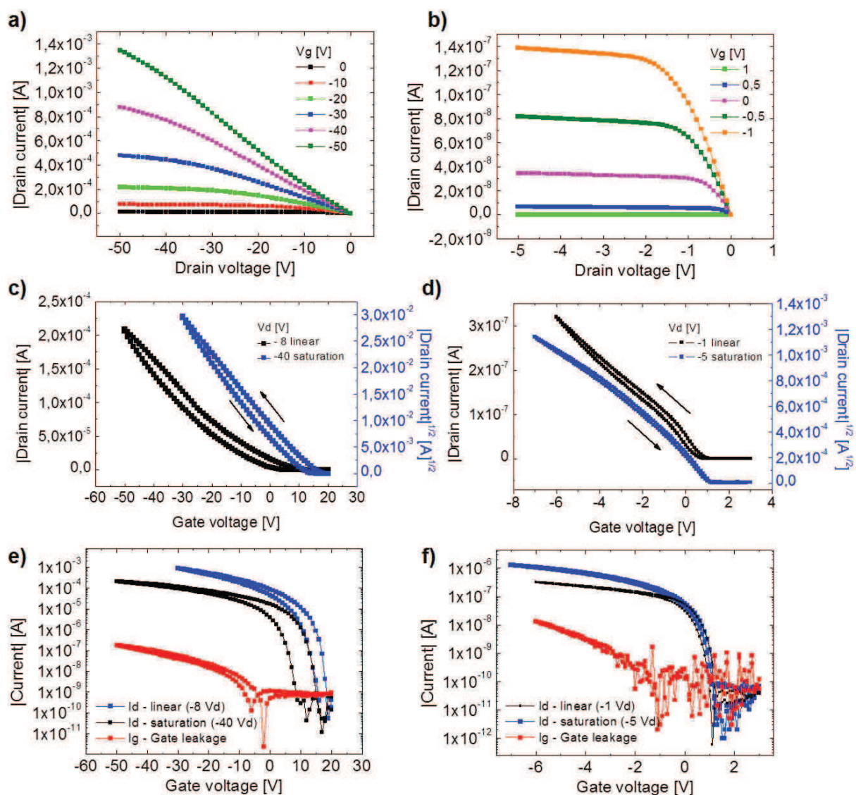
Figure 8.5: Current voltage characteristics of 3,5 \mu\text{m} channel length transistors on \text{SiO}_2 a), c), e) and \text{Si}_3\text{N}_4 b), d), f). Output characteristics: a) and b). Transfer characteristics in linear regime refer to the left y-axis. Square root of the drain current is plotted for the saturation regime, referring to the y-axis on the right side c) and d). Arrows indicate direction of hysteresis which is similar for all devices. e) and f) show semilogarithmic plot of transfer characteristics. Red plotted data shows leakage current from the gate for comparison.
