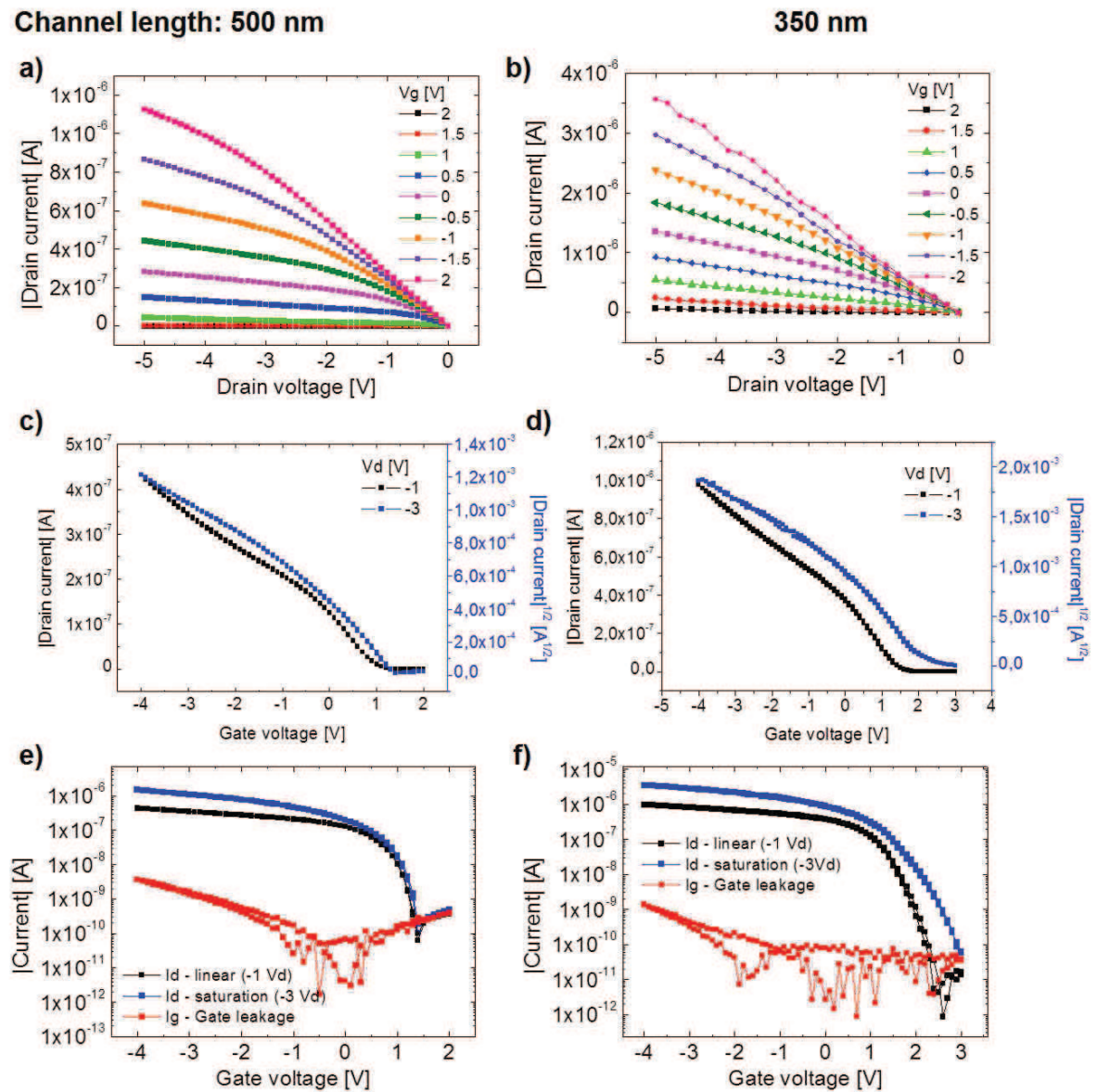
Figure 8.6: Current voltage characteristics of 500 and 350 nm channel length transistors with 31 nm width on 60 nm thick \text{Si}_x\text{N}_y . Output characteristics: a) and b). Transfer characteristics in c) and d) at -1 V refer to the left y-axis. For -3 V the square root of the drain currents are plotted, referring to the y-axis on the right side. e) and f) show semilogarithmic plots of transfer characteristics. Red plotted data show leakage currents from the gate for comparison.
