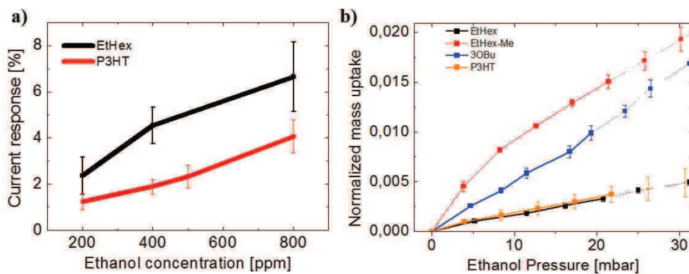
Figure 7.9: a) Comparison current response to ethanol for EtHex and P3HT devices. b) Normalized mass uptake.
