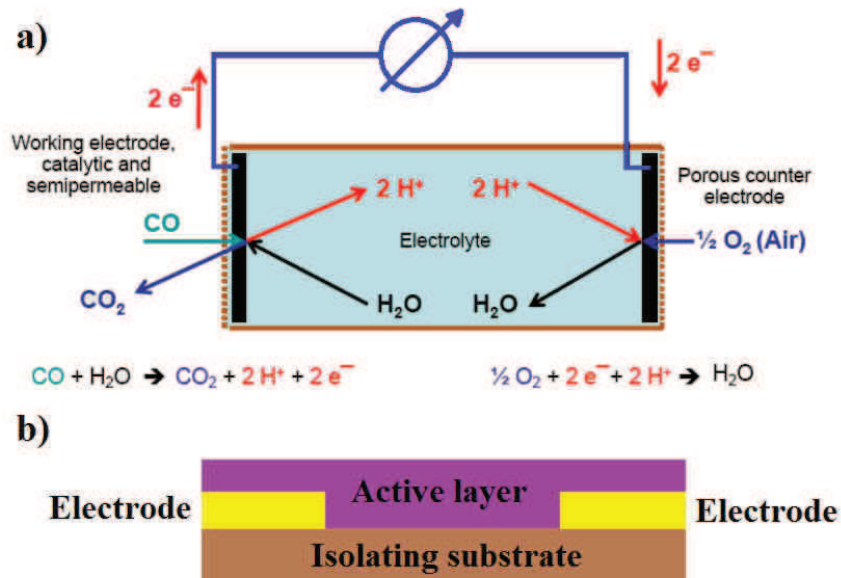
Figure 2.7: a) Schematic diagram of an electrolytic cell (adapted from [112]). b) Side view of chemiresistor.
