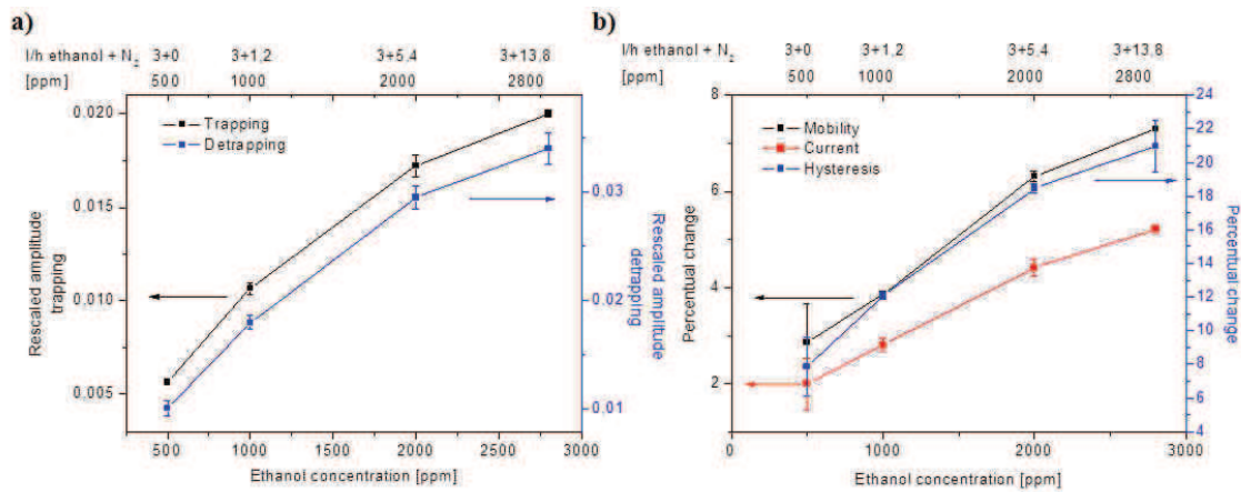
Figure 6.17: a) Response of rescaled transient current amplitude to ethanol exposure. b) Response of transfer characteristics for the same device. Outliers in b) at 500 ppm are perhaps due to incorrect ethanol concentration.
