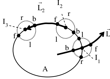
Figure II.5 Local characteristics of the intersections of neighbouring discs
