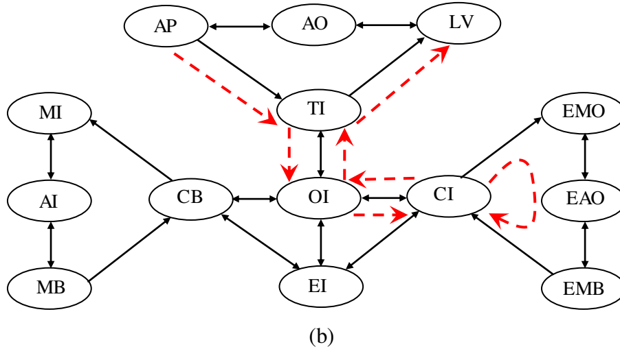
Figure IV.3 Continuous transitions of A moving over a smaller region B
