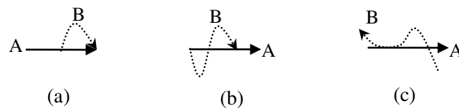
Figure II.13 Examples of configurations between directed lines
