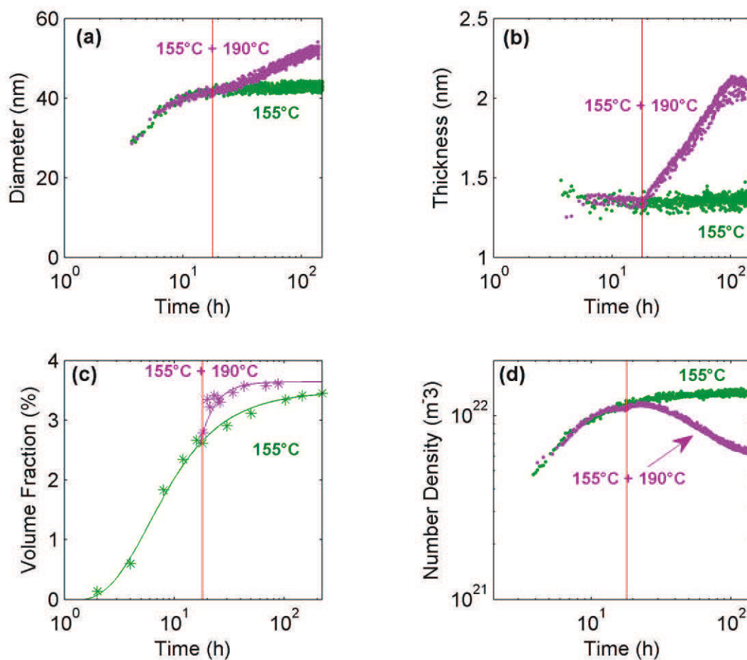
Figure 60: Evolution of the T_1 precipitate characteristics during ageing of the 2.5% pre-deformed sample at 155°C (green symbols) and duplex ageing 18h at 155°C followed by ageing at 190°C (purple symbols): (a) T_1 mean diameter and (b) thickness, (c) T_1 volume fraction evolution and (d) T_1 Number density.
