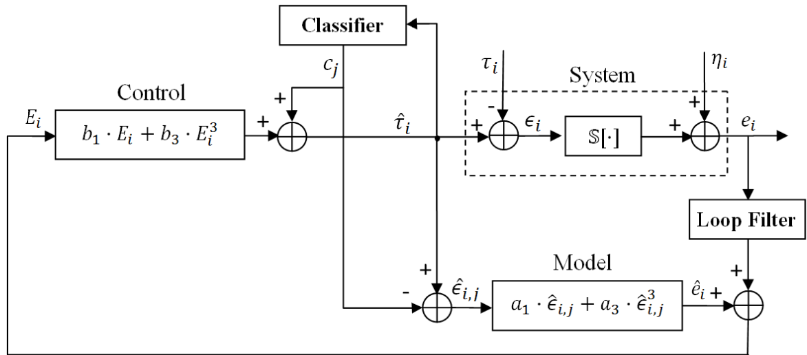
Figure 7.20 IMMC structure with loop filter
