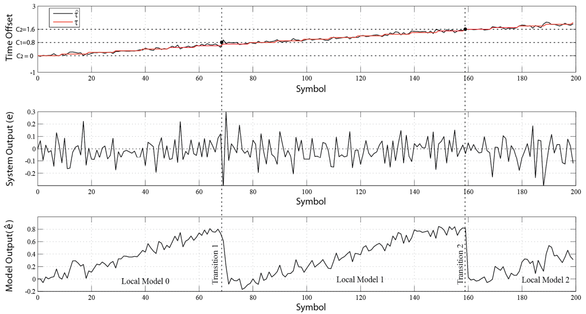
Figure 7.10 Evolution of the IMMC DLL tracking (SNR=3dB and \tau(n) increases in step form)
