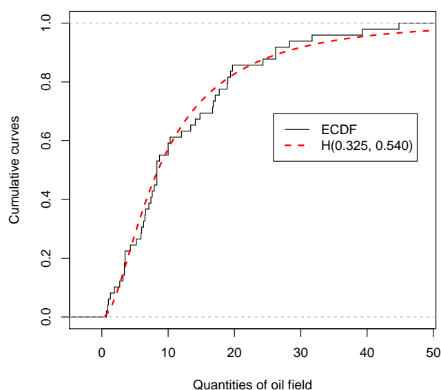
Figure 4.2: Empirical and H(0.325, 0.540) cumulative curves of quantities of oil field data.
