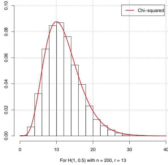
Figure 3.4: Simulated distribution of the \mathbf{Y}_n^2 statistic ( n = 200 , r = 13 ) under the null hypothesis H(a, b) recovering difference of parameters versus the chi-squared distribution with 12 degree of freedom.
