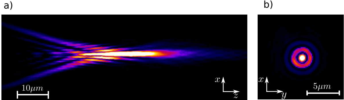
Figure 3.8: Measurements of 500µm diameter ball lens - (a) XZ-slice of focus spot generated by the microlens and (b) the focal plane (XY-slice), measurement performed with NA_{obj} = 0.45 .
