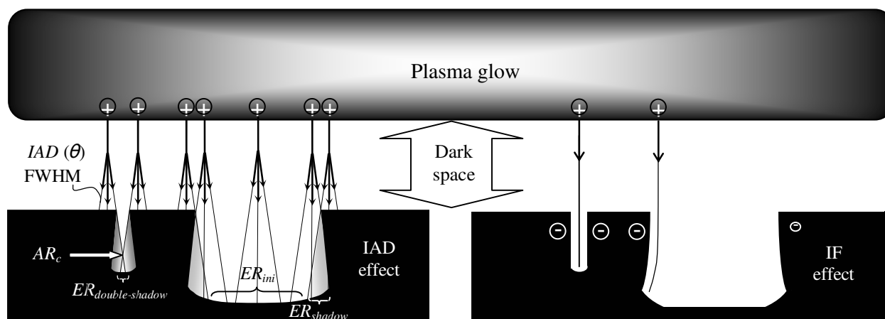
Figure 4.28: Scheme of plasma etching process - Geometry of etched structures by RIE depends on ions angular distribution (IAD), electrical interaction of ions and grounded etched surface (image force - IF). The different phenomena are usually highly dependent on the scale and aspect ratio of the etched structures [210].
