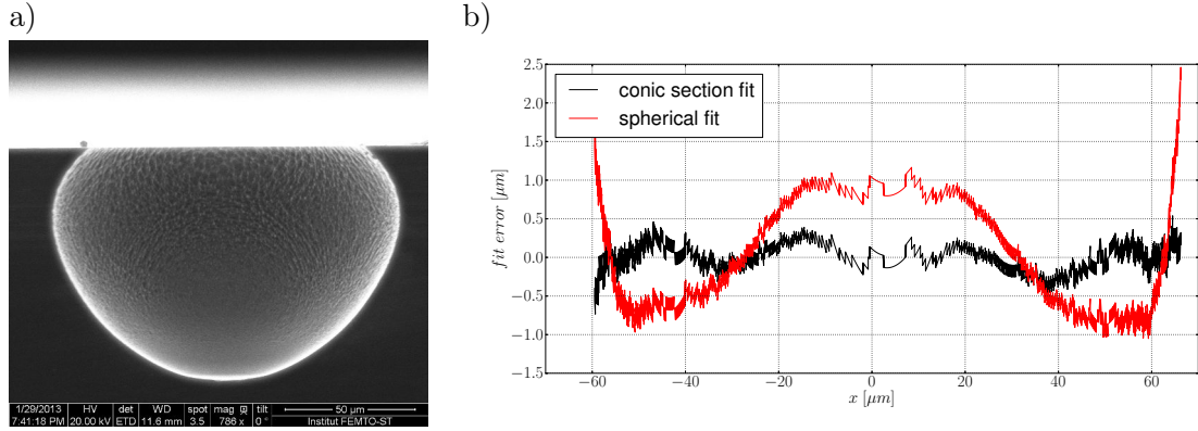
Figure 4.32: Negative conic constant profile - Generated ( p = 40mTorr, t = 1800s, d_{mask} = 30\mu m ) structure of aspect ratio slightly higher than a hemisphere, results in a profile that can be described as a conic section with negative conic constant. (a) SEM image of diced structure and (b) results of the fitting the profile to: conic section (black line) and to a sphere (red line), resulted fit parameters of the conic sections: k = -0.35 , ROC = 55.5\mu m RMS_{fit} = 0.18\mu m .
