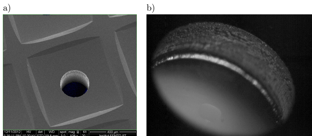
Figure 4.46: Realized mirrors for Schwarzschild micro-Objective - (a) SEM image of primary mirrors, (b) optical micrograph of secondary mirror within its silicon frame.
