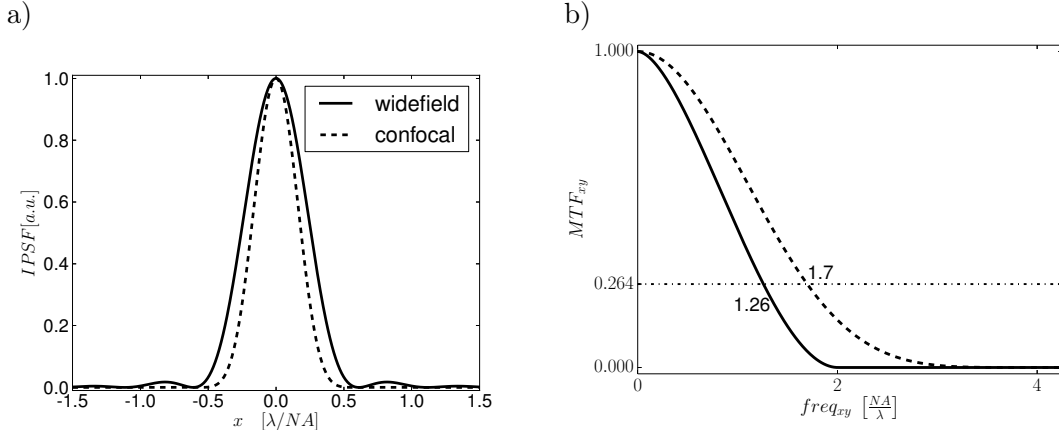
Figure 1.10: Classical wide-field vs confocal imaging system - Lateral resolution comparison via (a) IPSPF and (b) MTF, of confocal microscope (dashed line) and wide field system (solid line). It is visible that confocal system has higher resolution since MTF reaches higher spatial frequencies than classical system.
