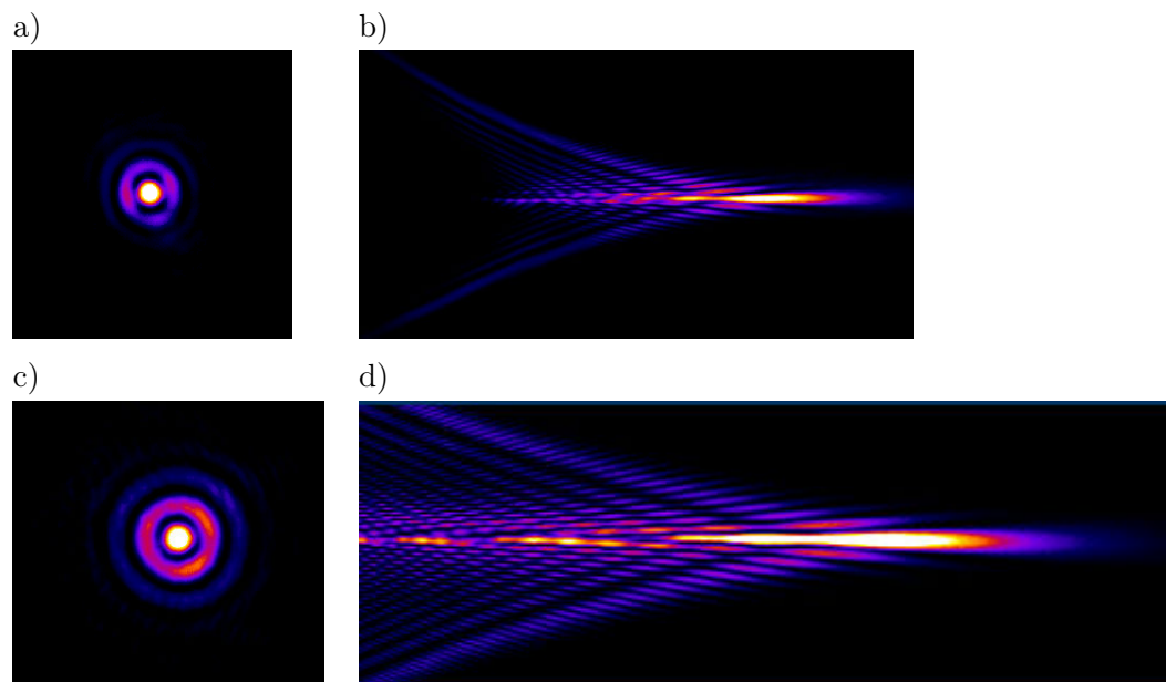
Figure 4.22: Optical measurements of micromolds: large mask window - Similar measurements to figure 4.21 in the case of two structures etched 40minutes through masks of diameters 110\mu\text{m} (a),(b) and 350\mu\text{m} (c),(d). Focus dimensions are summarized in table 4.2.
