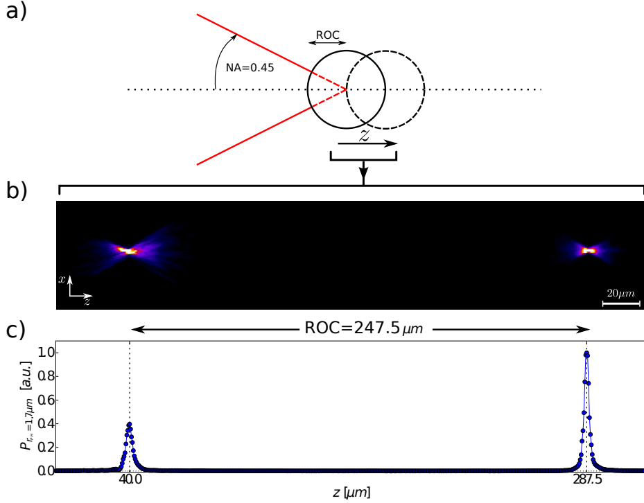
Figure 3.15: ROC measurement of 500 μm diameter ball lens - a) scheme of measuring configuration, b) slice (XZ) of measured intensity along all scanned distance (320 μm) visible two focal spots correspond to confocal (left) and cat's eye (right) positions, c) plot of power passing through virtual pinhole ( r = 1.7 \mu m ) located on the center of the beam, clearly visible two peaks allows accurate location of confocal and cat's eye position and determine the ROC value.
