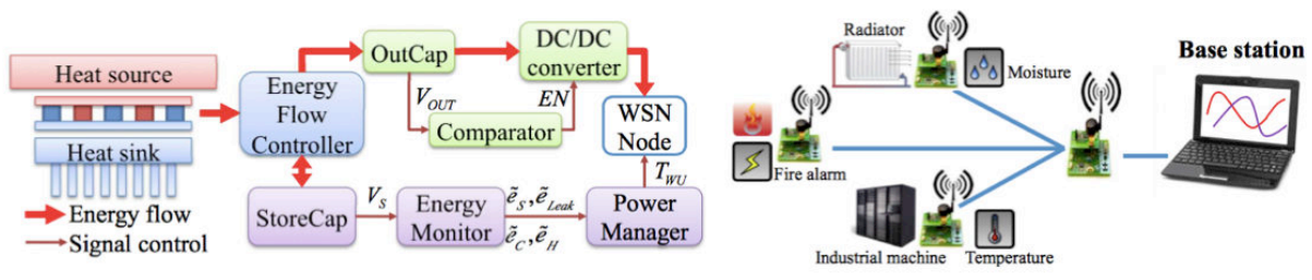
Figure 4.1: Generic architecture of the thermal-powered WSN node [1]
