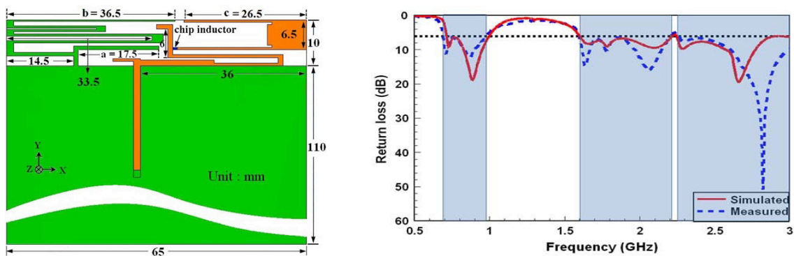
Figure 3.3: Coupled-fed and directed-fed monopole for mobile handset application [4].
