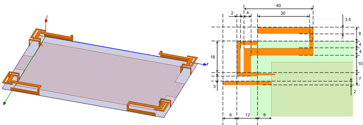
Figure 3.18: SPECTRA antenna geometry.
